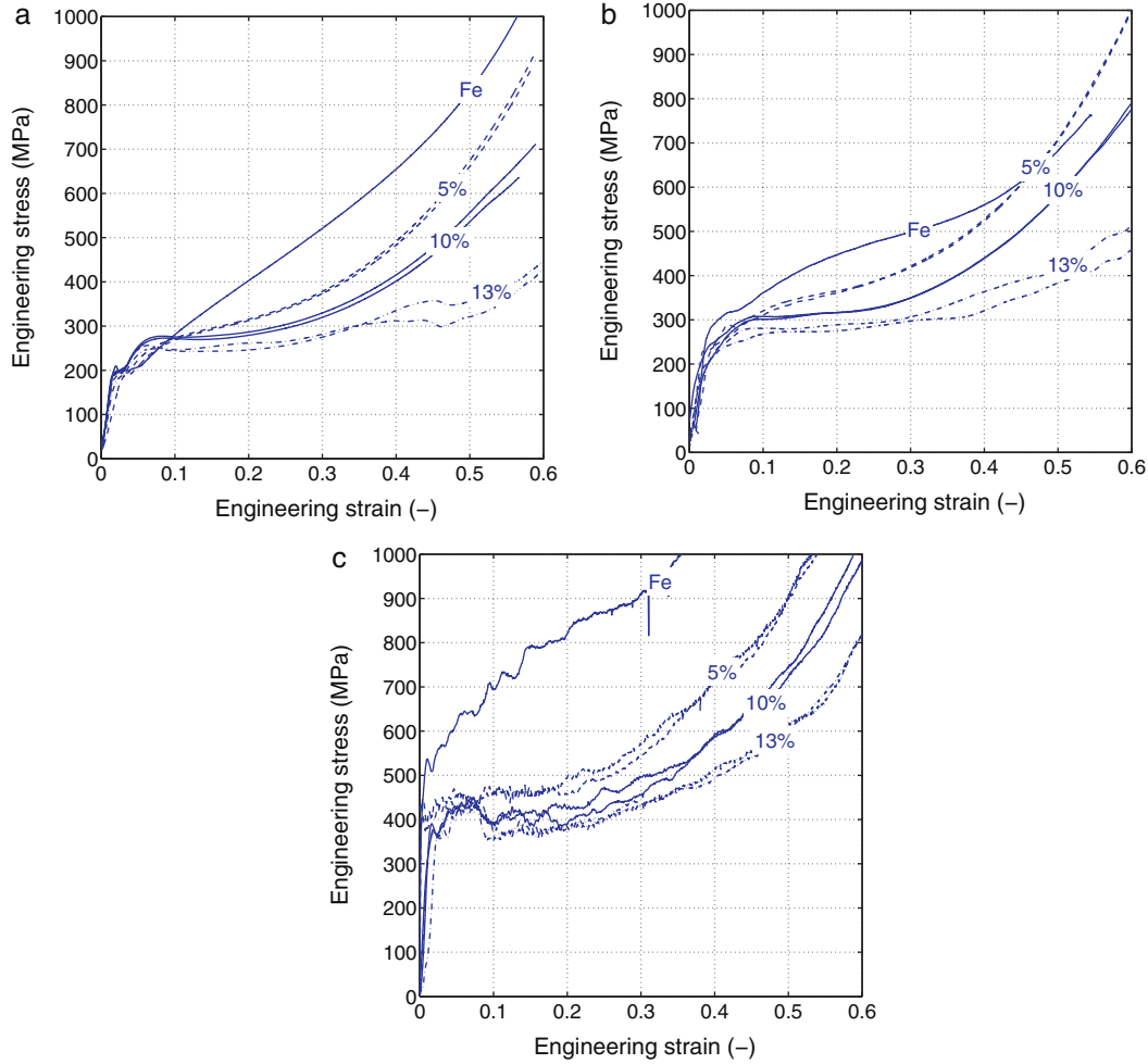
Fig. 5. Stress-strain characteristics for the iM30K syntactic foams: (a) quasi-static tests ( 10^{-2} \text{ s}^{-1} ); (b) medium strain-rate tests ( 10\text{--}20 \text{ s}^{-1} ); (c) high-speed SHPB tests ( 1000\text{--}2000 \text{ s}^{-1} ). For all test cases only two samples are reported for sake of clarity but repeatability was always very good.
