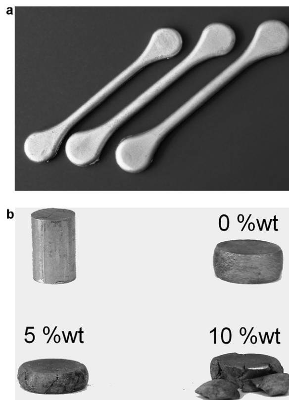
Fig. 2. Tensile specimens of syntactic foam (a), from the left: 0 wt%, 5 wt%, 10 wt%; cylindrical compression specimens before and after the test (b).
