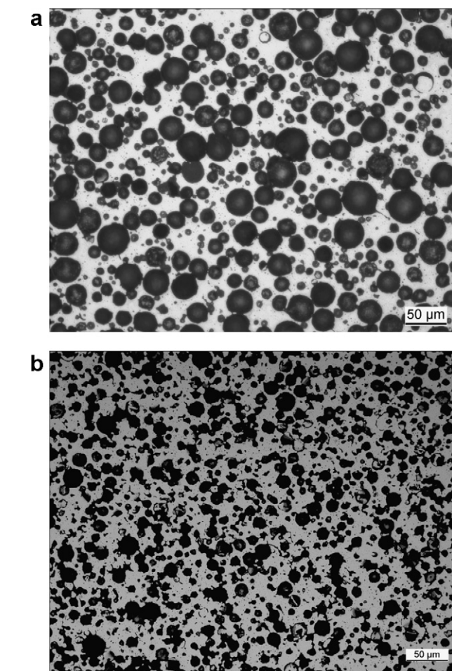
Fig. 1. Light microscopy of the metallographic sections of syntactic foams with different types of hollow spheres (10 wt%): (a) S60HS and (b) iM30K.
