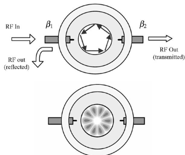
Figure 1.7 Basic principles of WGM
