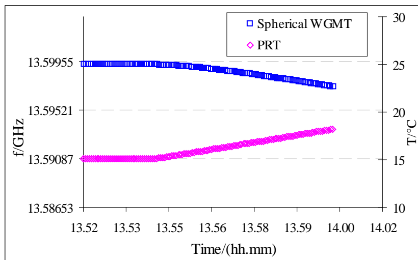
Figure 3.13 Zoom in of one part of the response comparison from Figure 3.12
