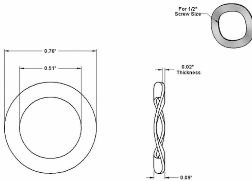
Figure B 10 Steel triple-wave washer
