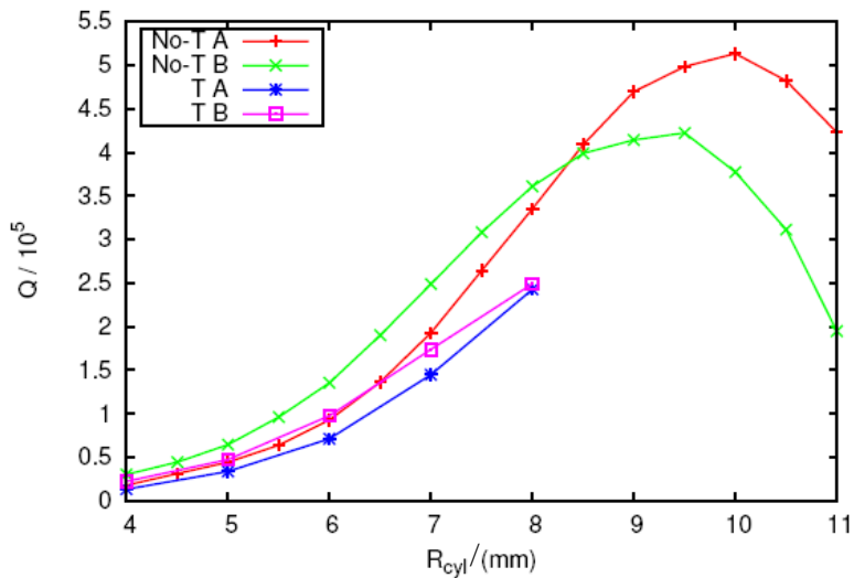
Figure 4.11 Q vs R_{cyl} for uniform-gap models with and without Teflon supports
