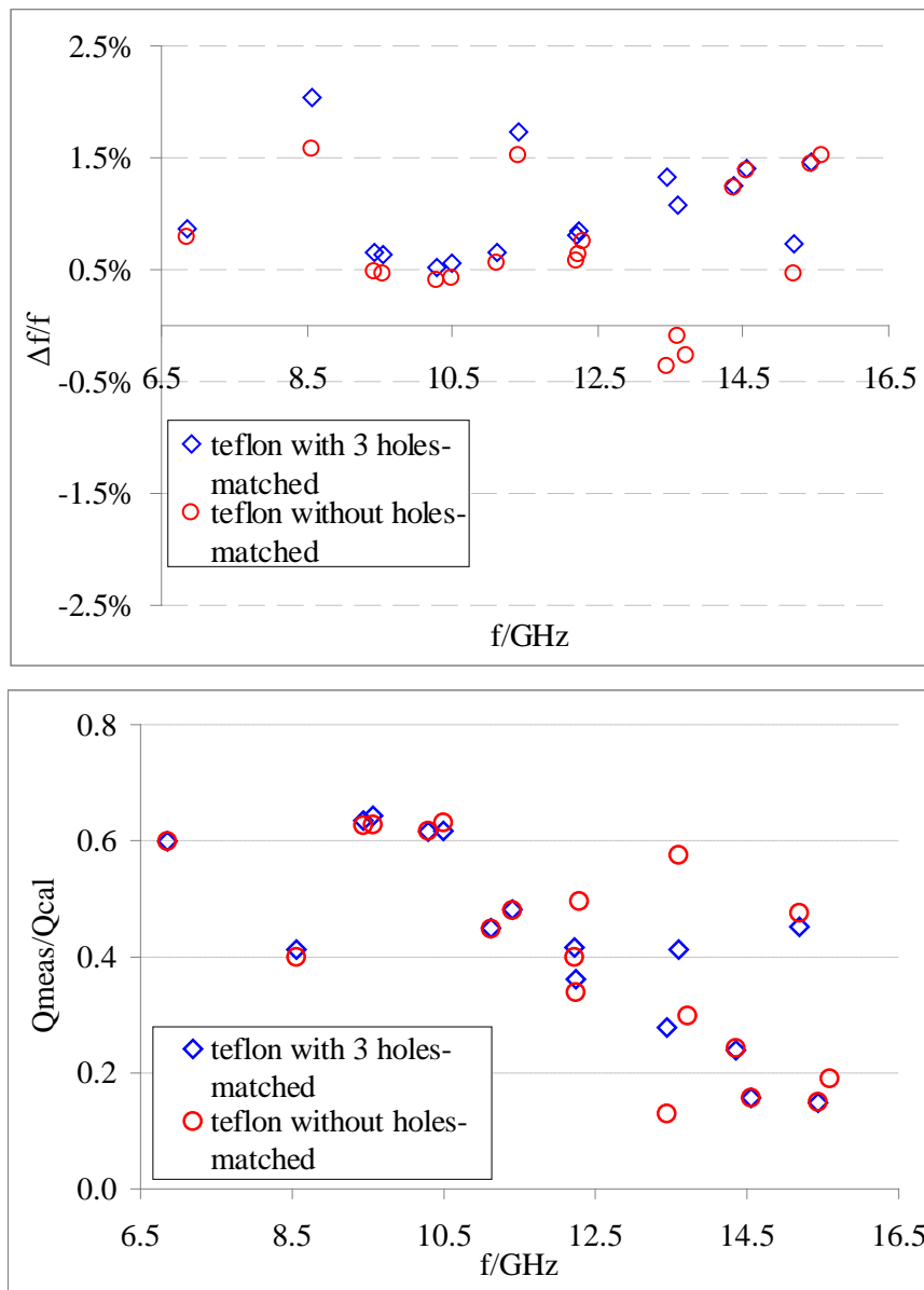
Figure 4.6 Frequencies and Qs comparisons between resonators with Teflon with and without holes
