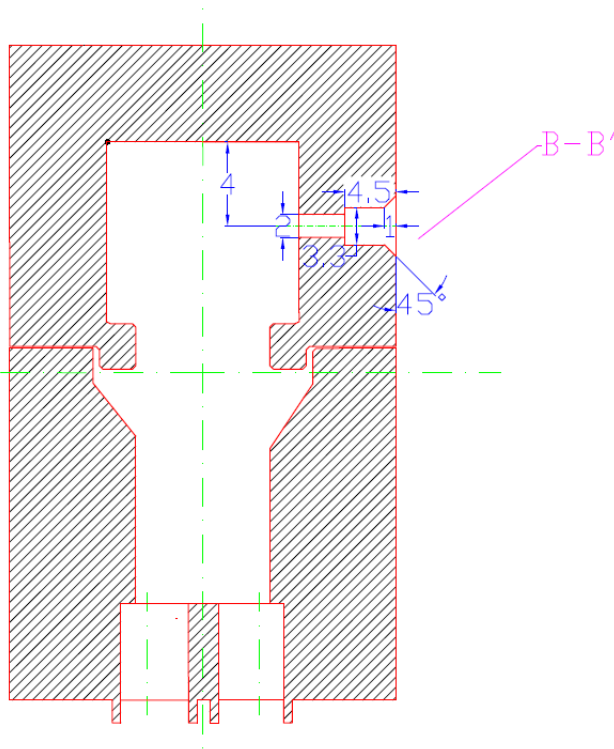
Figure B 6 Cut plane 2 of the cavity body front view (cut from the vacuum line)
