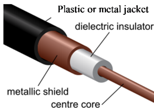
Figure 1.9 Coaxial cable cutaway
