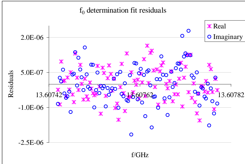
Figure 3.3 Fit residuals of the determination of f_0 for one mode
