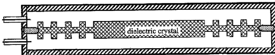
Figure 1.16 Bragg reflection mode thermometer
