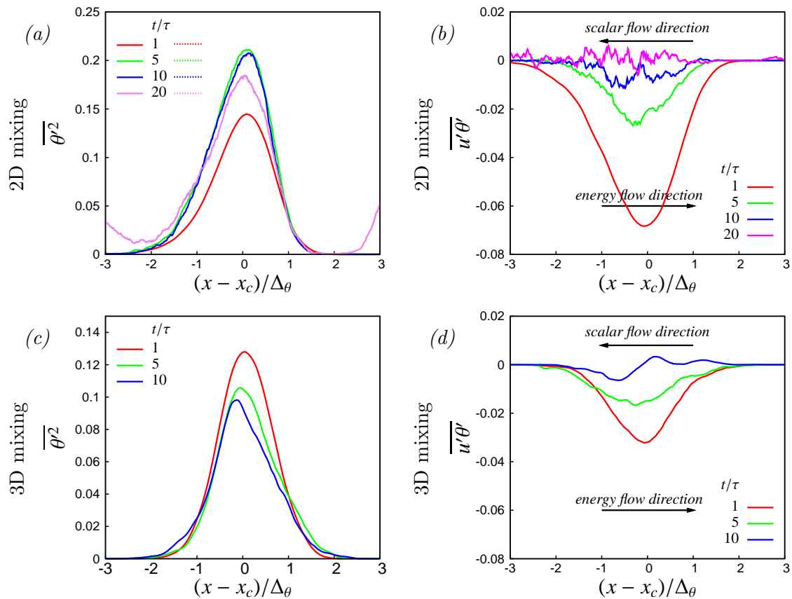
Figure 4. Left (a-c): Scalar variance in the simulations with initial energy ratio E_1/E_2 = 6.7 . Right (b-d): scalar flow \overline{u'\theta} in the simulations with initial energy ratio E_1/E_2 = 6.7 . The arrows indicate the scalar and energy flow directions.
