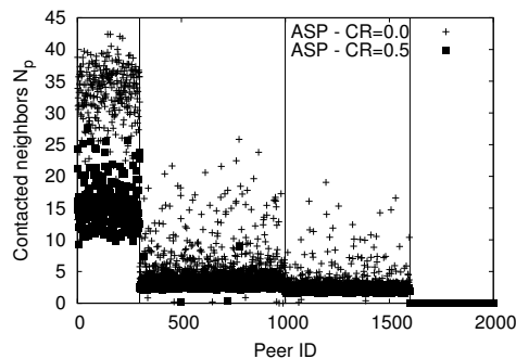
Figure 5. Average number of contacted neighbors N_p with ASP algorithms for all the peers, that are in decreasing order with their bandwidth at \rho = 0.9 .
