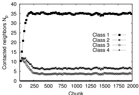
Figure 3. N_p evolution versus time with APS with CR = 0.0 and \rho = 0.9 .
