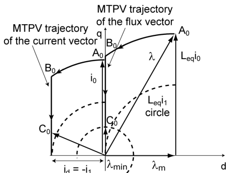
Figure 5. Vector diagram of the SPM motor at overload current i_o .
