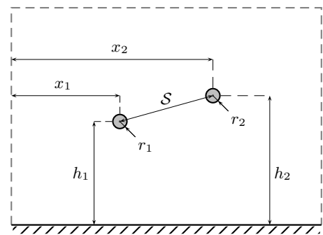
Fig. 4. Cross-section of the coupled lines setup used for validation. The heights above ground and separation of wires are selected as uncertain parameters.
