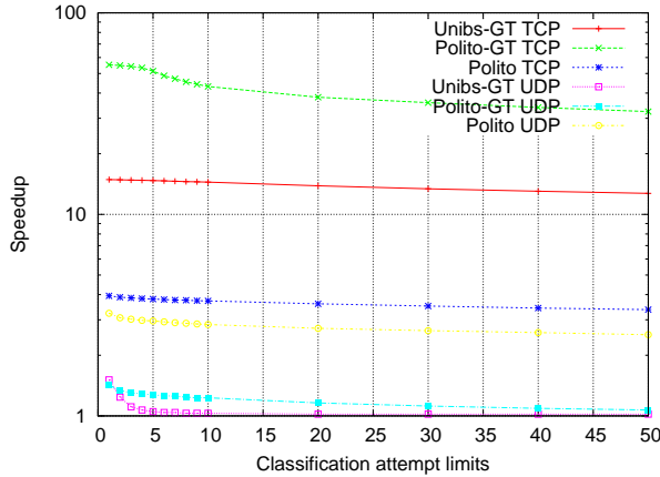
Fig. 8 Performance speedup at different classification attempt limits (Y scale is logarithmic).
