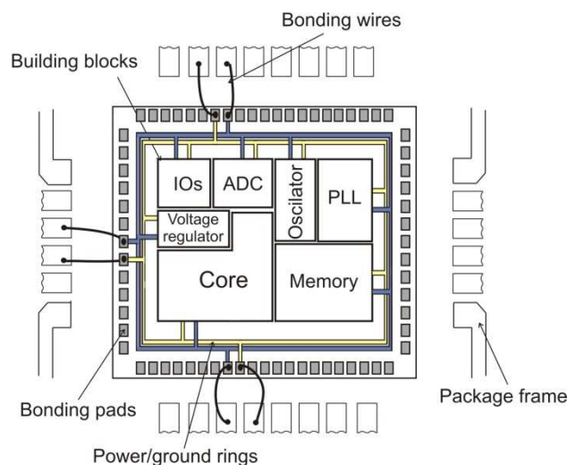
Fig. 1. Block diagram of a generic \mu C.
