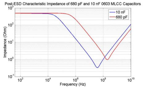
Fig. 10. Simulated Post-ESD Impedance Characteristics, R3 = 500 \Omega
