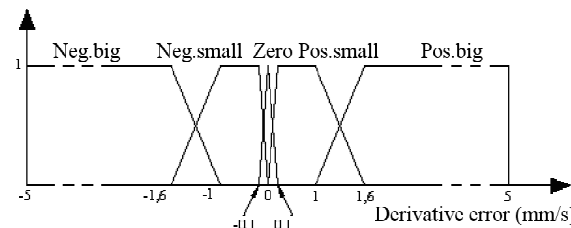
Fig. 7. Membership functions of the derivative error variable
