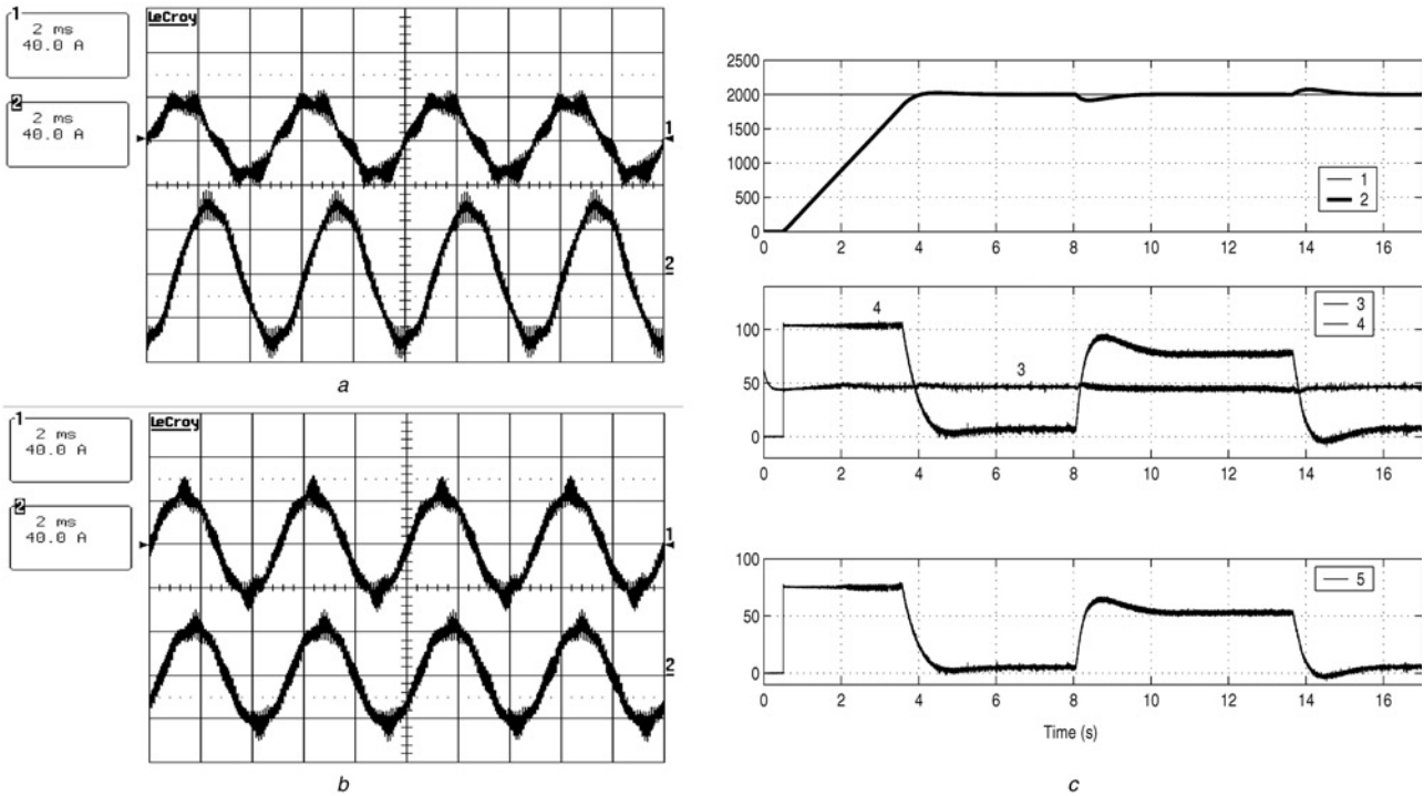
Fig. 22 Current control in the stationary reference frame
