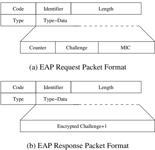
Figure 5 – Proposed EAP Packets format for Zero Authentication
