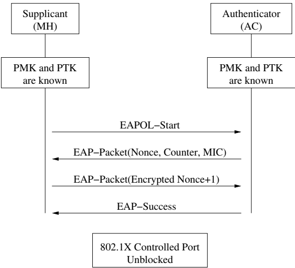
Figure 4 – Zero Authentication message flow
