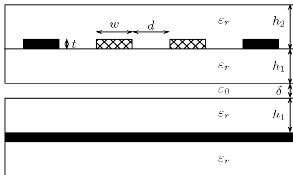
Fig. 1. Cross-section of the transmission-line under investigation. Crosshatch and solid fill indicate signal and ground conductors, respectively. The air-gap \delta is generated between two flexible printed circuit layers when the layers are turned and slid over each other in moving mechanisms.
