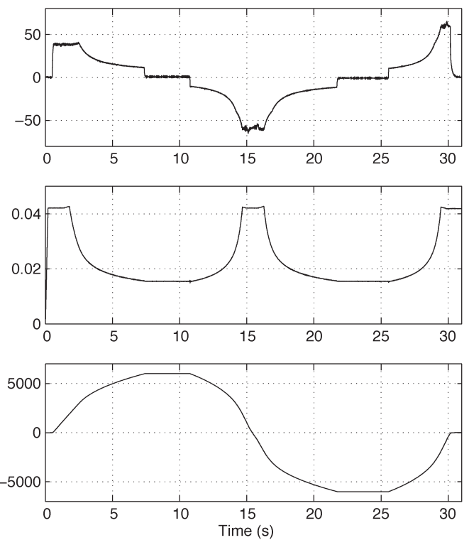
Fig. 13. Startup of the drive with inertial load to 6000 r/min ( \approx 600 Hz). From top to bottom: T_e (Nm); \lambda_s (Vs); and \omega_r (r/min).
