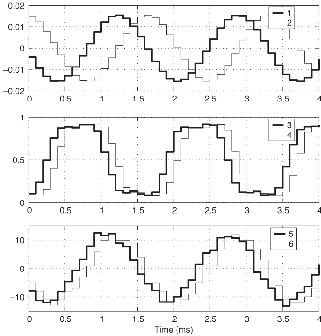
Fig. 15. Steady-state operation at 6000 r/min ( \approx 600 Hz) and no load. (1) \lambda_{s\alpha} (Vs); (2) \lambda_{s\beta} (Vs); (3) duty-cycle phase as \delta_{as} ; (4) duty-cycle phase xs \delta_{xs} ; (5) i_{s\alpha} (A); (6) i_{s\beta} (A).
