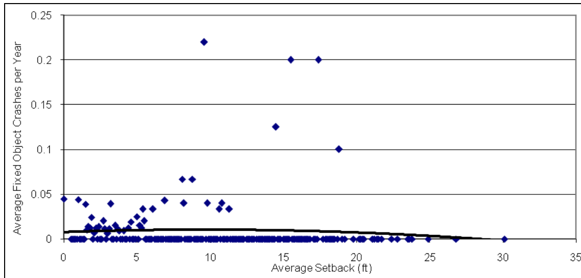
Figure 5-7. Average setback in 15 m analysis
