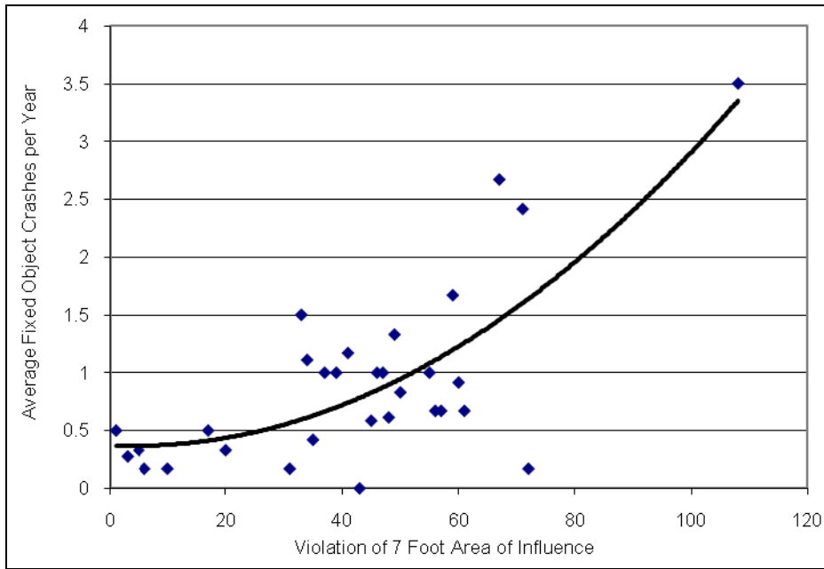
Figure 5-17. Violation of 7 ft area of influence in segment analysis
