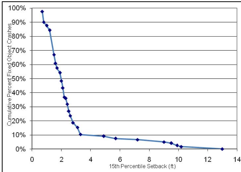
Figure 5-66. Cumulative percent 15th percentile setback in segment analysis at ADT over 6,000
