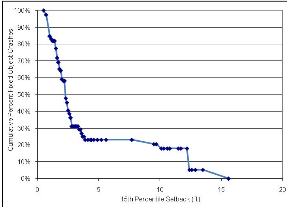
Figure 5-75. Cumulative percent 15th percentile setback in block analysis at 35 mph
