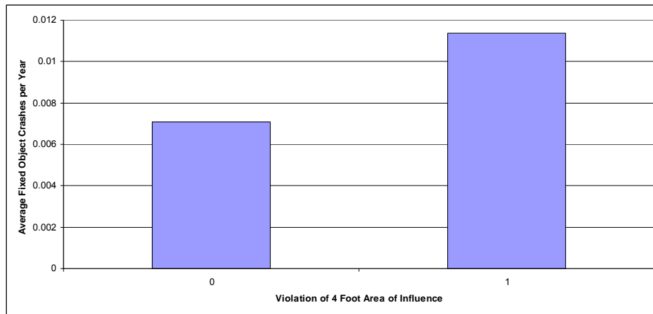
Figure 5-34. Violation of 4 ft area of influence in 15 m analysis
