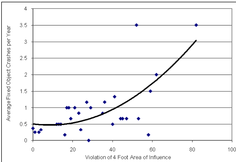
Figure 5-14. Violation of 4 ft area of influence in segment analysis
