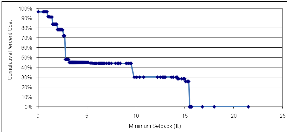
Figure 5-136. Cumulative cost minimum setback in 15 m analysis at 30 mph
