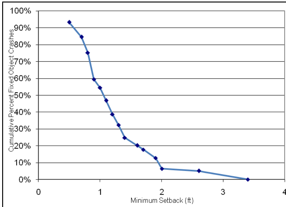
Figure 5-64. Cumulative percent minimum setback in segment analysis at ADT over 6,000
