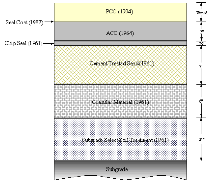
Pavement cross section
