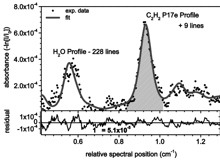
Figure 3 Experimental, emission and transmission corrected TDLAS line profiles and model fit data of the P17e C_2H_2 absorption line as well as the interfering H_2O spectrum, combining 228 H_2O lines.
