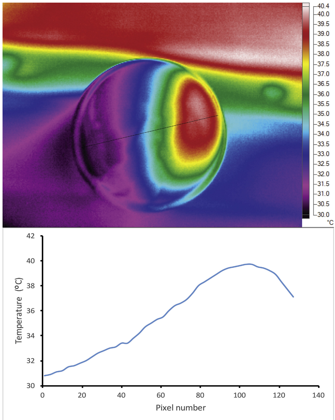
Fig. 2 – The upper panel shows the temperature distribution across a dry reference hemisphere in bright sunlight and low wind conditions, as recorded by the thermal camera. The temperature profile along the line across the centre of the dome is plotted in the lower panel.
