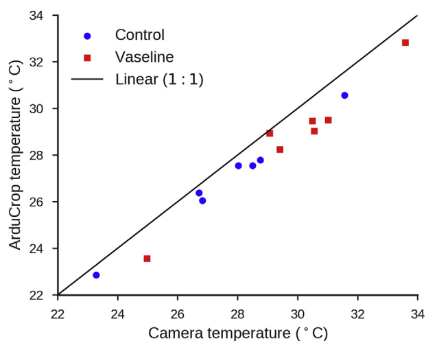
Fig. 3 – Relationship between ArduCrop estimates of canopy temperatures and camera estimates of temperatures of the same areas of canopy from the same view angle (data from 4th, 5th and 12th February, 2016). Each point represents the average of 16 measurements over 20–30 min periods (representative of a range of environmental conditions) with two separate ArduCrops at different representative positions in the crop (newly selected on each date). On average the camera estimate was 1.08 °C higher than the ArduCrop for the Vaseline canopy (red squares) and 0.71 °C for the control canopy (blue circles). The solid line denotes the 1:1 relationship. (For interpretation of the references to colour in this figure legend, the reader is referred to the web version of this article.)
