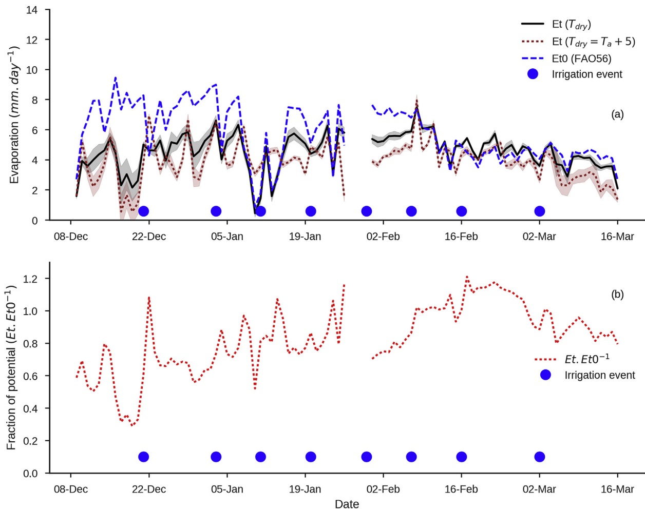
Fig. 5 – Daily Et ( T_{dry} , solid black line and T_{dry} = T_a + 5 , dotted brown line) and Et_0 (FAO56, dashed blue line) for the complete deployment on cotton (Kulki farm) (a) and the daily fraction of potential ( Et.Et_0^{-1} , dotted red line) (b). The scaling factor, \alpha , in Equation (1) was set equal to 0.5, being the value that scaled the calculated Et to Et_0 according to FAO56. Note the missing meteorological data from 26 to 30 Jan 2015. The dates of irrigation events are indicated by blue circles. For Et ( T_{dry} ) and Et ( T_{dry} = T_a + 5 ), the lines and shaded regions represent the mean and standard deviation, respectively, of three values (three ArduCrop dry reference sensors). (For interpretation of the references to colour in this figure legend, the reader is referred to the web version of this article.)
