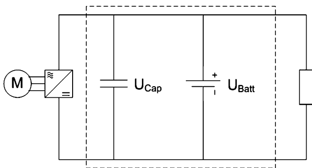
Fig. 5 Passive hybrid energy storage
