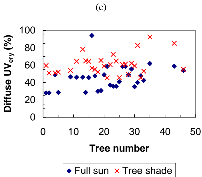
Figure 1 – The percentage diffuse erythemal radiation in the full sun and the tree shade in the (a) morning, (b) noon and (c) afternoon.
