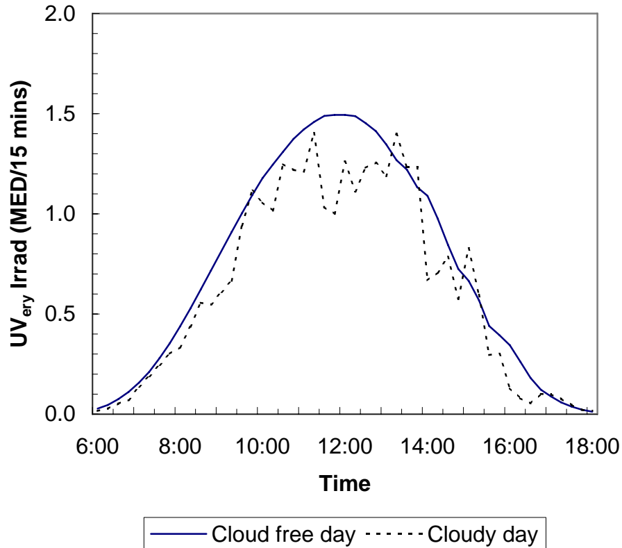
Figure 3 – Erythemal UV data for a relatively cloud free day and a cloudy day in summer.
