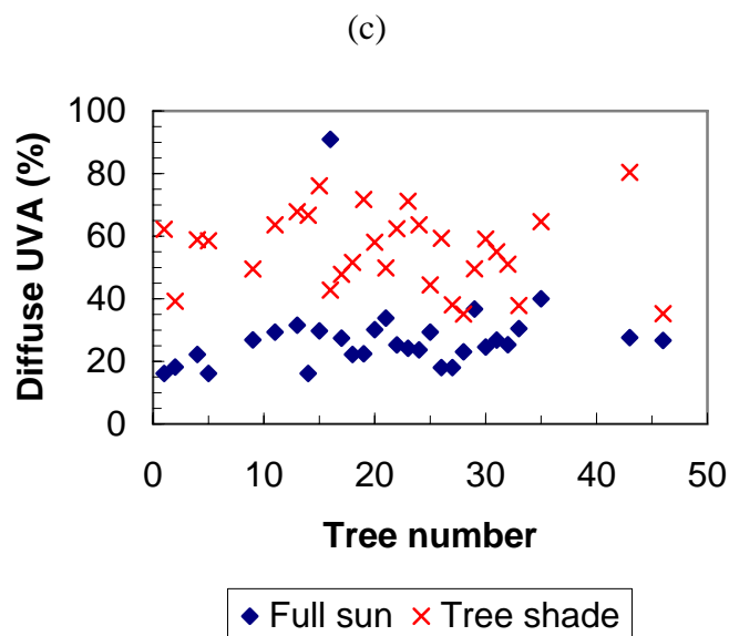
Figure 2 – The percentage diffuse UVA radiation in the full sun and the tree shade in the (a) morning, (b) noon and (c) afternoon.
