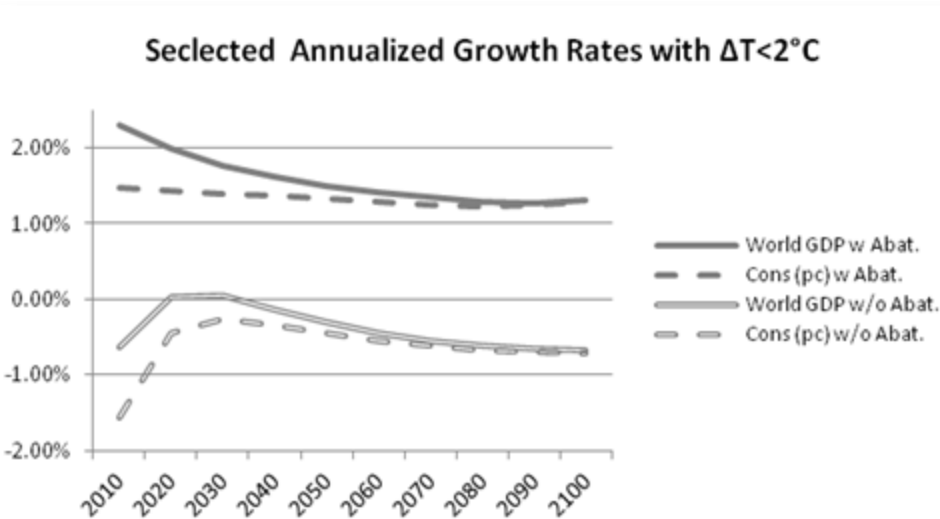
Figure 1: Optimal growth trajectories with and without mitigation in a neoclassical framework Source: Authors’ calculations
