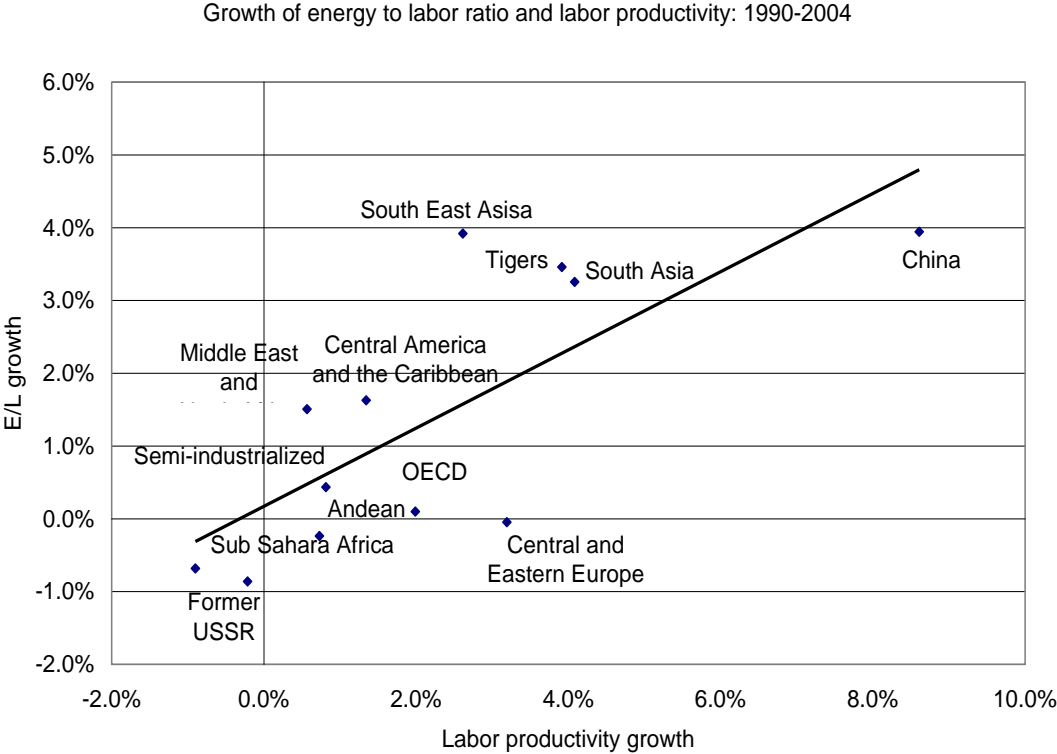
Figure 2: Relationship between the growth rates of labor productivity and energy intensity Source: Taylor (2009)
