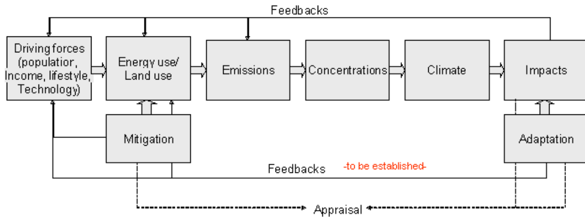
Figure 4: Integrated assessment analysis framework for assessing climate change policies including suggested feedback loops. Source: Van Vuuren et al., 2010.
