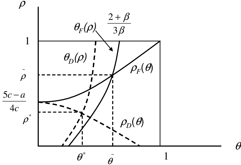
Figure 1: Equilibrium \theta and \rho
