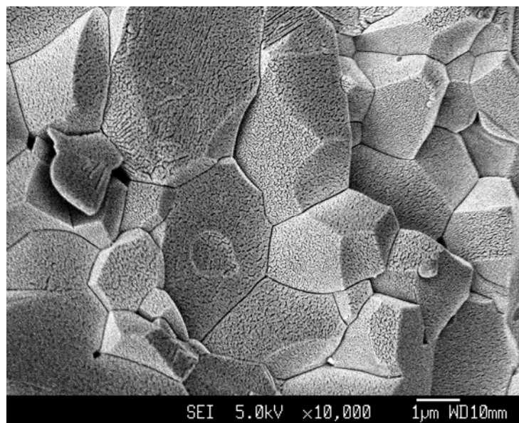
Fig. 8. SEM micrograph showing the fracture surface of a strut of the porous alumina.
