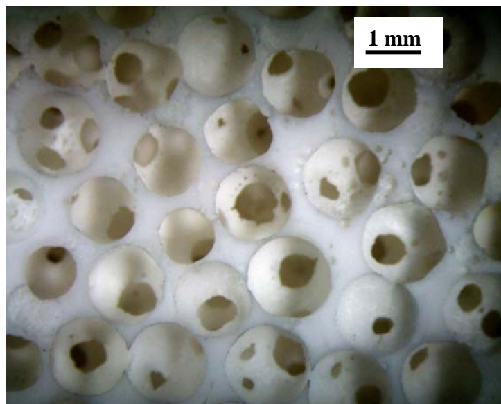
Fig. 5. Stereo-optical micrograph showing an overall porous structure of a porous alumina prepared using the EPS beads of 2.0 mm in size and compressed with the strain of 15 %.
