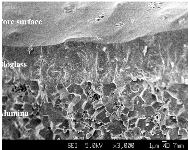
Fig. 9. SEM micrograph showing the fracture surface of a bioglass-coated alumina strut.
