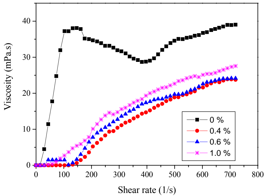
Fig. 4. Flow curves of alumina suspensions at a solid loading of 60 wt% and with different dispersant contents.
