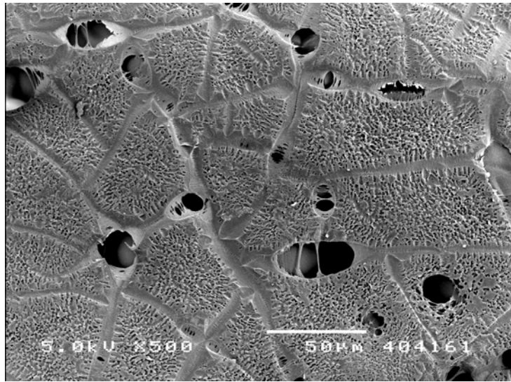
Fig. 2. SEM micrograph showing the surface morphology of the EPS bead.
