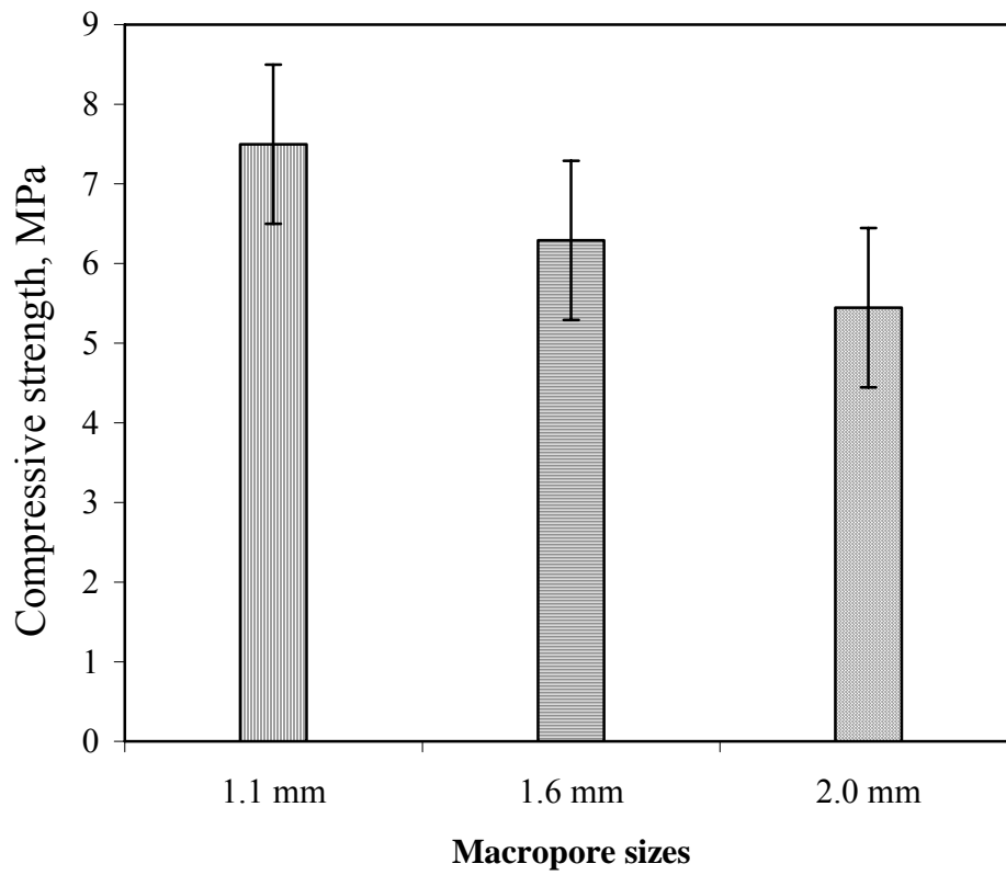
Fig. 7. The compressive strengths of the porous alumina ceramics prepared using EPS beads of different sizes.
