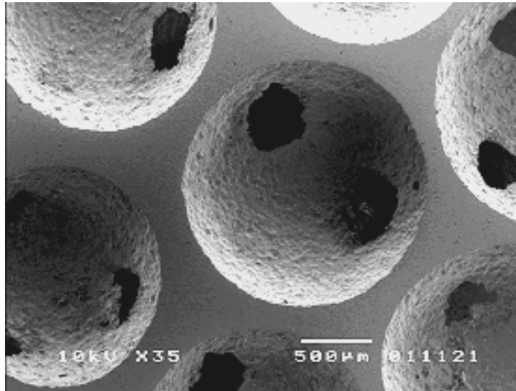
Fig. 6. SEM micrograph showing the pore windows in the macropores and the solid struts of the porous alumina prepared using EPS beads of 2.0 mm in size and compressed with the strain of 15 %.
