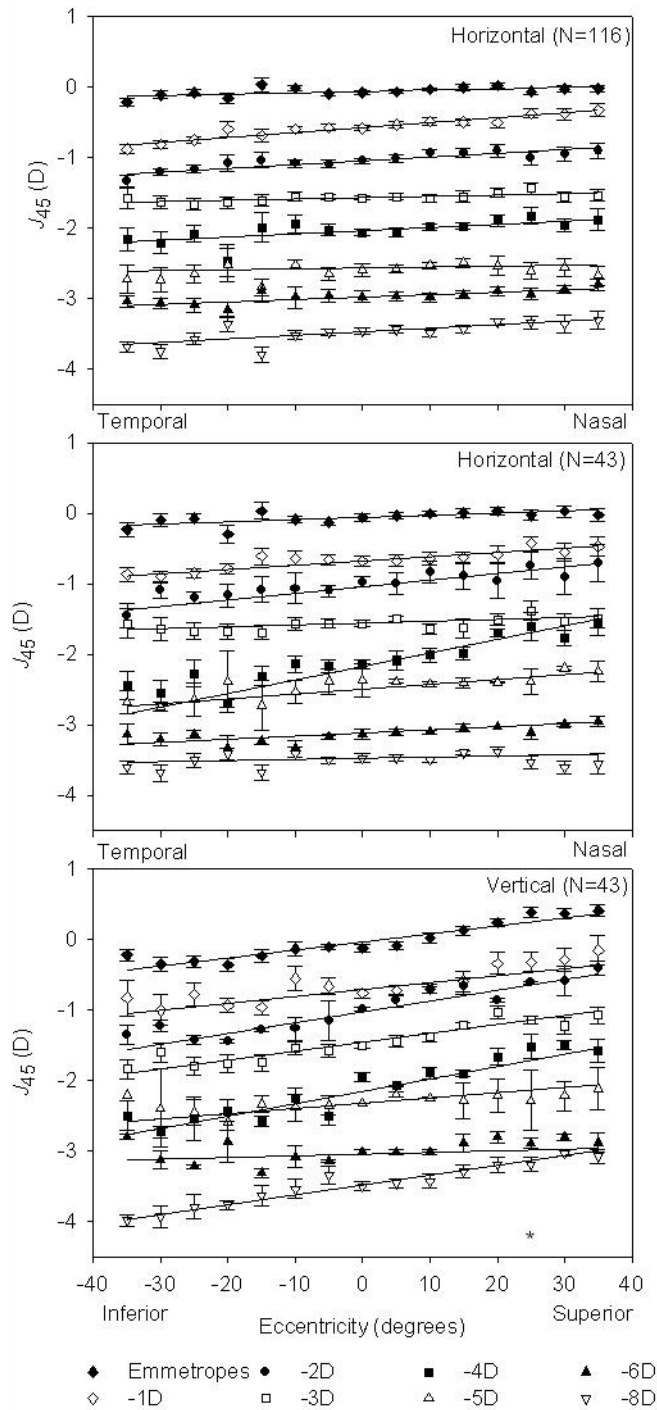
Fig. 3. Mean J_{45} astigmatism as a function of visual field angle for a) the horizontal visual field of all subjects ( n = 116 ), b) the horizontal visual field of the subset of subjects who also did vertical visual field measurements ( n = 43 ), and c) the vertical visual field ( n = 43 ). Errors bars indicate \pm SE (some error bars are smaller than the plot symbols). Visual field points marked with an asterisk are those for which the differences between peripheral and central J_{180} are significantly correlated with central M ( p < 0.05 ). Results for each myopic group (and the corresponding fitted curves) have been offset vertically for clarity by increments of 0.5 D such that the -8 D group is offset by 3.5 D. Curve fit coefficients before the offsets are shown in Table 2.
