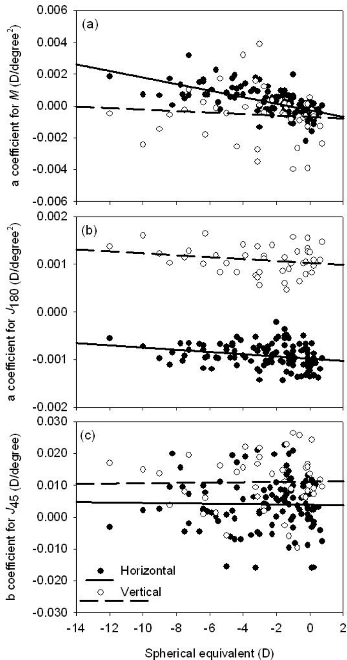
Fig. 4. Highest order co-efficient in Equations (2) for all subjects along both horizontal and vertical visual fields as a function of central spherical equivalent. a) Co-efficient “a” for mean spherical equivalent M , with y = -0.000206x - 0.000270 , adjusted R^2 = 0.42 , t = -8.43 p < 0.0001 , ( n = 116 ) horizontally, and y = -0.000047x - 0.000694 , adjusted R^2 = -0.016 , t = -0.59 , p = 0.56 ( n = 43 ) vertically; b) Co-efficient “a” for J_{180} astigmatism with y = -0.000023x - 0.000977 , adjusted R^2 = 0.056 , t = -2.79 , p = 0.006 , ( n = 116 ) horizontally, and y = -0.000020x + 0.001027 , adjusted R^2 = 0.056 , t = 1.44 , p = 0.16 ( n = 43 ) vertically; c) Co-efficient “b” for J_{45} astigmatism, with y = -0.000060x + 0.003897 , adjusted R^2 = -0.008 , t = -0.21 , p = 0.83 ( n = 116 ) horizontally, and y = +0.000051x + 0.011187 , adjusted R^2 = 0.121 , t = 0.12 , p = 0.90 ( n = 43 ) vertically [note that the constants in both equations are significant at t = 3.72 , p = 0.0003 horizontally and t = 6.12 , p < 0.0001 vertically]
