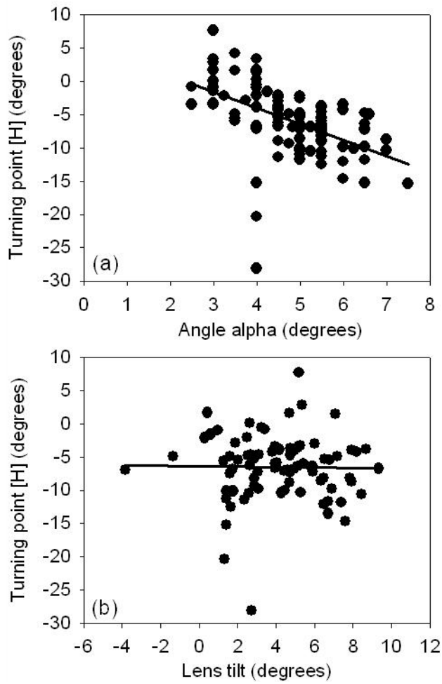
Fig. 6. The turning points of individuals' J_{180} astigmatism plots along the horizontal visual field as a function of a) angle alpha and b) horizontal lens tilt. Correlation coefficients and p-values of linear regression are a) adjusted R^2 = 0.27 , t = -6.25 , p < 0.0001 ( n = 108 ); b) adjusted R^2 = -0.001 , t = -0.14 , p = 0.89 ( n = 84 ).
