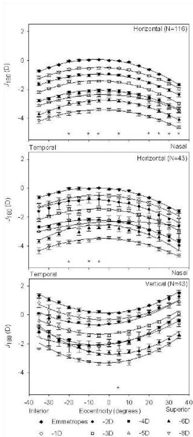
Fig. 2. Mean J_{180} astigmatism as a function of visual field angle for a) the horizontal visual field of all subjects ( n = 116 ), b) the horizontal visual field of the subset of subjects who also did vertical visual field measurements ( n = 43 ), and c) the vertical visual field ( n = 43 ). Errors bars indicate \pm SE (some error bars are smaller than the plot symbols). Visual field points marked with an asterisk are those for which the differences between peripheral and central J_{180} are significantly correlated with central M ( p < 0.05 ). Results for each myopic group (and the corresponding fitted curves) have been offset vertically for clarity by increments of 0.5 D such that the -8 D group is offset by 3.5 D. Curve fit coefficients before the offsets are shown in Table 2.
