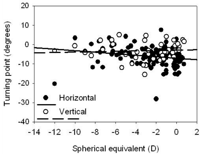
Fig. 5. The turning points of subjects' J_{180} astigmatism plots along the horizontal and vertical visual field as a function of central spherical equivalent. Correlation coefficient and p-value of linear regression are adjusted R^2 = 0.035 , t = -2.26 , p = 0.03 ( n = 116 ) horizontally, and adjusted R^2 = -0.020 , t = 0.43 , p = 0.67 ( n = 43 ) vertically.
