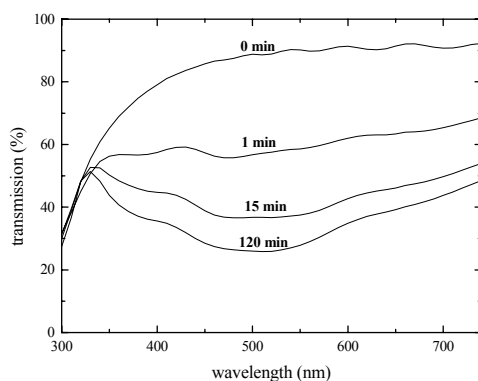
Figure 8. Darkening of the AgCl-doped coating after irradiation (700 W) [57, 58]
