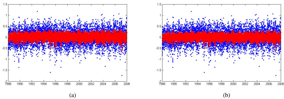
Fig. 14. Initialization of the final model for the wind data in New York using the BE method (a) and the fit of the trained network with 2 HU (b). The WN converged after 225 iterations.
