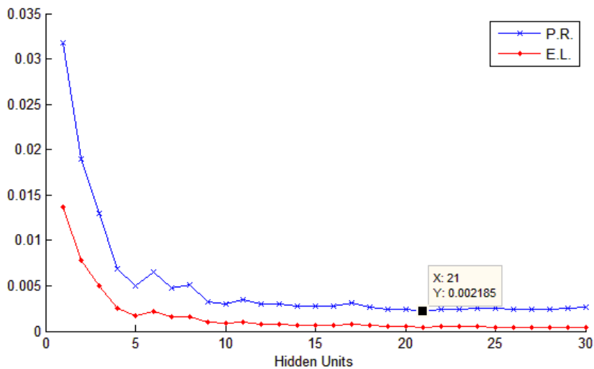
Fig. 15. The prediction risk (P.R.) and empirical loss (E.L.) for the first 30 hidden units for the Mackey-Glass equation.
