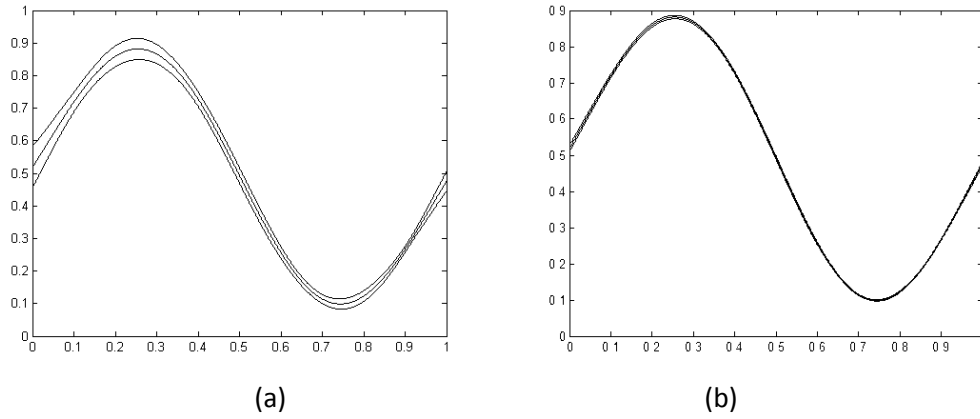
Fig. 7. Confidence intervals for the first case using the bagging (a) and balancing (b) method
