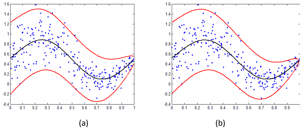
Fig. 9. Prediction intervals for the first case using the (a) bagging ( PICP=98\% ) and (b) balancing ( PICP=95\% ) method
