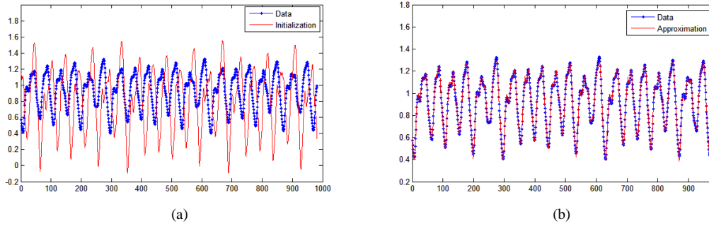
Fig. 16. The (a) initialization of the WN using the BE method and 21 HUs and (b) the approximation of the WN after the training phase for the Mackey-Glass equation.
