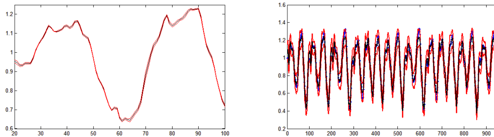
Fig. 18. In-sample confidence intervals (a) and out-of-sample prediction intervals (b) for the Mackey-Glass equation using the balancing method ( PICP=98.8\% ).
