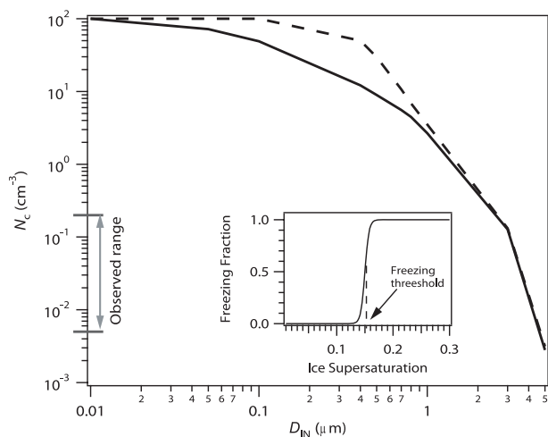
Fig. 2. Simulations of ice crystal concentration by pure heterogeneous freezing. N_c is presented as a function of the initial size of the ice nuclei. Conditions (Lawson et al., 2008) used were T = 185 K, p = 100 hPa, and vapor-to-ice deposition coefficient, \alpha_d , of 0.07 (dashed line), and 1.0 (solid line). The IN population was assumed to be monodisperse with total number concentration of 100 \text{ cm}^{-3} (Lawson et al., 2008). Freezing of solid ammonium sulfate was assumed to occur in a “burst” around the heterogeneous freezing threshold described by sigmoidal freezing spectrum with inflection point S_{\text{het}} = 15\% (Abbatt et al., 2006), where 99% of the aerosol freeze within a 2% supersaturation interval about S_{\text{het}} (inset plot).
