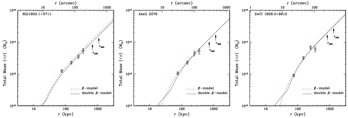
Fig. 5. Total mass profiles for the isothermal \beta -model and double \beta -model shown as dashed and continuous lines, respectively. The dots represent the total mass profile derived from the measured deprojected temperature profile by fixing the density profile to the best fit of the double \beta -model. The arrows indicate the radii at overdensities of 500 and 200 times the critical density.
