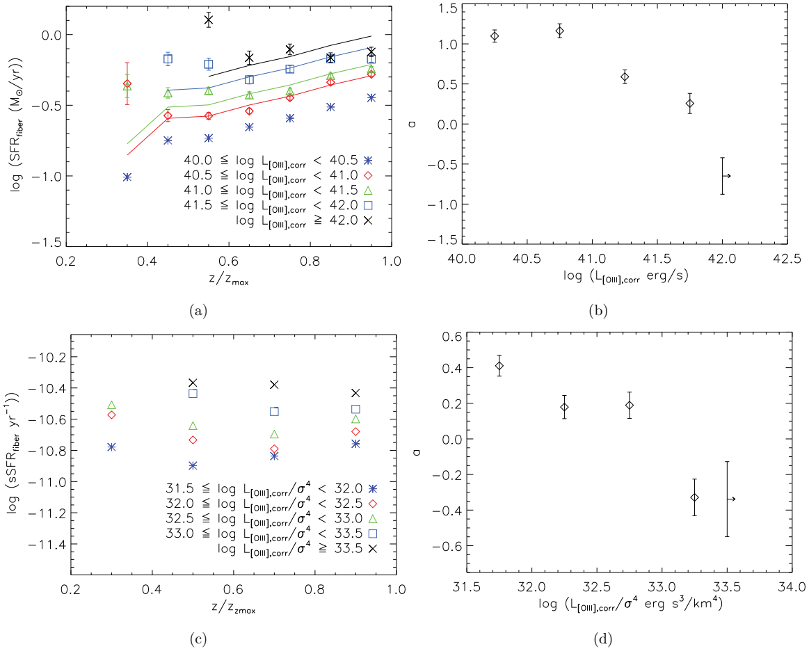
Figure 3. (a) \log(\text{SFR}_{\text{fiber}}) as a function of z/z_{\text{max}} in increasing L_{[\text{OIII}],\text{corr}} bins and (b) the best-fit slope in each bin. (c) \log(\text{sSFR}_{\text{fiber}}) as a function of z/z_{\text{max}} in increasing L_{[\text{OIII}],\text{corr}}/\sigma^4 bins and (d) the best-fit slope in each bin. At higher AGN luminosities and accretion rates, galactic star formation becomes more centrally concentrated. The lines in (a) correspond to the best-fit parameters from \text{SFR}_{\text{fiber}} = \text{SFR}_{\text{nuclear}} + \text{SFR}_{\text{disk}} , where \text{SFR}_{\text{nuclear}} = \alpha (M_{\odot} \text{yr}^{-1}) \times (L_{[\text{OIII}],\text{corr}}/10^{42} \text{erg s}^{-1})^{\beta} and \text{SFR}_{\text{disk}} is \text{SFR}_{\text{fiber}} associated with the lowest AGN luminosity bin (i.e., 40.0 < \log(L_{[\text{OIII}],\text{corr}} < 40.5 dex). From a reduced \chi^2 minimization, we find \alpha = 0.44 \pm 0.02 and \beta = 0.36 \pm 0.04 .
