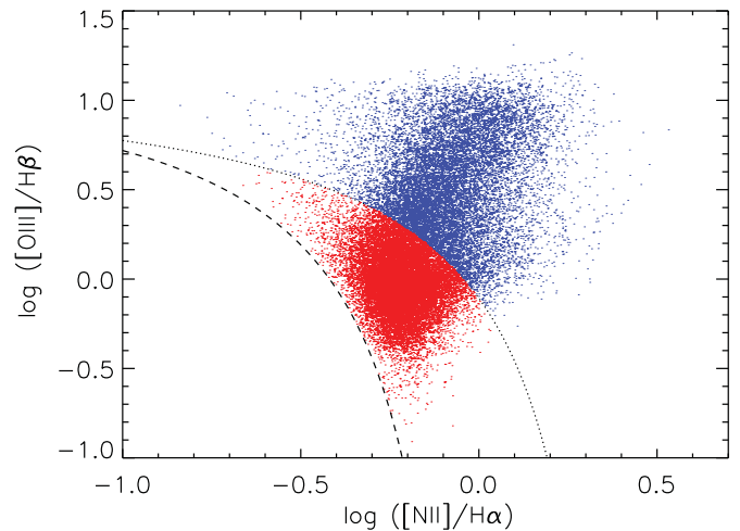
Figure 1. BPT diagram for galaxies used in our analysis. The lower dashed line represents the empirical boundary between star-forming galaxies and active systems from Kauffmann et al. (2003a) while the upper dotted line delineates the maximum theoretical starburst line from Kewley et al. (2001). There are 15,508 composite galaxies (red data points, between the two curves) and 12,444 Sy2 galaxies (blue data points). These composite systems represent the subset of composites in which the AGN contribution to [O\text{ III}] emission is estimated at \geq 30\% of the total.
