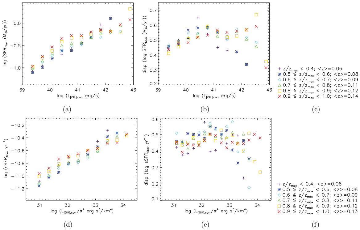
Figure 2. (a) SFR_{\text{fiber}} as a function of AGN luminosity and (d) sSFR_{\text{fiber}} as a function of Eddington parameter in increasing z/z_{\text{max}} bins, (b, e) associated dispersions, and (c, f) legends. The legends give the median redshift of the galaxies in each bin: with increasing redshift, the projected physical aperture size grows, encompassing greater amounts of the host galaxy. The relationship between AGN luminosity and star formation shows a dependence on the amount of the host galaxy that is sampled at lower AGN luminosities, but not at higher ones. The slope of the relation between sSFR and Eddington parameter becomes flatter as the aperture size grows, meaning that the star formation in more luminous AGN is centrally concentrated.
