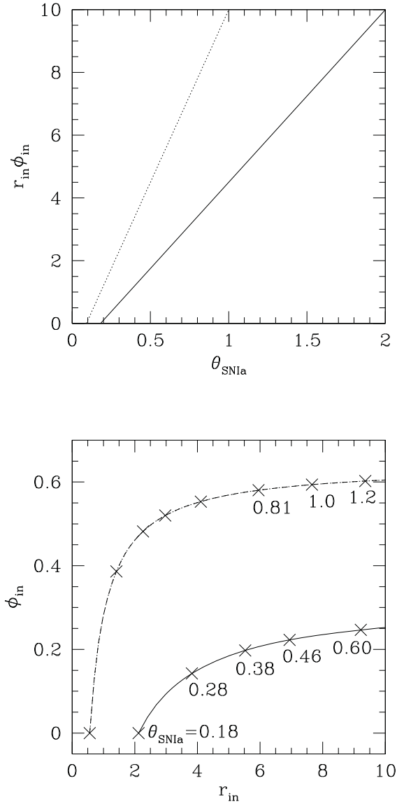
Figure 15. Top panel (a): r_{\text{in}}\phi_{\text{in}} vs. \theta_{\text{SNIa}} for the best-fit model (solid line in Figure 14). Also shown, is the corresponding curve for [Fe/H]_{\text{stars}} = -0.3 (dotted line). Bottom panel (b): \phi_{\text{in}} vs. r_{\text{in}} implied by the observed f_{\text{ISM}}^{\text{Fe}} for the best-fit abundance ratio patterns assuming [Fe/H]_{\text{stars}} = 0 and b_{\text{out}} = 0.0 (solid curve) or 1.0 (broken curve). The corresponding \theta_{\text{SNIa}} are shown by crosses; the first five values are the same for each curve. Abundance ratios are invariant along the lines in (a); abundances are invariant along the curves in (b) for the specified SNIa rates.
