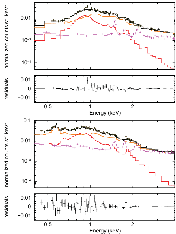
Figure 1. 6–8′ aperture Suzaku XIS source (NXB-subtracted) spectra and best simultaneous fit models to data from all three detectors (black data points and histogram in top panel), with residuals (bottom panel). Contributions from the ensemble of low mass X-ray binaries (if significant; LMXB, blue), from hot ISM thermal plasma components (red), and from the sum of GXB, CXB, and ICM background components (orange) are separately plotted. The NXB (purple), that is subtracted prior to spectral fitting, is also displayed. The top panel (a) shows the sum of the XIS0 and XIS3 spectra, folded through a weighted response, the bottom panel (b) shows the XIS1 spectrum.
