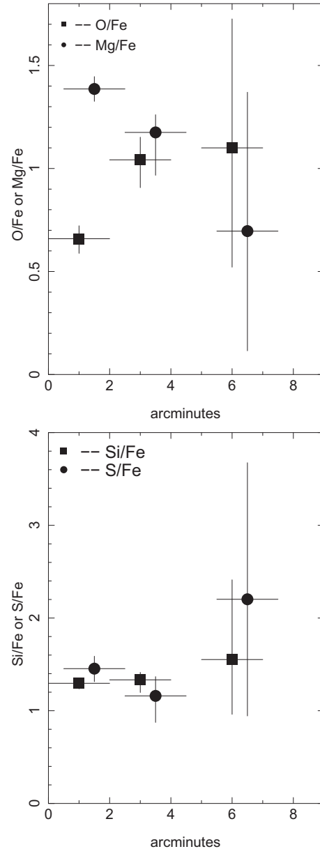
Figure 12. Profiles of abundance ratios with respect to Fe for O and Mg ( top panel, (a) ); and, Si and S ( bottom panel, (b) ) derived from the EPIC data.
