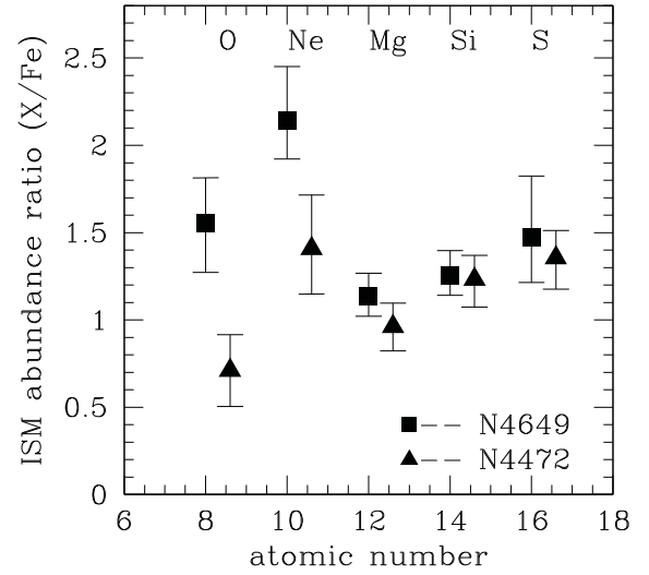
Figure 7. Abundance pattern comparison between NGC 4649 (solid squares) and NGC 4472 (solid triangles). The NGC 4472 values from Paper I have been rescaled to the Asplund et al. (2009) solar standard.
