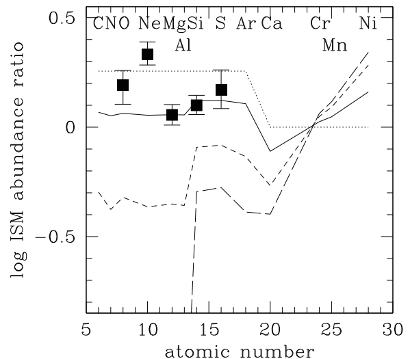
Figure 14. Best-fit model to the observed abundance pattern derived from Suzaku data (filled squares) assuming equal numbers of C-DEF, O-DDT, and WDD3 SNIa (solid line), compared with the ratios for pure stellar (dotted) and SNIa (long-dashed) enrichment and that for \theta_{\text{SNIa}} = 1 , r_{\text{in}}\phi_{\text{in}} = 0 (standard SNIa rate, no inflow; short-dashed line).
