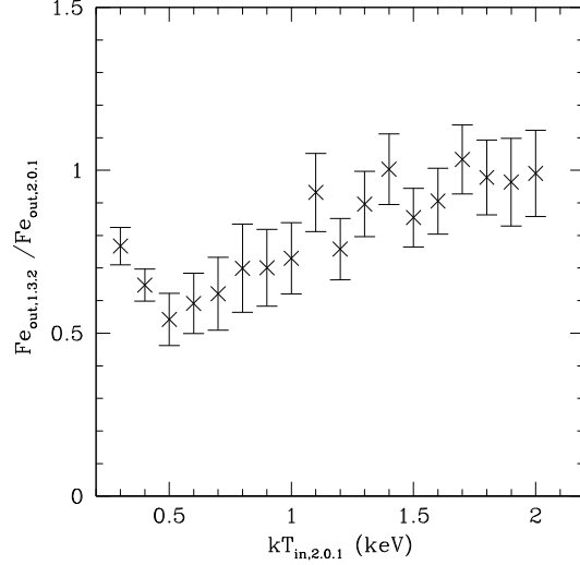
Figure 18. Ratio of the best-fit Fe abundance using AtomDB v1.3.2, to the best-fit that using AtomDB v2.0.1, versus simulation input temperature.
