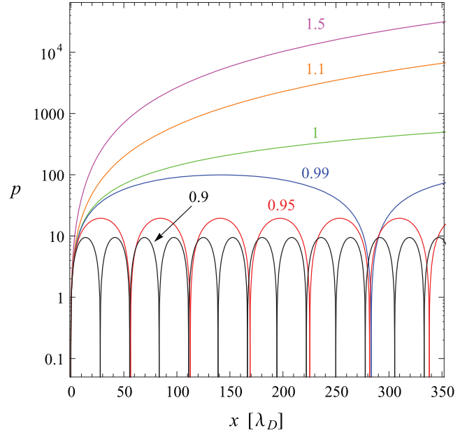
Figure 3. Phase space trajectories for stationary space charge limited flow for current densities j_m/j_{GJ} = 0.9, 0.95, 0.99, 1, 1.1, 1.5 . Note that in contrast to Fig. 2 the vertical axis on this plot is logarithmic.
