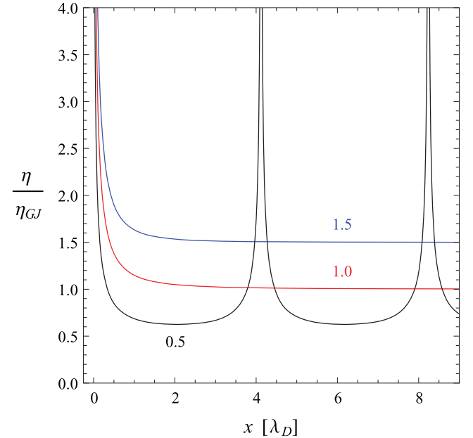
Figure 4. Charge density of stationary space charge limited flow normalized to the GJ charge density \eta_{GJ} as a function of distance x normalized to \lambda_{D,GJ} for current densities j_m/j_{GJ} = 0.5, 1.0, 1.5 .
