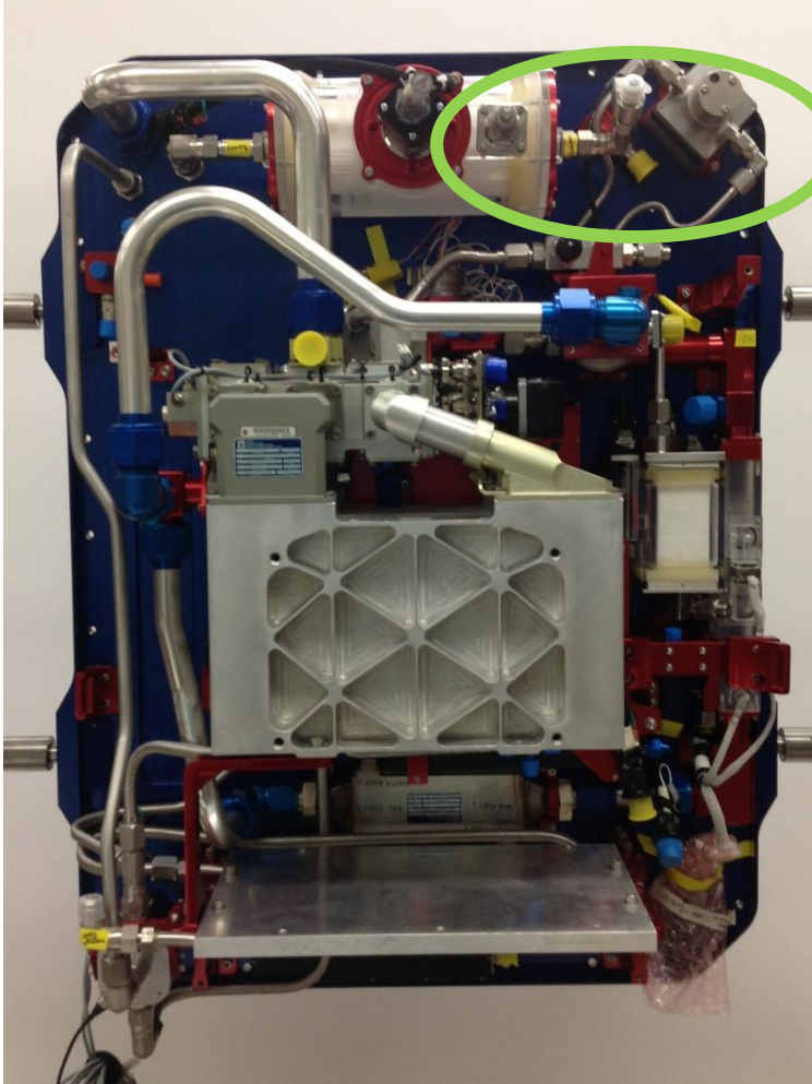
RVP SWME (circled in green) mounted on AEMU PLSS 2.0 Backplate.
