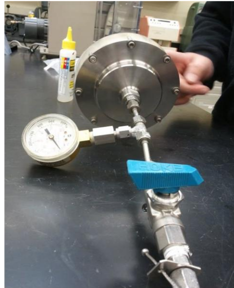
Plug Pressure Test Rig
