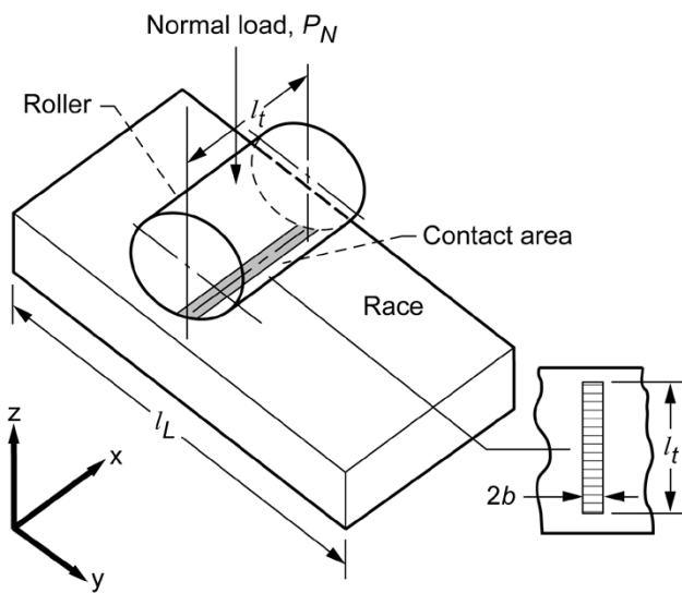
Figure 4.—Roller-race model for line contact.
