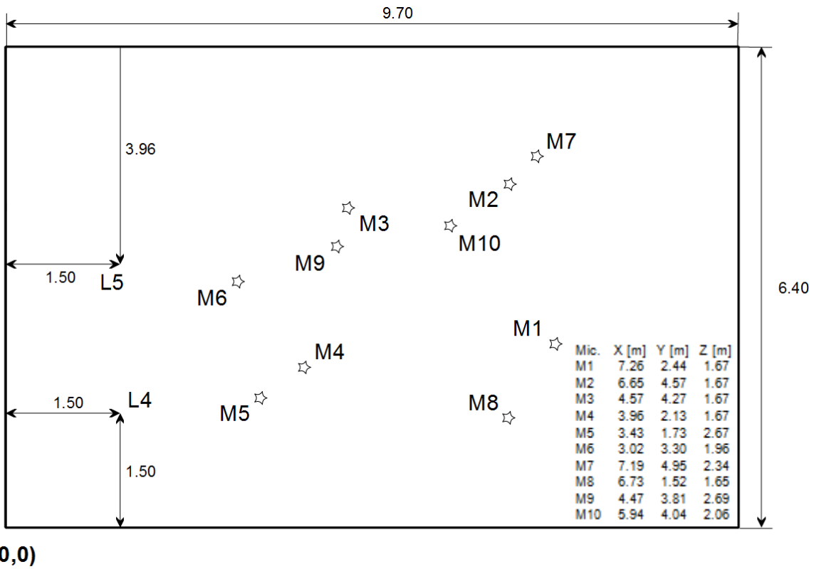
Figure 17. Sketch of the reverberation chamber layout for the ten-microphone variability measurements showing the two loudspeaker (L4 and L5) and the ten microphone (M1-M10) locations.
