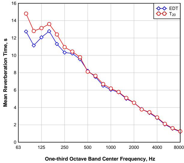
Figure 7. Mean measured EDT and T_{20} reverberation times with the MDF insert mounted flush in the TL window but without the two horns (Configuration A).
