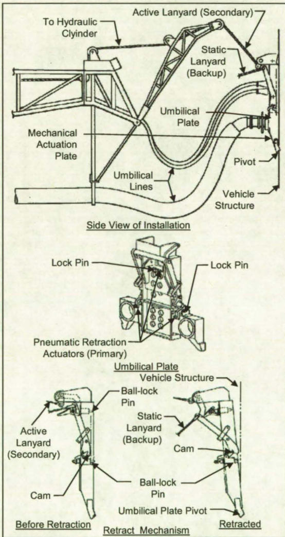
Figure 5. Redundant Retract Mechanism
