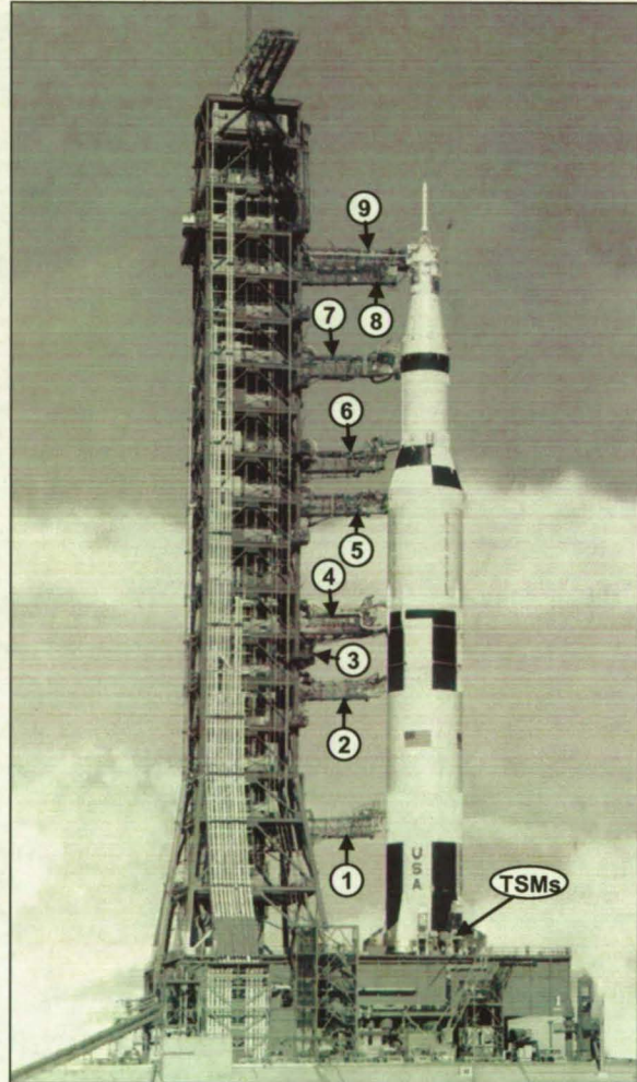
Figure 3. Saturn V TSM's and Service Arms (SA) 1-9 (SA-3 shown retracted)
