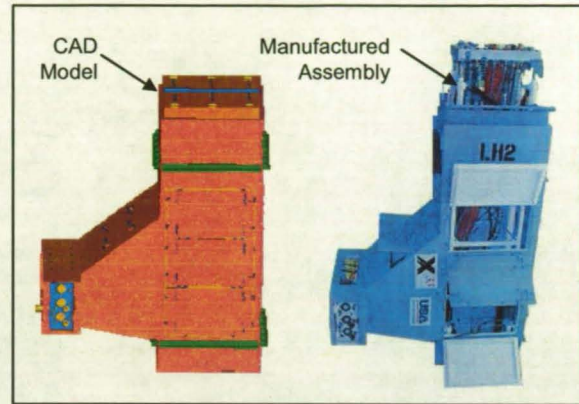
Figure 12. X-33 LH2 Umbilical Assembly CAD Model and Manufactured Assembly
