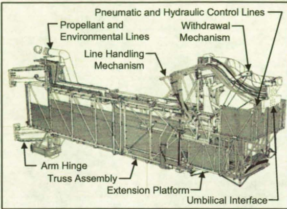
Figure 4. S-IVB Aft Service Arm (SA-6)
