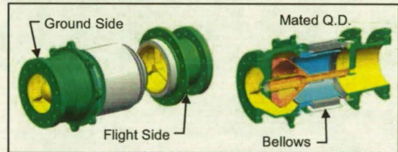
Figure 18. Bellows Type Quick Disconnect
