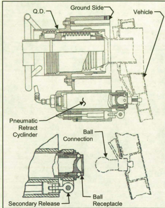
Figure 16. Ball-Locking Type Mechanism
