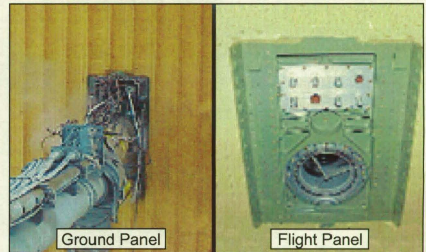
ET H2 Ground and Flight Panels
