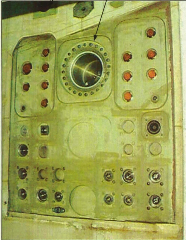
Shuttle LH2 Vehicle Side Plate
