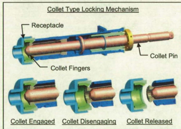
Figure 17. Collet Type Locking Mechanism
