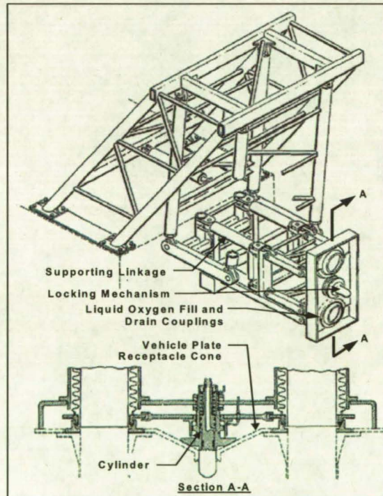
Figure 15. Self-aligning Umbilical (Saturn V – SIC Intertank)
