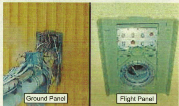
Figure 10. ET H2 Ground and Flight Panels
