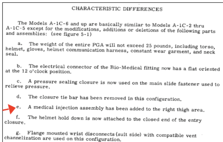
Figure 3. Text Excerpt noting addition of injection hardware to David Clark A-1C. Source: Apollo Block 1 Spacesuit Assembly, Model A-1C Technical Manual, November 1, 1965.
