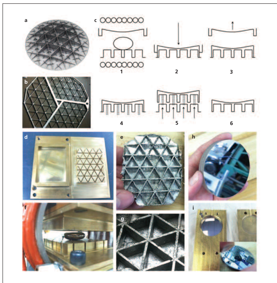
Figure (a) Example of an Isogrid Mirror Backing machined from a solid block of metal. (b) An aluminum isogrid machined from a solid plate. (c) The processing steps necessary to fabricate an amorphous metal mirror and isogrid in a single step. An ingot of amorphous metal or composite is heated using radio frequency heating while sitting on water-cooled molds. The liquid is forged into the mold and cools into a glass, which allows it to be ejected from the mold without sticking. With sufficient casting pressure, the isogrid and the mirror surface can be fabricated in one step. (d-g) The water cooled brass molds used to make the mirror, the isogrid, and the part after being ejected from the mold. (h) Example of a mirror assembly with isogrid backing all made from an amorphous metal. (i) A mirror polished steel mold with curvature acts as the template for casting a perfect metallic glass mirror (shown in the inset).
