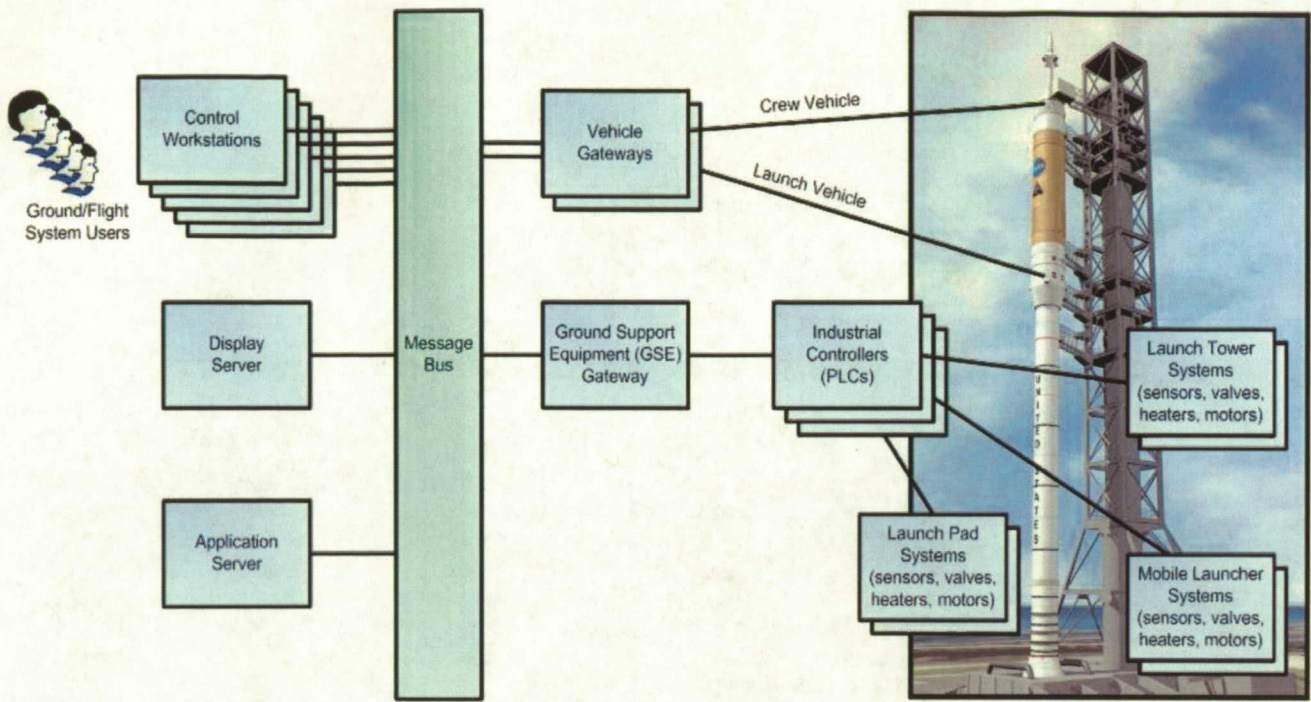
Figure 2 - Simplified Architecture of KSC's Launch Control System (LCS).
