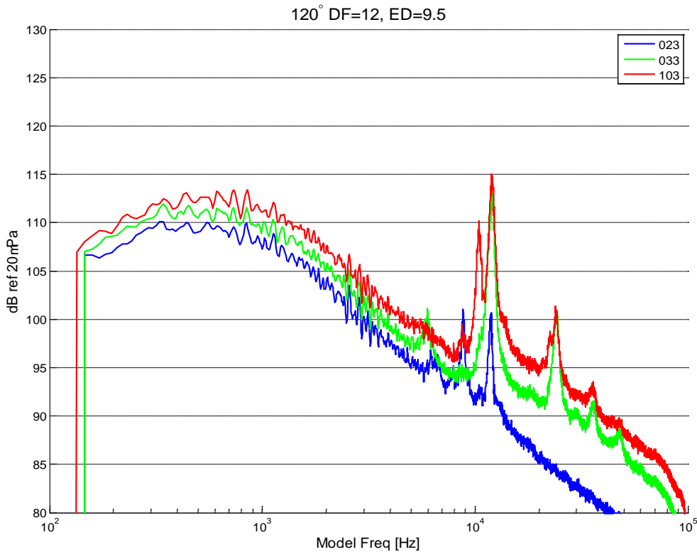
Figure 26 Effect of third stream pressure ratio on residual tone strength
