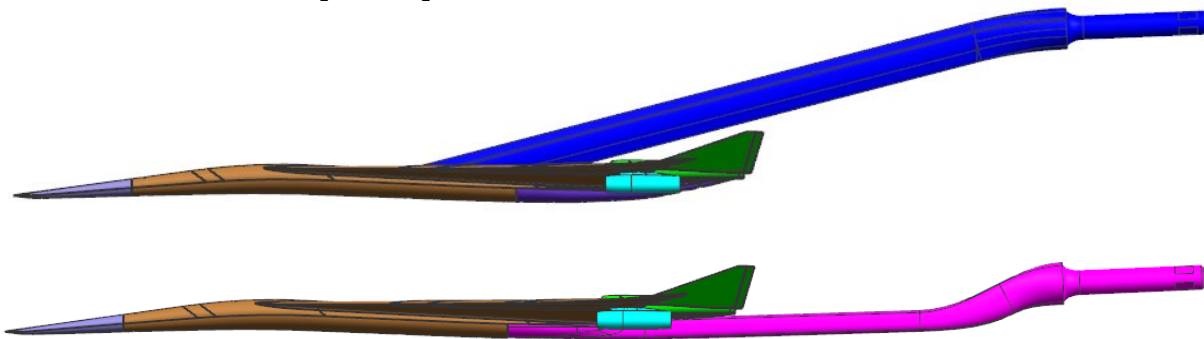
Figure 66. Both a sting and blade support system were designed and fabricated for the low boom test to reduce risk due to viscous effects at model scale
