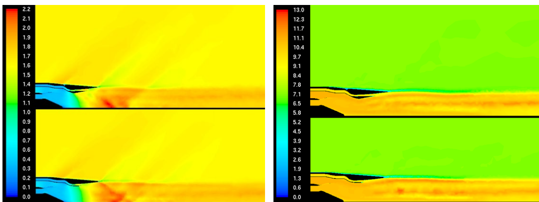
Figure 12 N+2 Mixer-ejector nozzle with Mach numbers and total pressures at Cruise, along 0° and 90° axial cuts, M = 1.6, altitude= 50,000 ft.
