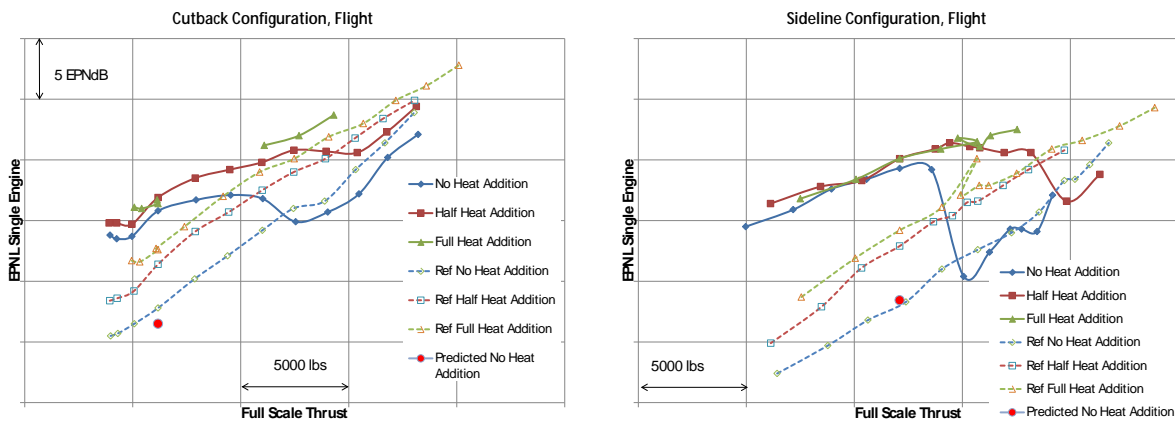
Figure 53 EPNL vs Thrust for cutback and sideline configurations including latest noise prediction.
