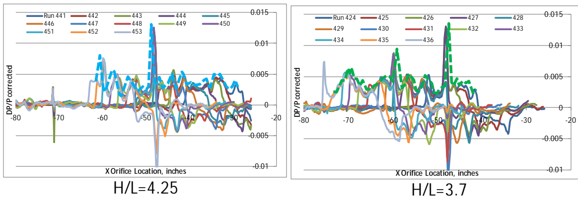
Figure 28. Variations of +/- 20% of Flat-Top Pressure Repeated at the Same Rail Position Despite Different Model Position
