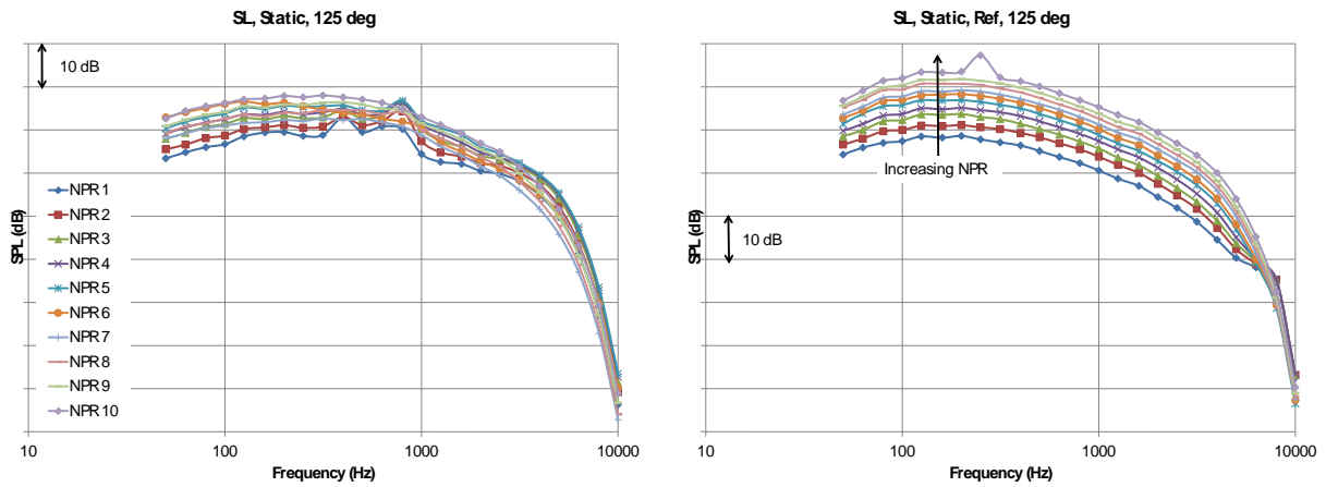
Figure 45 SPL at 125 deg for Sideline Configuration, Static Conditions, Processed to Sideline, No Heat Addition Cycle Conditions, Test Nozzle on Left, and Reference Nozzle on Right.
