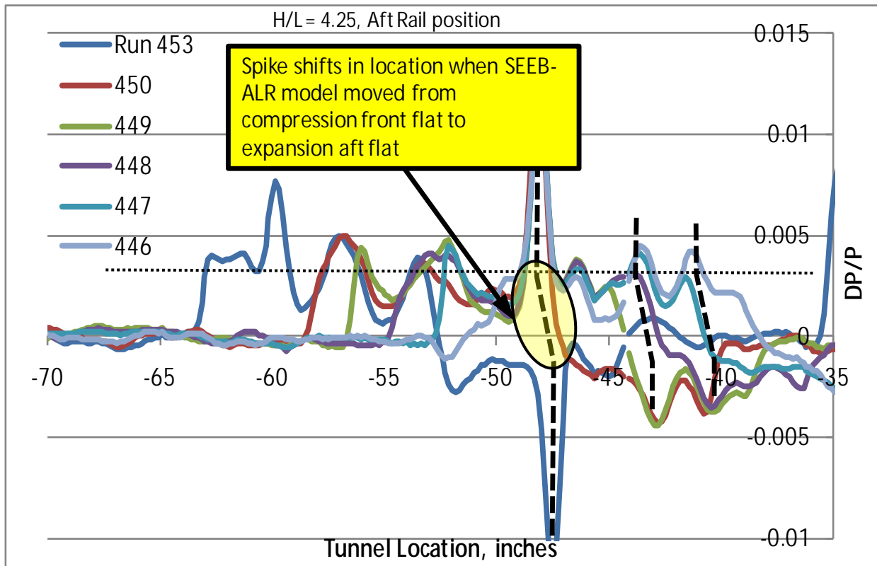
Figure 30. Measurement Sensitivity Spikes Shift with Model Induced Mach Angle Changes
