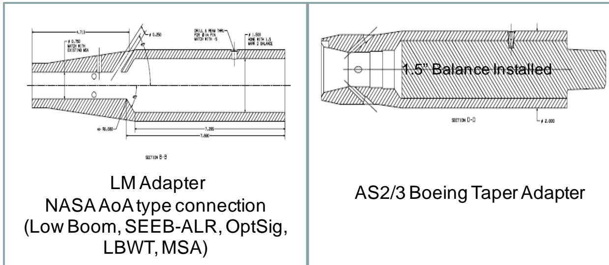
Figure 75. 1.5 in. Balance Adapters
