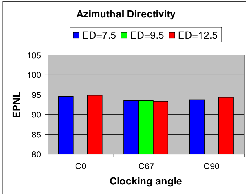
Figure 28 Effect of clocking angle (azimuthal directivity) on calculated EPNL (set point 103), all results at DF=10
