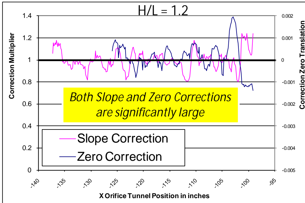
Figure 34. Calibrated Slope and Zero Correction
