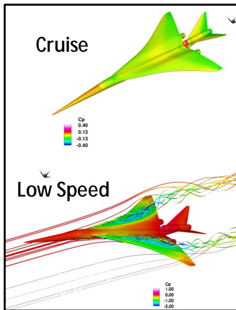
Figure 125. Smooth Flow at Cruise, Well-Controlled at Low Speed
