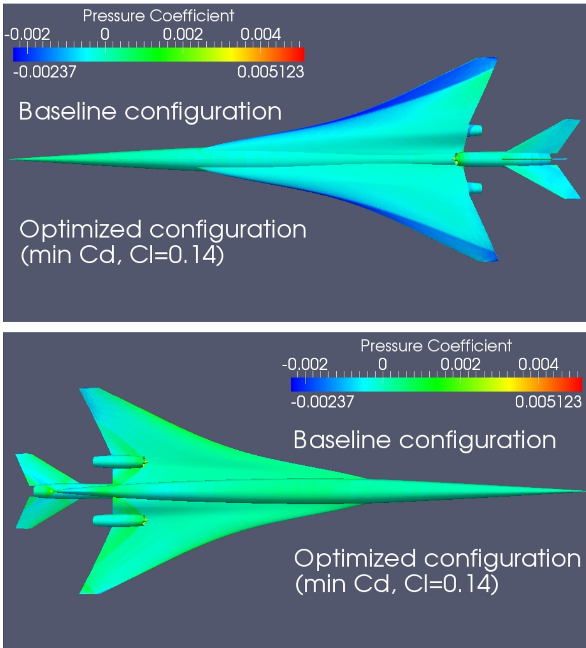
Figure 17. Shape design optimization (min Cd, Cl=0.14), upper and lower surfaces of the trijet.
