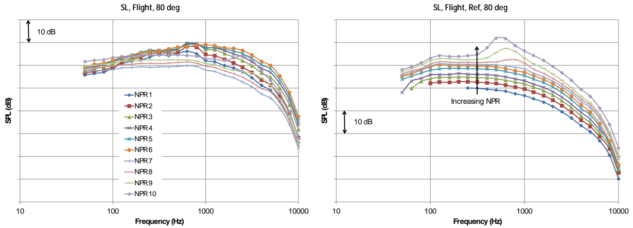
Figure 49 SPL at 80 deg for Sideline Configuration, Flight Conditions, Processed to Sideline, No Heat Addition Cycle Conditions, Test Nozzle on Left, and Reference Nozzle on Right.
