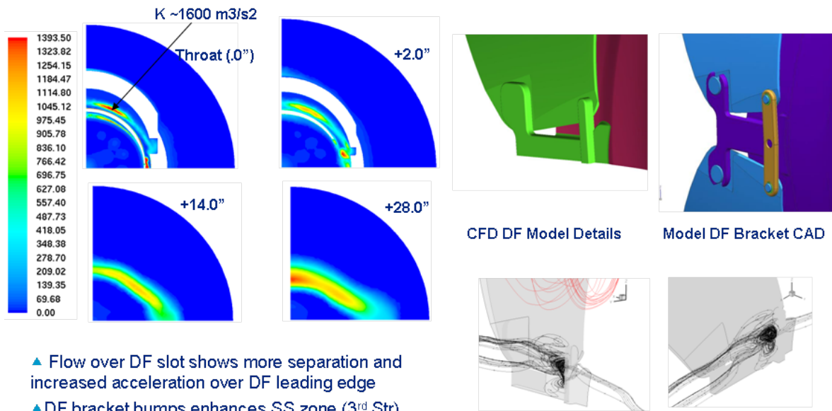
Predicted Path Lines around DF brackets
