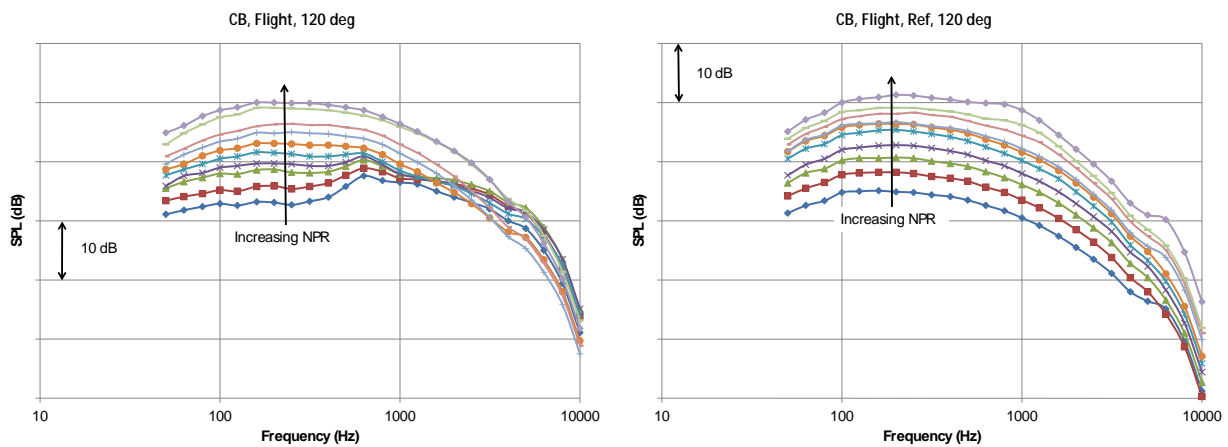
Figure 38 SPL at 120 deg for Cutback Configuration, Flight Conditions, Processed to Flyover, No Heat Addition Cycle Conditions, Test Nozzle on Left, and Reference Nozzle on Right.
