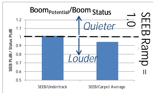
Figure 123. Current Low Boom Under-Track Better than SEEB
