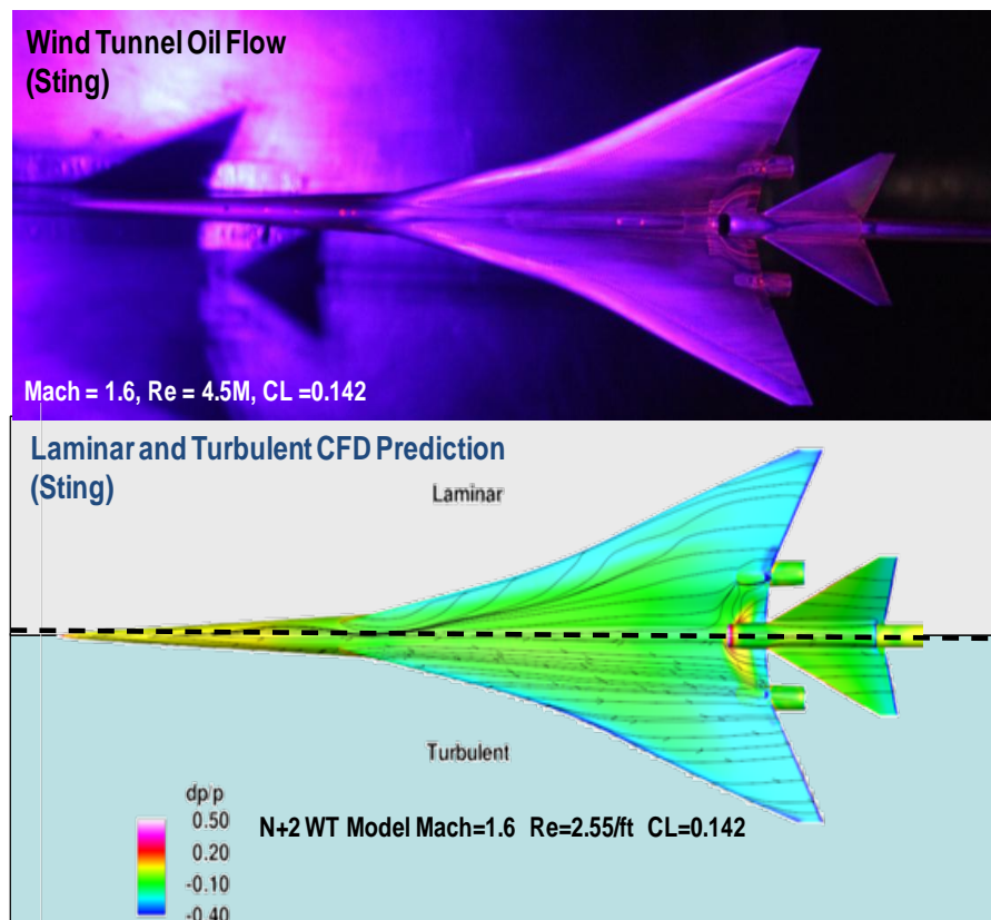
Figure 84. Oil flow showing fully attached like turbulent
