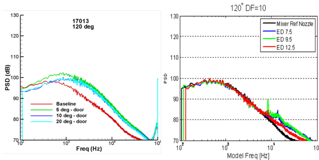
Figure 31 HVC10 data (left) compared to N+2 SUP data (right), showing that ejector noise had been significantly reduced
