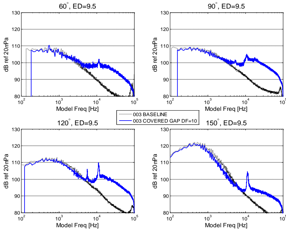
Figure 25 Repeat run of mixer ejector system with covered divergent flap gaps at set point 003 compared to reference nozzle. Divergent flaps set to 10 degrees, ejector doors set to 9.5 degrees, tones significantly reduced compared to Figure 23.
