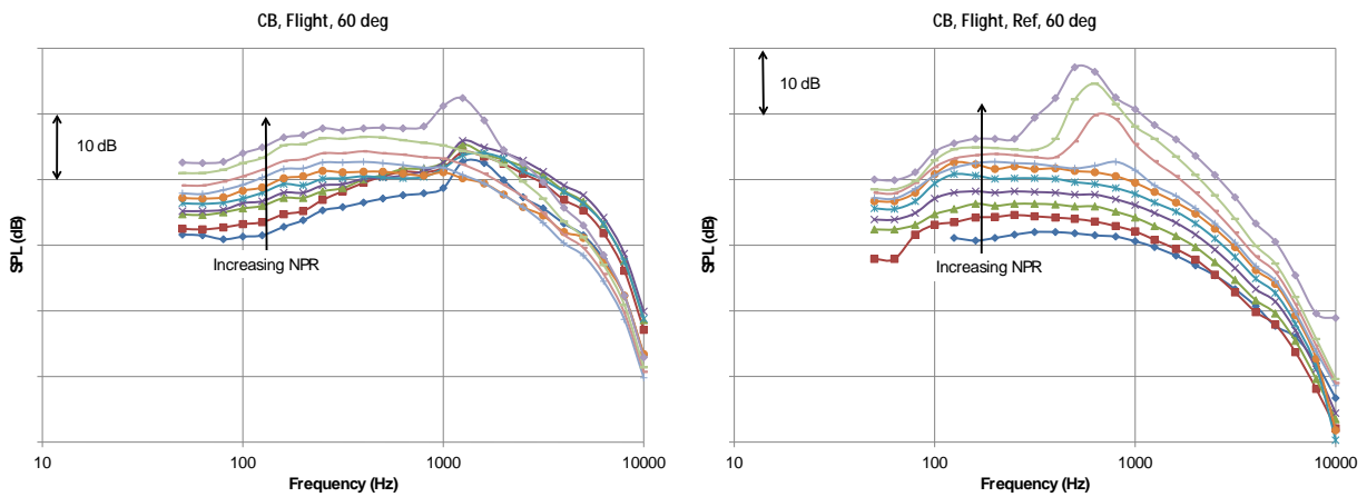
Figure 35 SPL at 60 deg for Cutback Configuration, Flight Conditions, Processed to Flyover, No Heat Addition Cycle Conditions, Test Nozzle on Left, and Reference Nozzle on Right.
