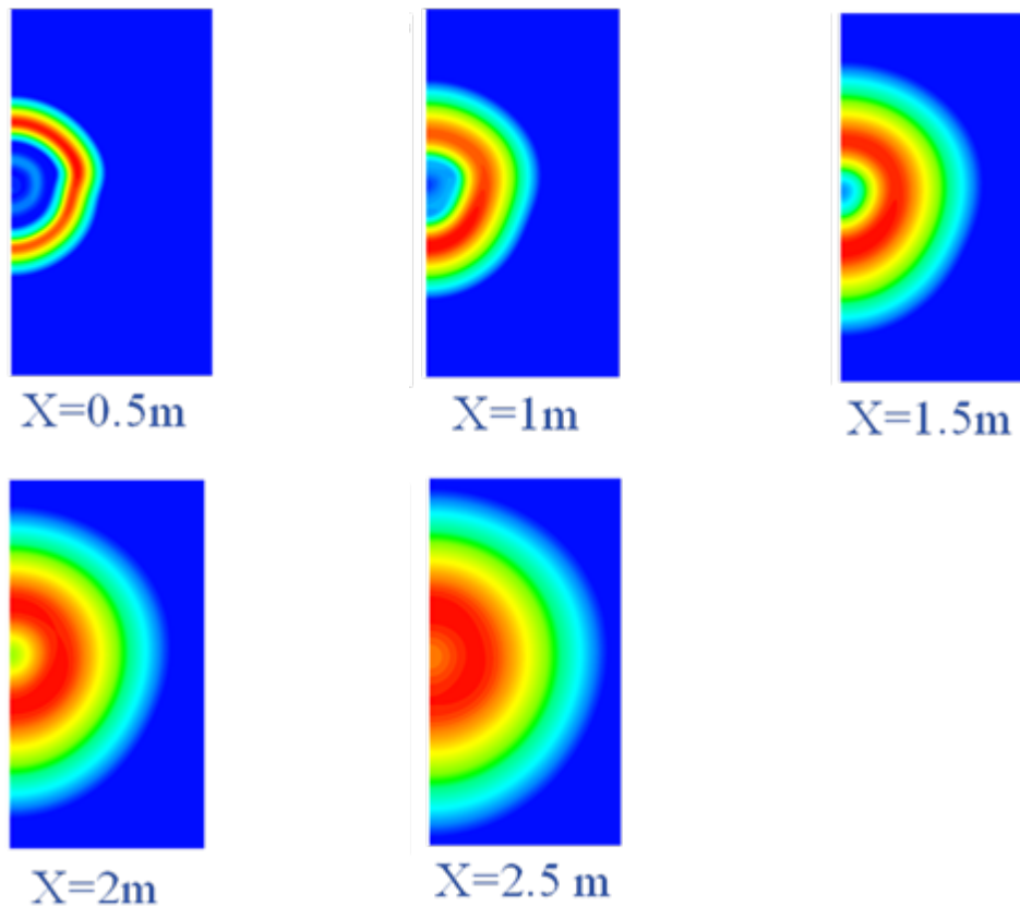
Figure 16 Contours of turbulent kinetic energy at different axial locations.
