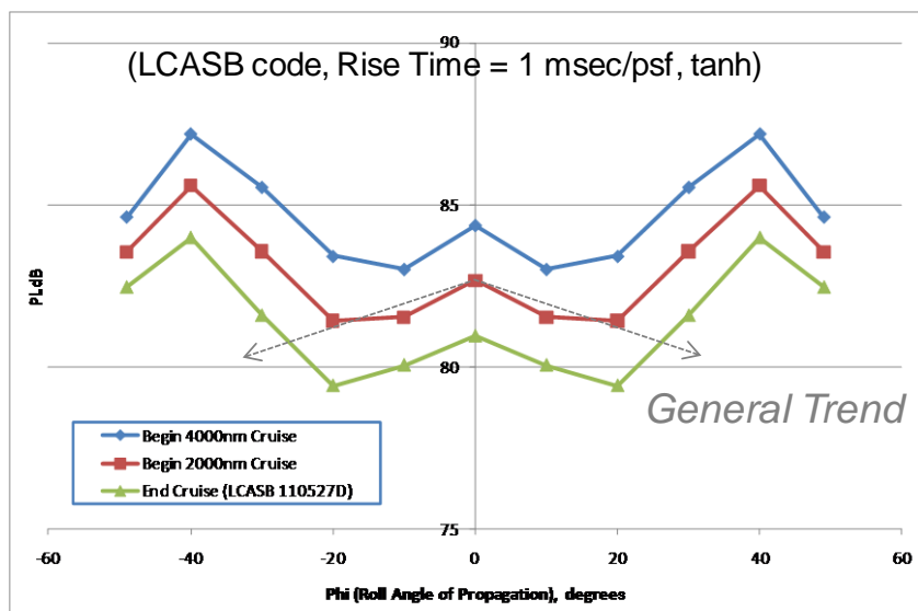
Figure 56. The QR4 1021-01 (N+2) Trijet configuration maintains a loudness level below 85 dB PL up to 28 degrees off-track at the start of cruise, and over the full carpet and mid-cruise and end-of-cruise
