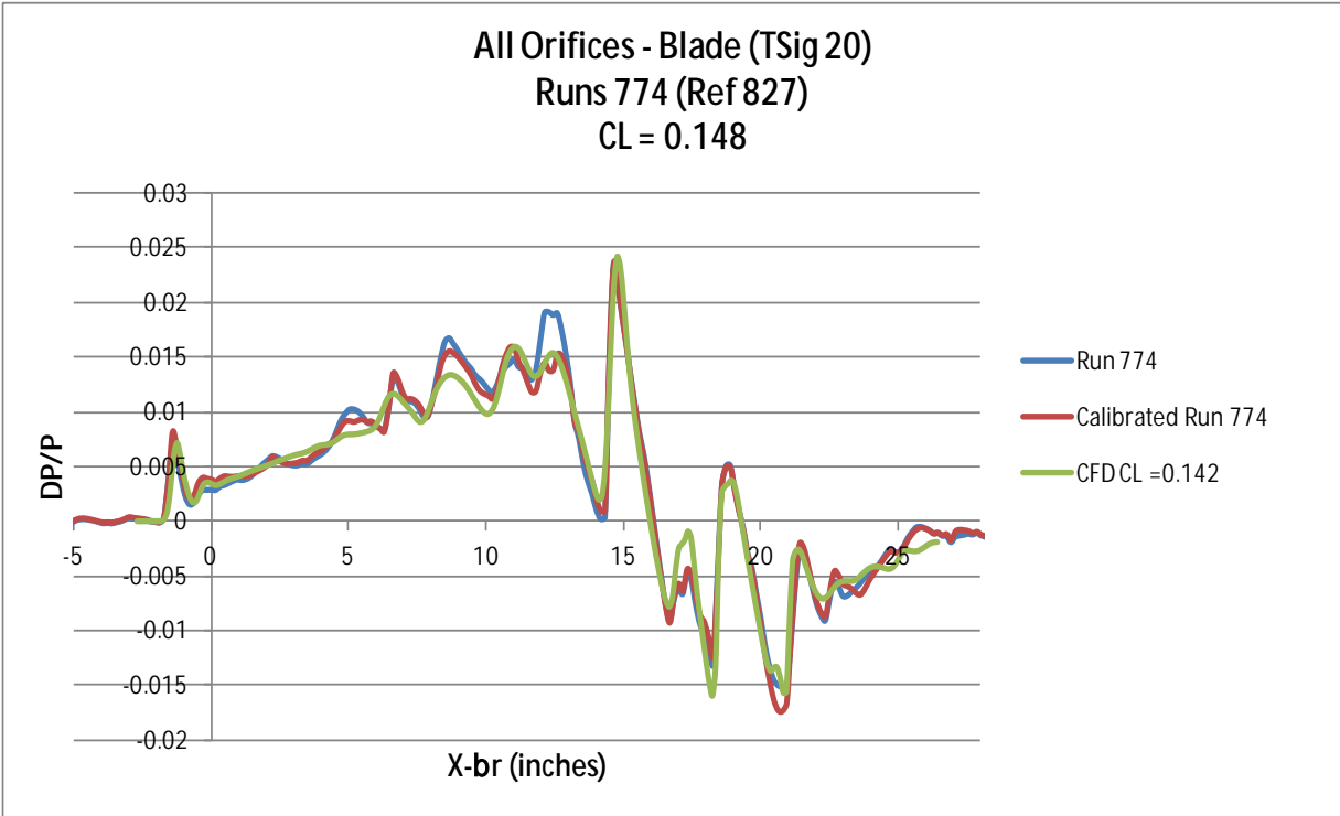
Figure 96. Calibration provides necessary improvement, but improvement is less necessary as runs available to average increases
