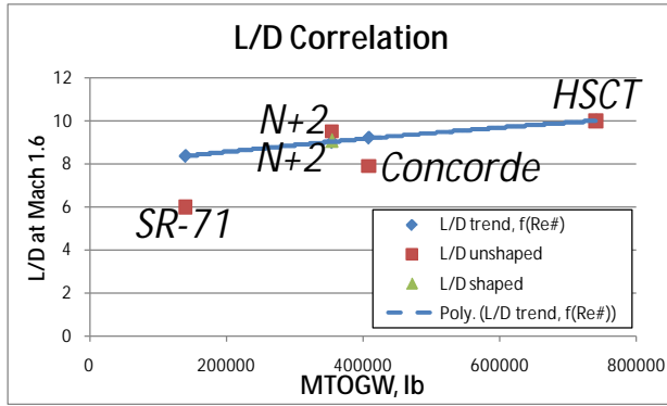
Figure 124. L/D with Low Boom Near Best Trend
