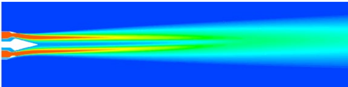
Figure 18 Contours of total temperature at the symmetric plane.
