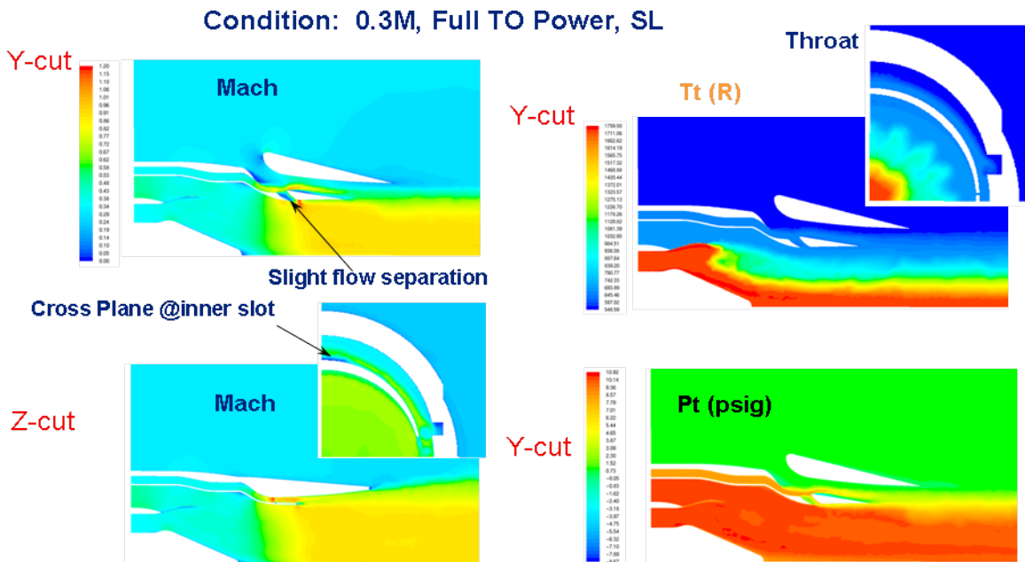
Mixer-ejector nozzle concept (patent pending)
