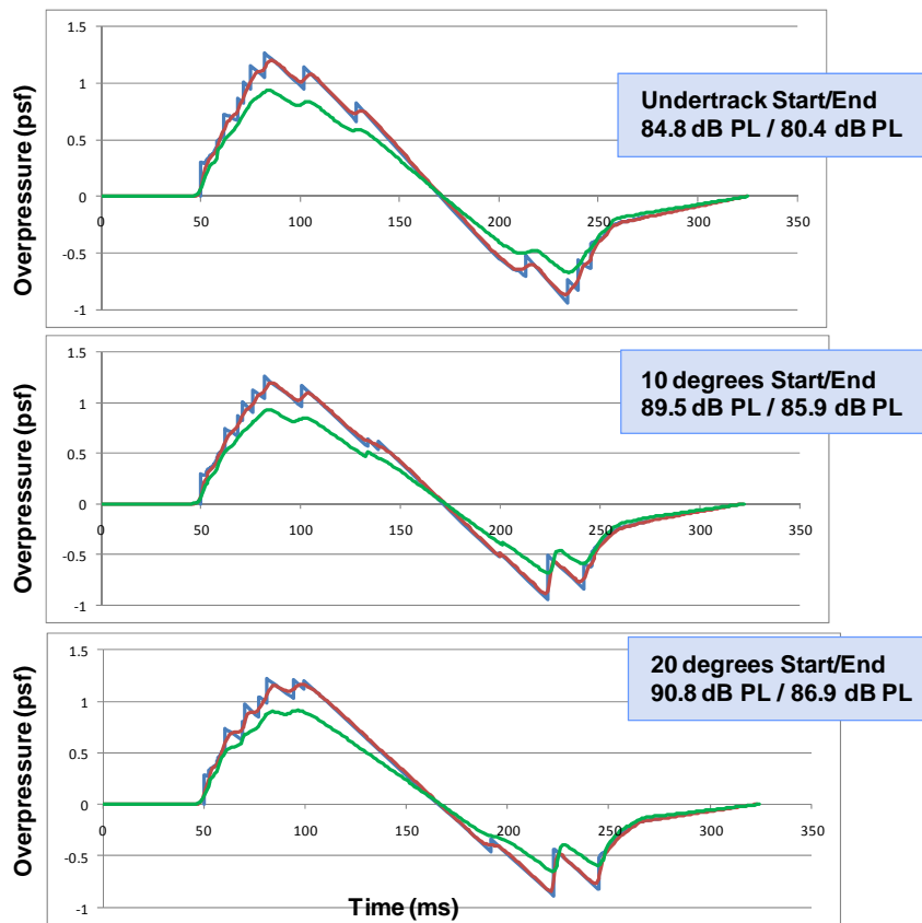
Figure 50. The loudness of the optimized Trijet configuration was reduced to below the 85 PL dB undertrack
