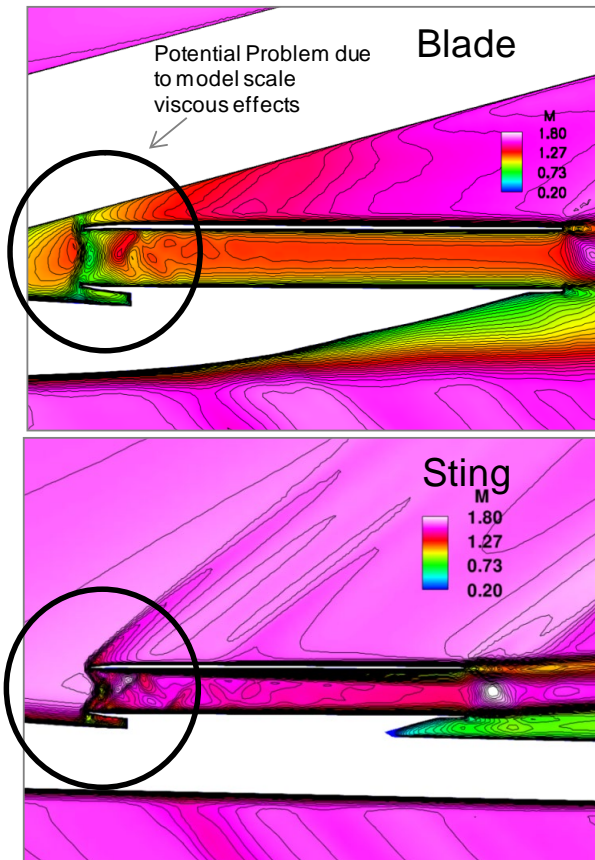
Figure 68. Viscous CFD predictions indicate the potential for a interaction between the blade mount and the centerline nacelle
