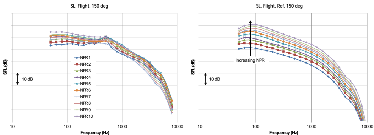
Figure 52 SPL at 150 deg for Sideline Configuration, Flight Conditions, Processed to Sideline, No Heat Addition Cycle Conditions, Test Nozzle on Left, and Reference Nozzle on Right.
