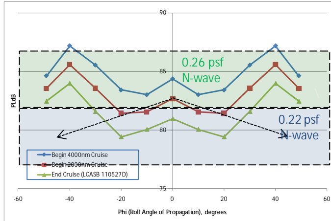
Figure 122. Current Low Boom Equivalent to 0.26 psf N-wave, Nearing Target of 0.22 psf N-wave
