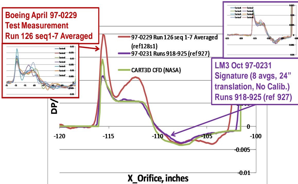
Figure 91. LM3 Good Match from 8 (90 sec) Measurements and Partial New Process. 97-0229 with 7 (2 sec) Measurements Converging with Reflections
