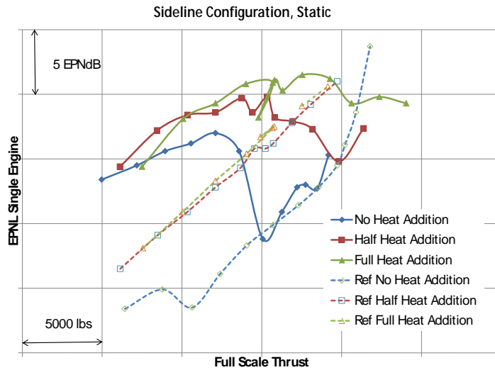
Figure 40 EPNL for Sideline Configuration, Static Conditions Processed to Sideline.
