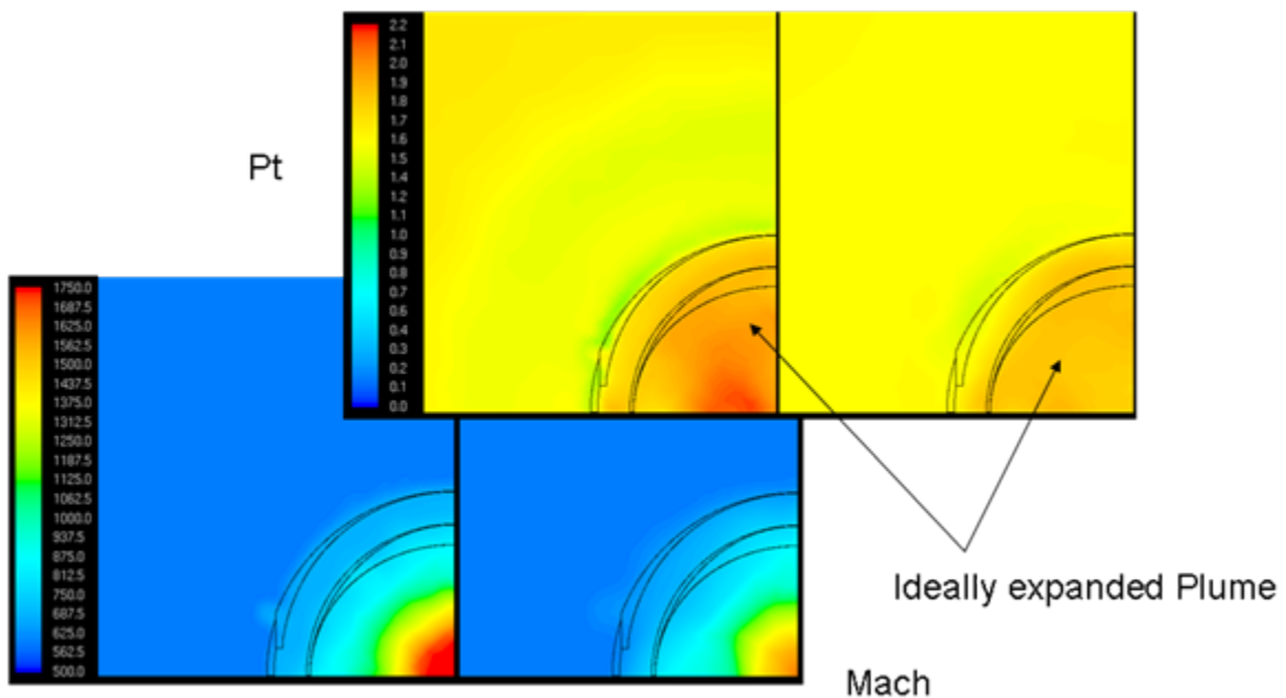
Cruise Mach and total pressure distributions in exit plume at L = 1D and 5D from nozzle exit, M = 1.6 , Alt = 50kft
