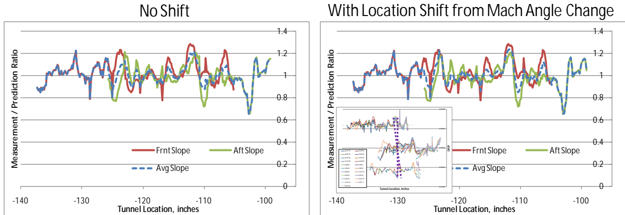
Figure 32. Offset Ratios Align Best with Model Induced Mach Angle Changes
