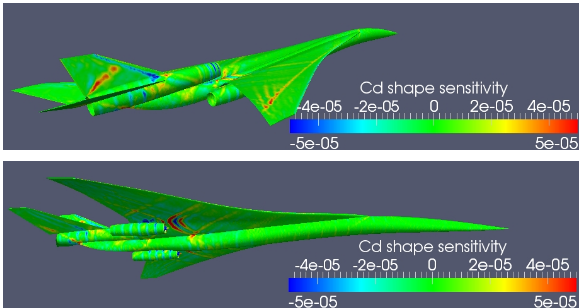
Figure 6. Shape sensitivity of the Drag coefficient (baseline configuration).
