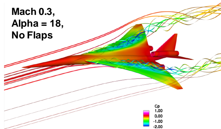
Figure 59. The wing vortex system maintains good quality airflow to the centerline nacelle even at high AOA
