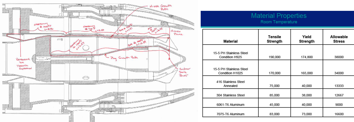
Figure 16 Structural materials and thermal growth
