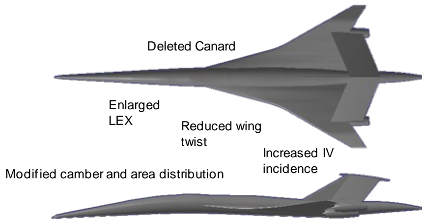
Figure 44. Modifications to the baseline N+2 improved the front signature significantly but were unable to prevent coalescence of the aft signature
