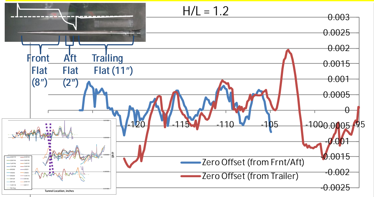
Figure 33. Zero Offsets from Front/Aft Flats and Trailer Match
