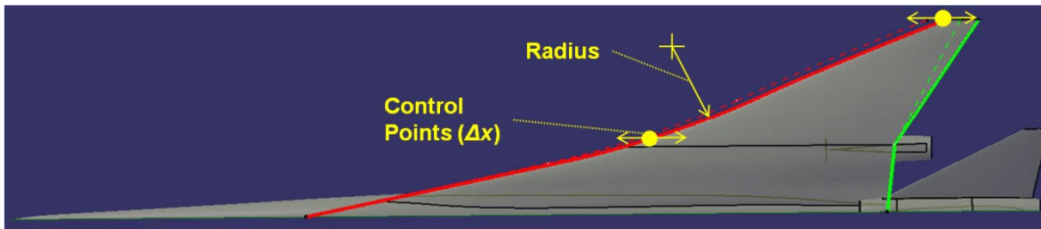
Figure 105. MDAO Planform Design Variables
