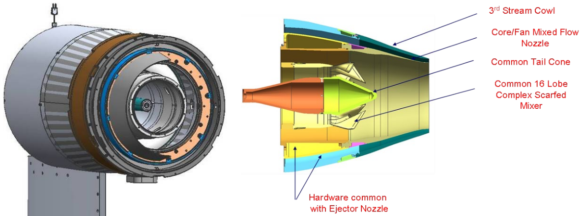
Figure 18 Modified HFJER (left) and N+2 Reference nozzle (right)
