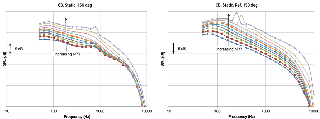
Figure 33 SPL at 150 deg for Cutback Configuration, Static Conditions, Processed to Flyover, No Heat Addition Cycle Conditions, Test Nozzle on Left, and Reference Nozzle on Right.
