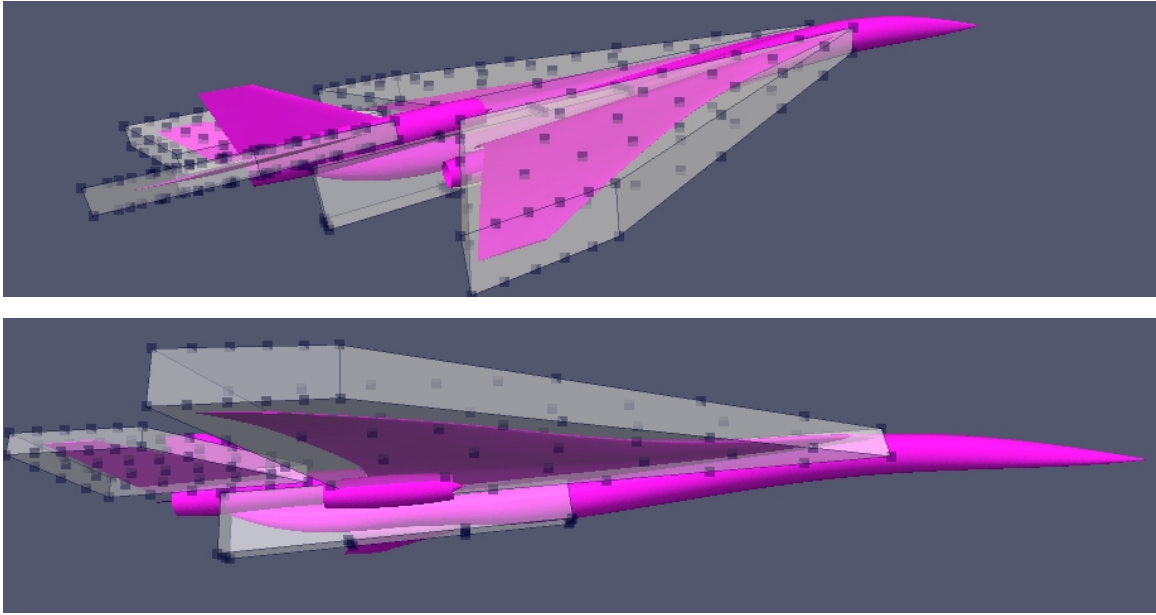
Figure 13. Free Form Deformation boxes used in the current optimization.
