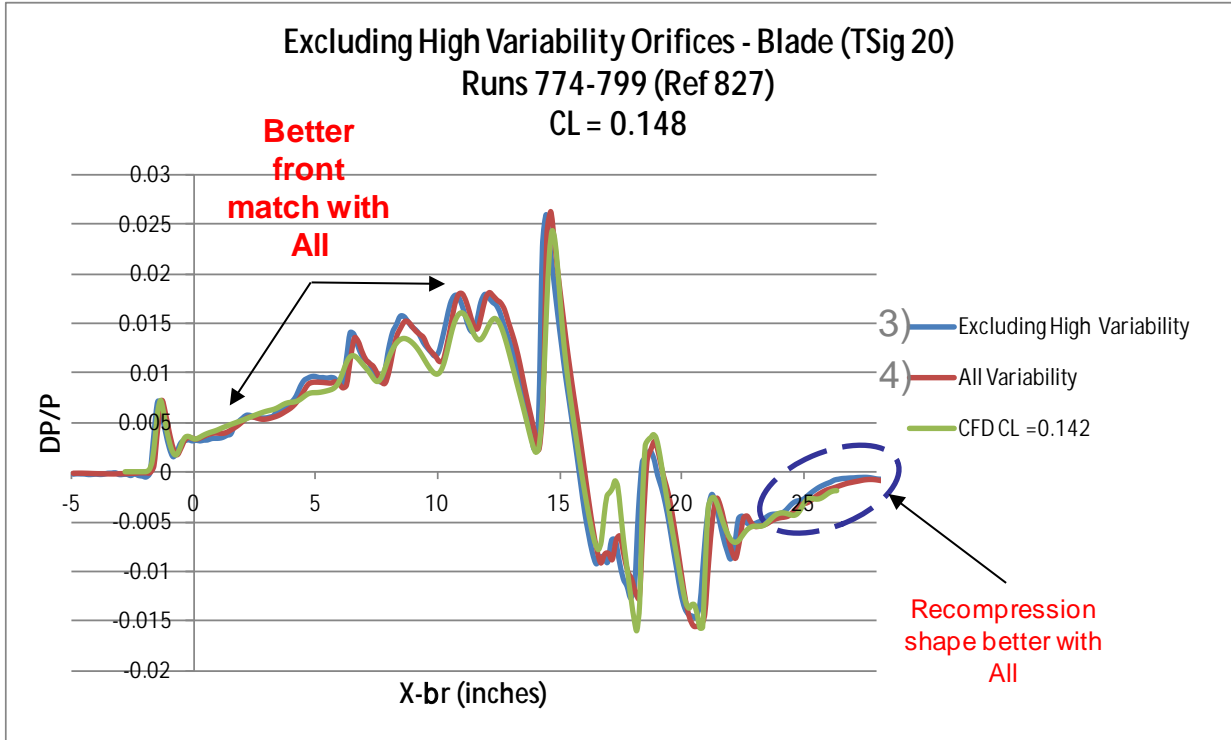
Figure 97. Averaging All Orifices (4) better than Excluding High Variability Orifices (3), and easier to process
