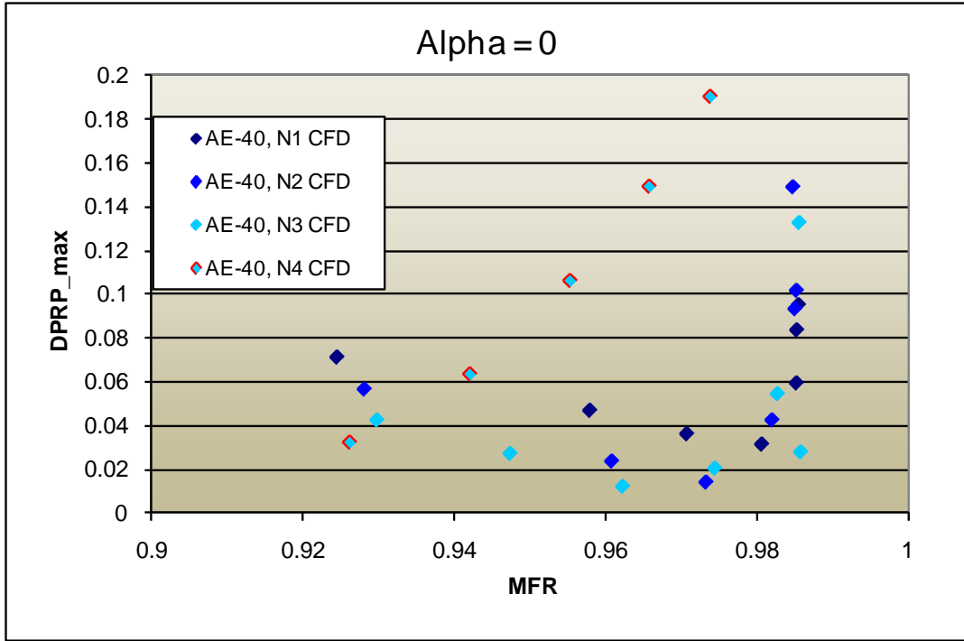
Figure 118. Diffuser-Shortening Effects on Engine Face Distortion
