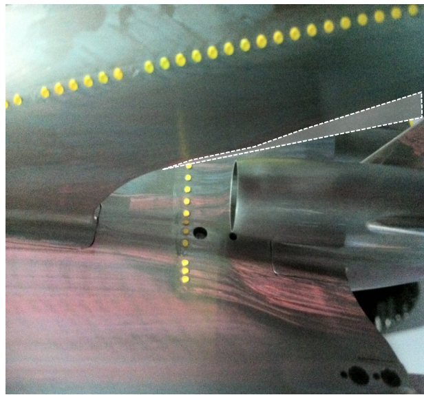
Figure 82. Blade Flow Separation Above Nacelle and Induced by Nacelle Shock
