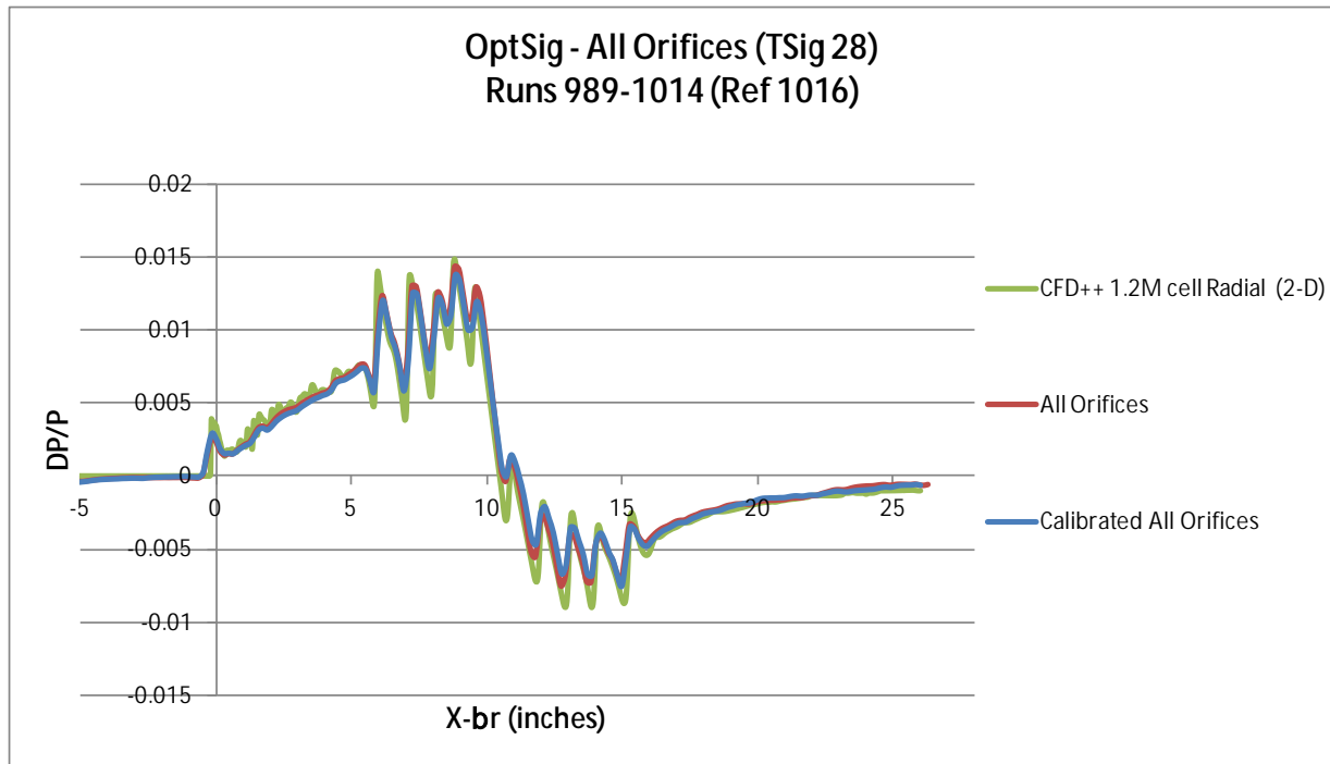
Figure 99. Calibration improves front shock match and recompression shape, but less initial aft expansion than Radial (2-D) CFD (like SEEB-ALR)
