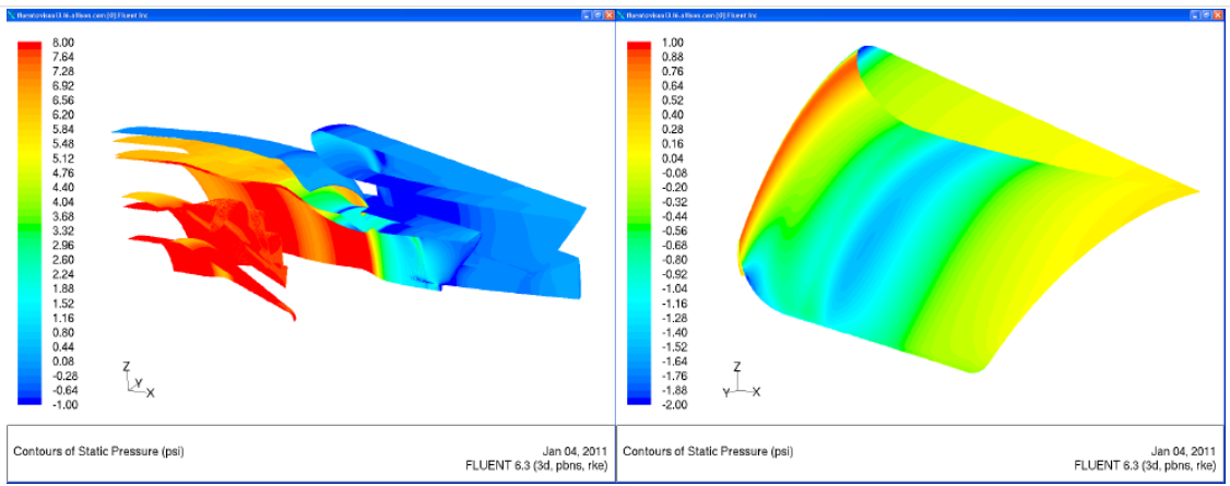
CFD based pressure loads were provided to ASE for conducting model design
