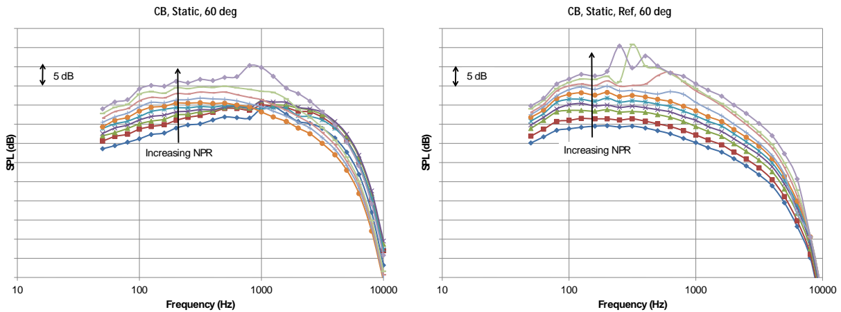
Figure 30 SPL at 60 deg for Cutback Configuration, Static Conditions, Processed to Flyover, No Heat Addition Cycle Conditions, Test Nozzle on Left, and Reference Nozzle on Right.
