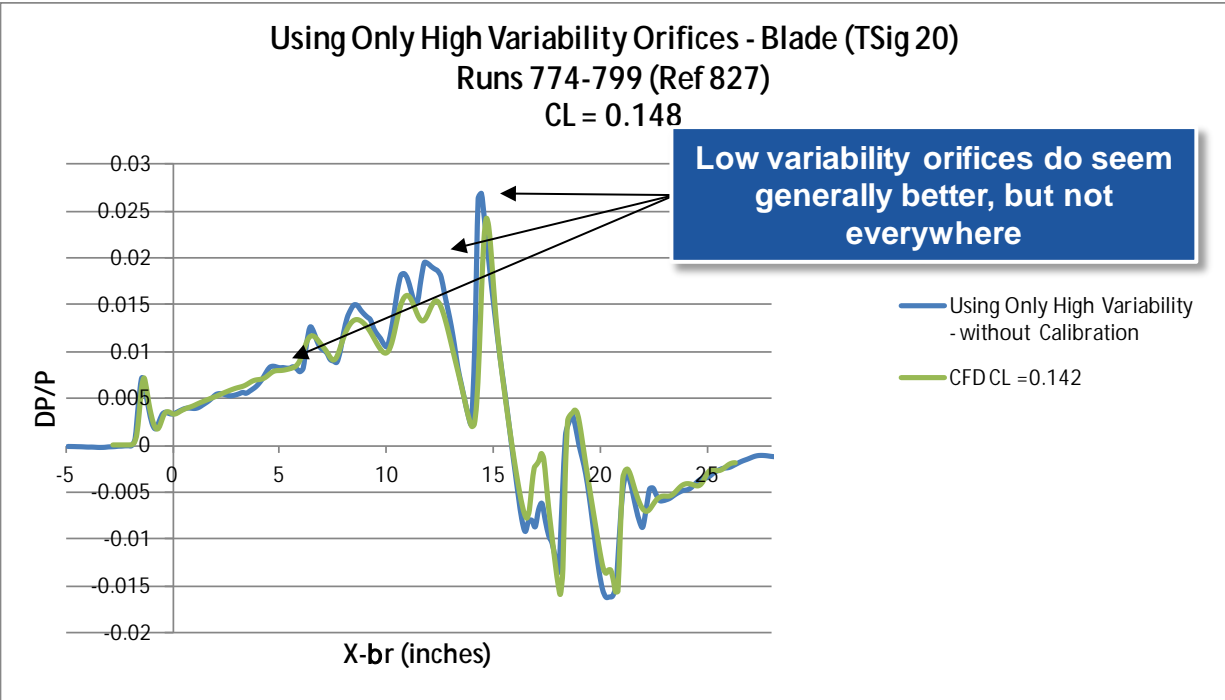
Figure 94. Low variability versus high variability orifices
