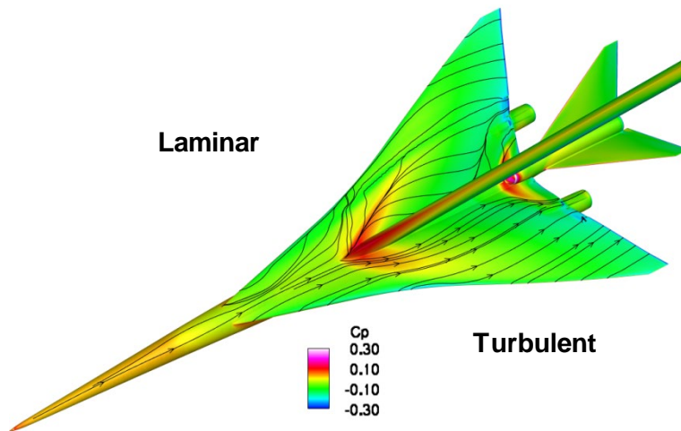
Figure 69. Viscous CFD results at model scale indicate that the blade mount may cause shock-induced separation on the upper surface of the wing if the boundary layer is laminar, suggesting it may be desirable to use grit to force transition on the upper surface during the test
