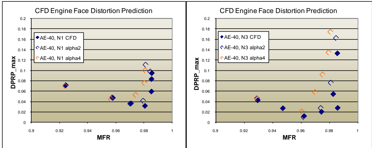
Figure 120. Angle-of-Attack Effects on Engine Face Distortion
