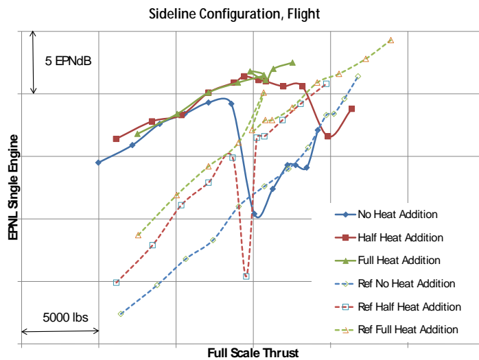
Figure 41 EPNL for Sideline Configuration, Flight Conditions Processed to Sideline.
