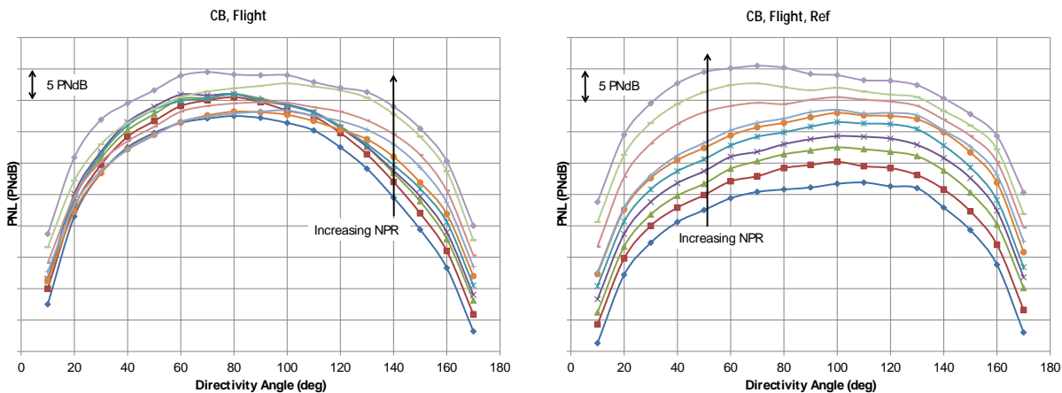
Figure 34 PNL for Cutback Configuration, Flight Conditions, Processed to Flyover, No Heat Addition Cycle Conditions, Test Nozzle on Left, and Reference Nozzle on Right.
