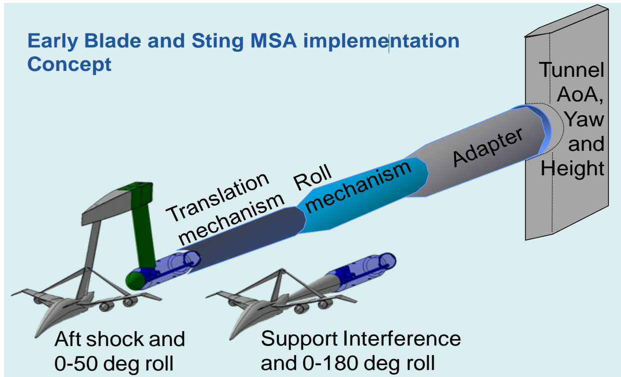
Figure 4. Keeping the Model in the Same Position with Sting and Blade was Deemed Unnecessary, Simplifying the Final Design
