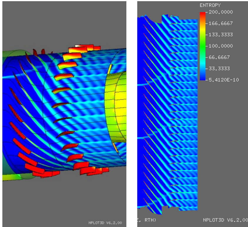
Figure 60 Progression of the inlet distortion through the fan and OGVs.
