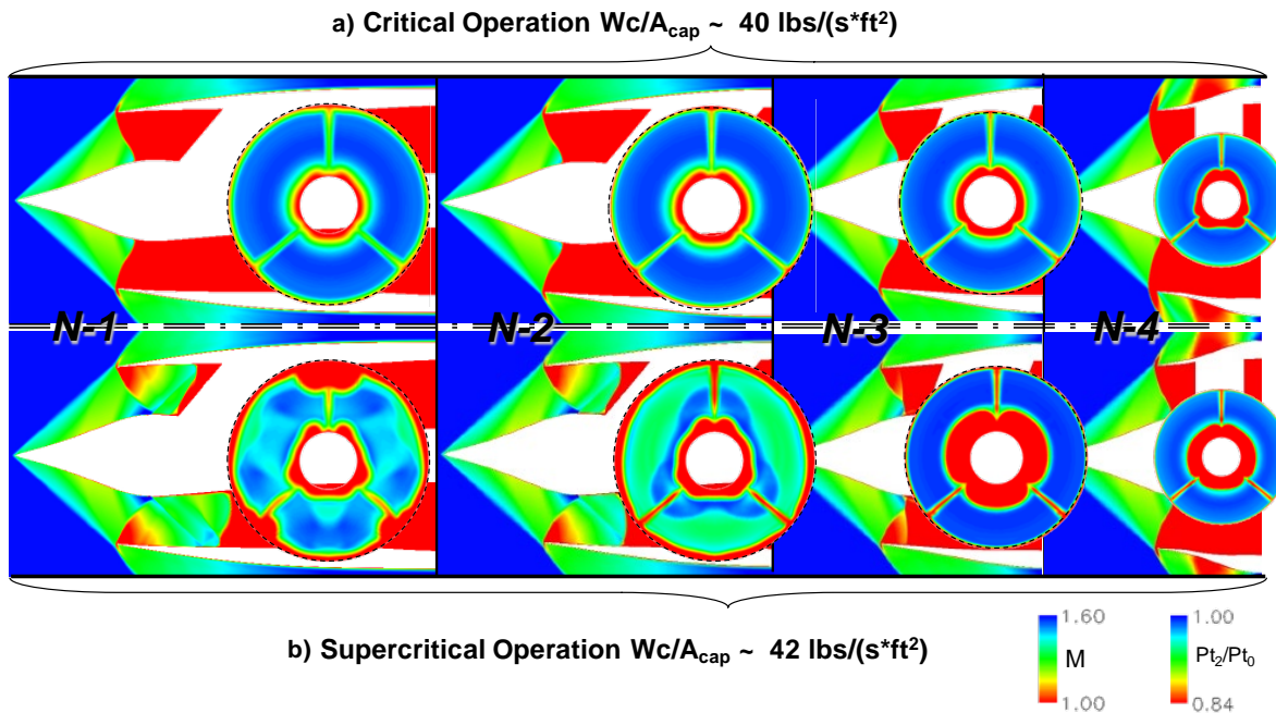
Figure 116. Symmetry Plane Mach Contours and Engine Face Recovery Contours Comparing Diffuser Length at Critical and Supercritical Operation
