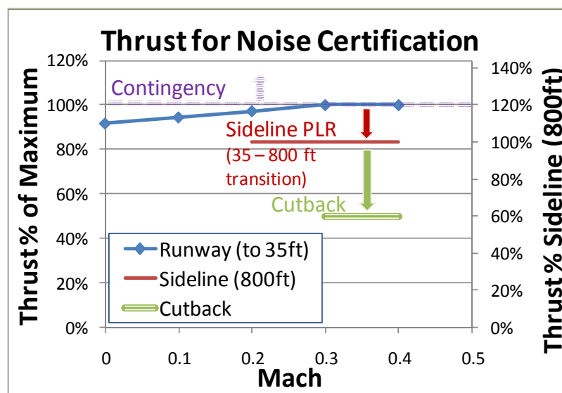
Figure 128. Engine Designed for Noise Compliance with Best Performance
