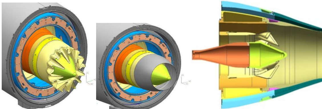
Figure 21 Reference Nozzles: PRFN (mixer Core), and SPFN (splitter core) – both nozzles have same external annular cowls (shown on right)
