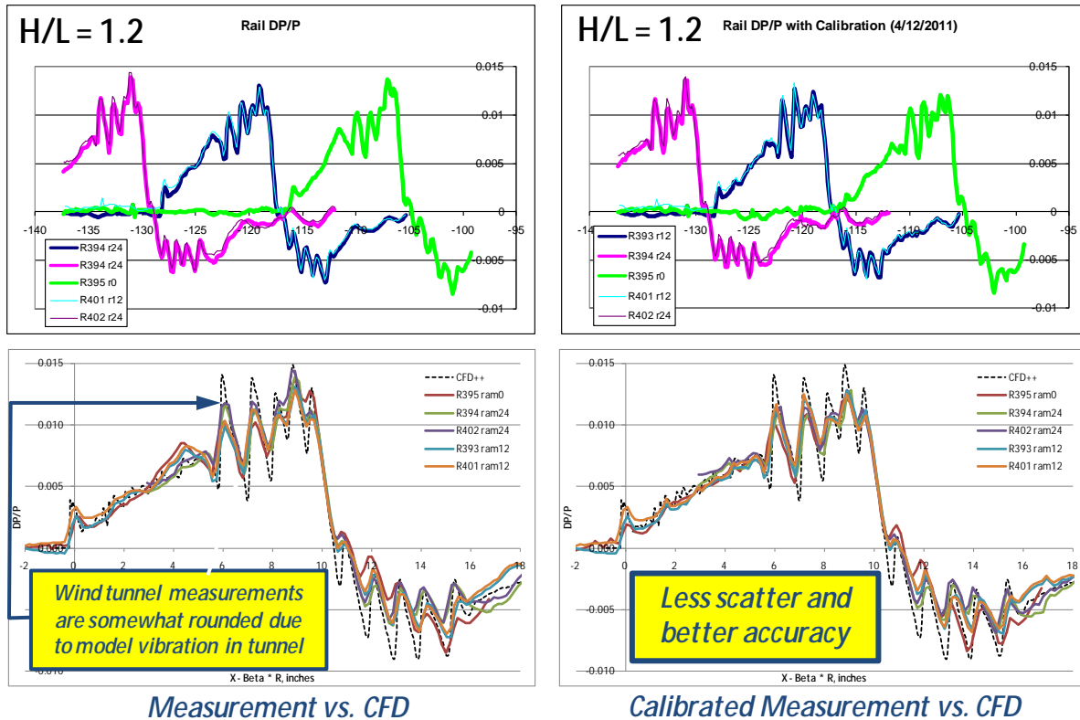
Figure 35. Slope and Zero Correction Improves OptSig Measurements
