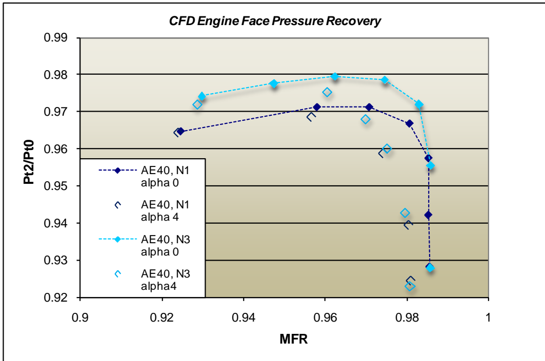
Figure 119. Angle-of-Attack Effects on Engine Face Recovery
