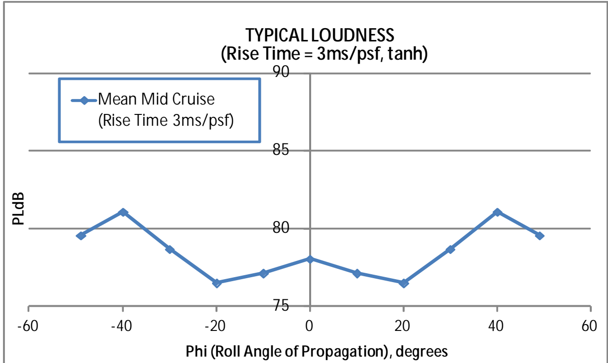
Figure 58. Using methodology matching typically measured rise time and using an averaged operational weight, the above trend intends to portray the average typical vehicle loudness versus roll angle
