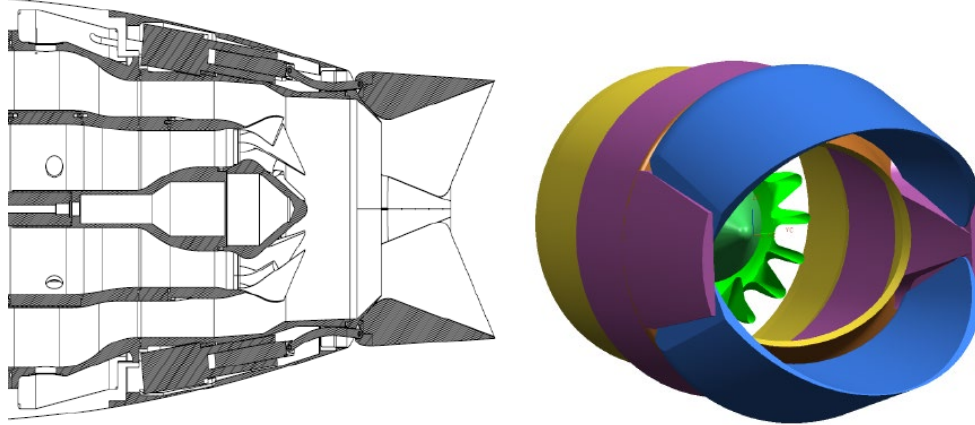
Figure 7 HVC10 Mixer-Ejector Nozzle Design
