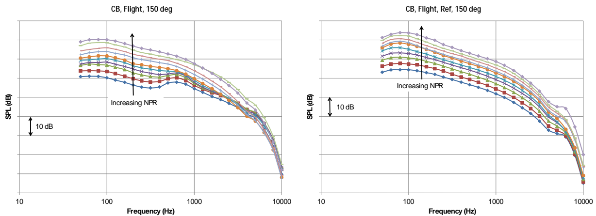
Figure 39 SPL at 150 deg for Cutback Configuration, Flight Conditions, Processed to Flyover, No Heat Addition Cycle Conditions, Test Nozzle on Left, and Reference Nozzle on Right.
