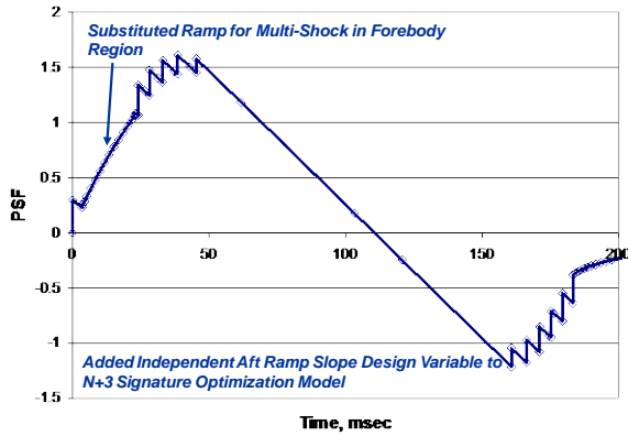
Figure 19. (1) Optimized Ground Target
