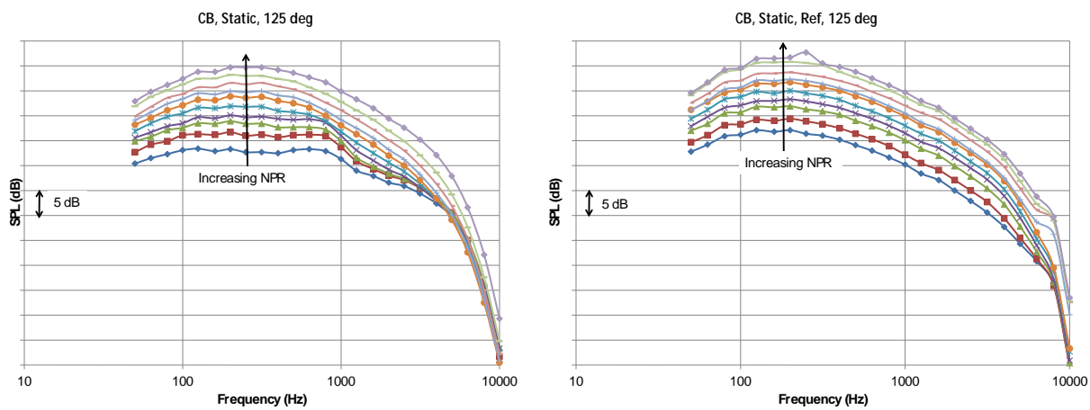
Figure 32 SPL at 125 deg for Cutback Configuration, Static Conditions, Processed to Flyover, No Heat Addition Cycle Conditions, Test Nozzle on Left, and Reference Nozzle on Right.
