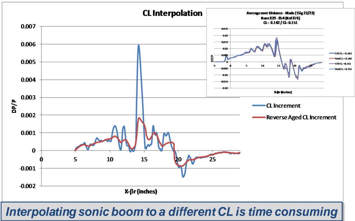
Figure 89. CL increment initially coalesced at each shock into spikes
