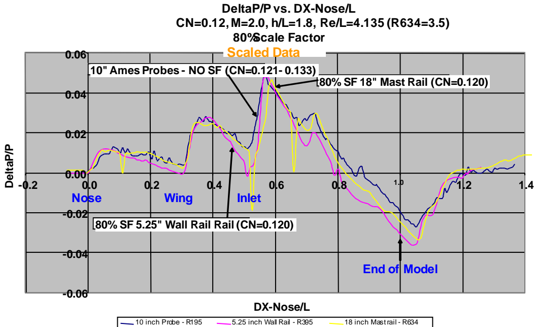
Figure 11. x1.6 Reflection at CL = 0.12 Not Matching
