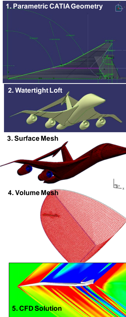
Figure 41. Associativity between parametric CAD and CFD models enables rapid generation and evaluation of low boom design concepts
