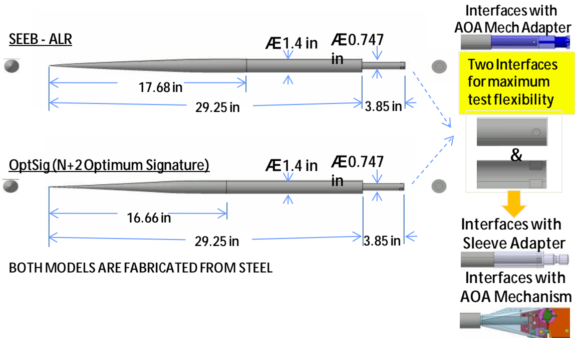
Figure 26. Axi-Symmetric “Javelin” Models’ Geometry
