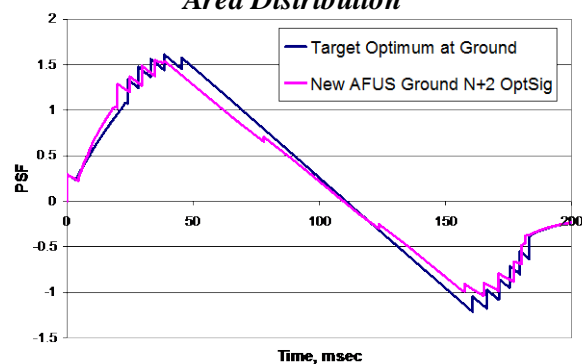
Figure 24. (6) Final Ground N+2 OptSig
