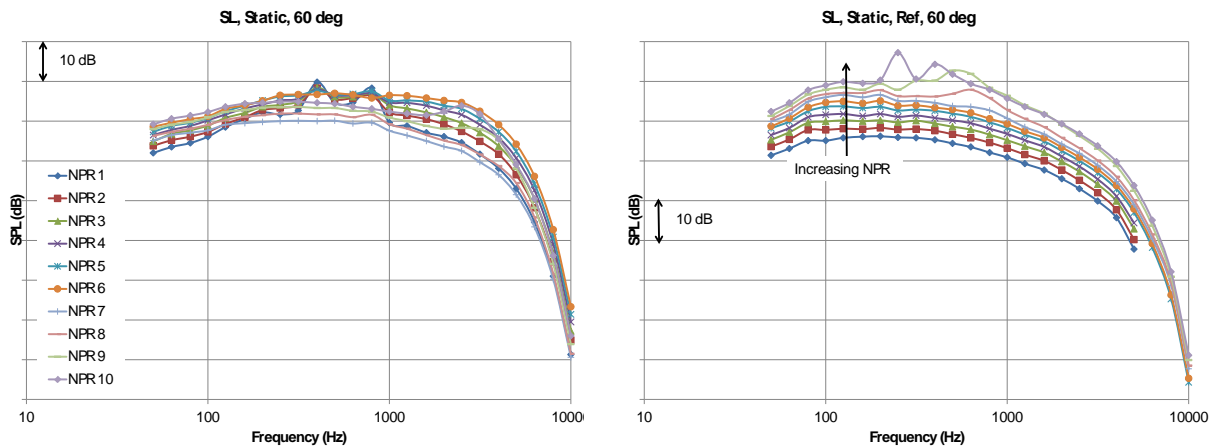
Figure 43 SPL at 60 deg for Sideline Configuration, Static Conditions, Processed to Sideline, No Heat Addition Cycle Conditions, Test Nozzle on Left, and Reference Nozzle on Right.
