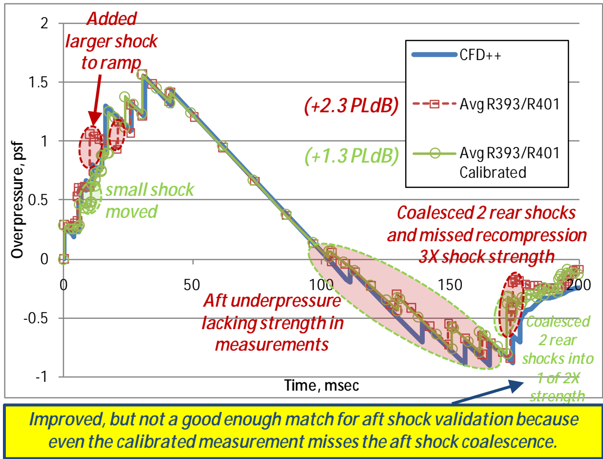
Figure 36. OptSig Propagation to the Ground
