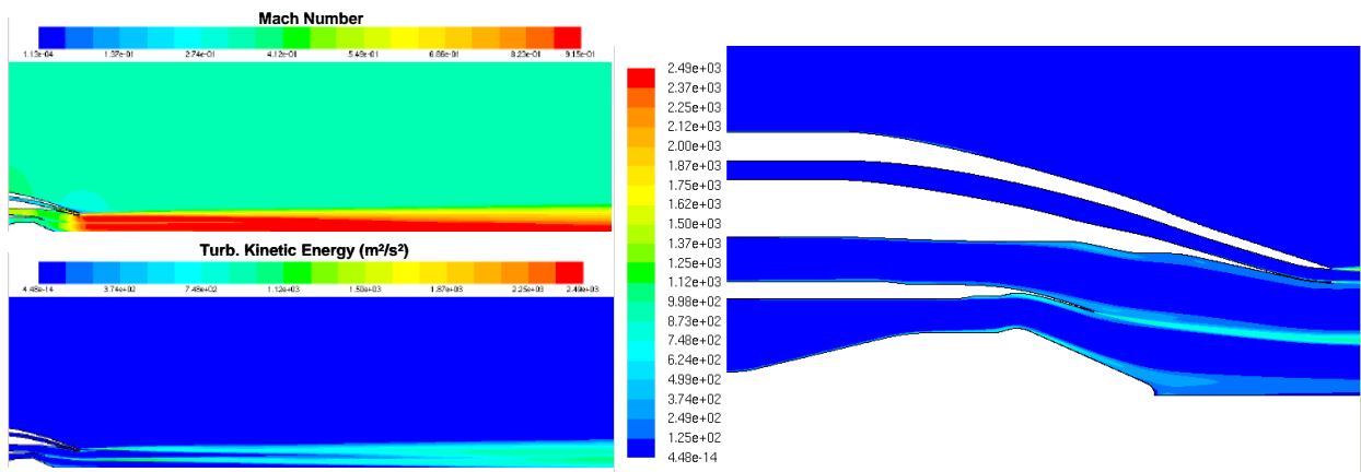
Figure 14 Reference nozzle plume Mach numbers (Max = 0.91) and Turbulence kinetic energy tke (Max= 800m 2 /s 2 ), TO, 0.3M
