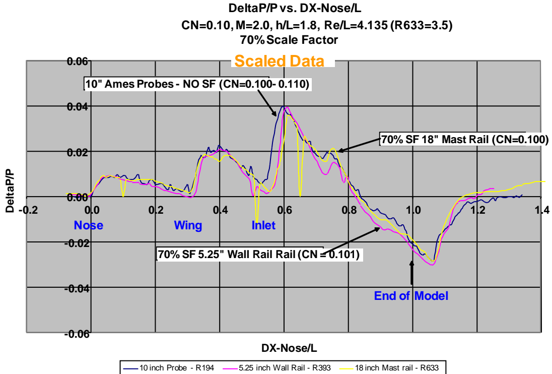
Figure 10. x1.4 Reflection at CL = 0.10 Mostly Matches
