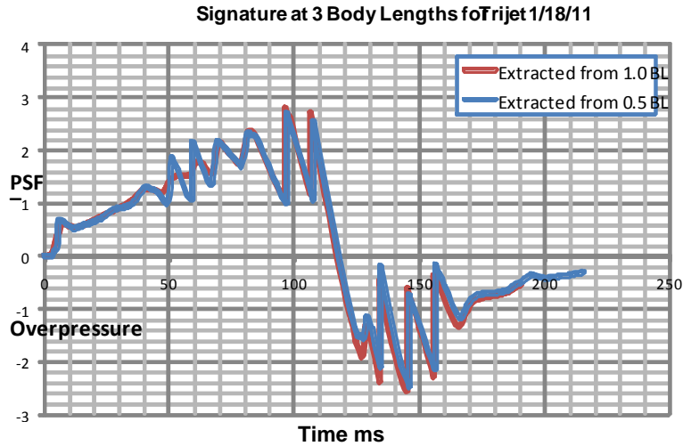
Figure 49. Use of the near-field cylinder correction method permits extrapolation of signatures from CFD solutions at only 0.5-1 body lengths, significantly reducing computational burden
