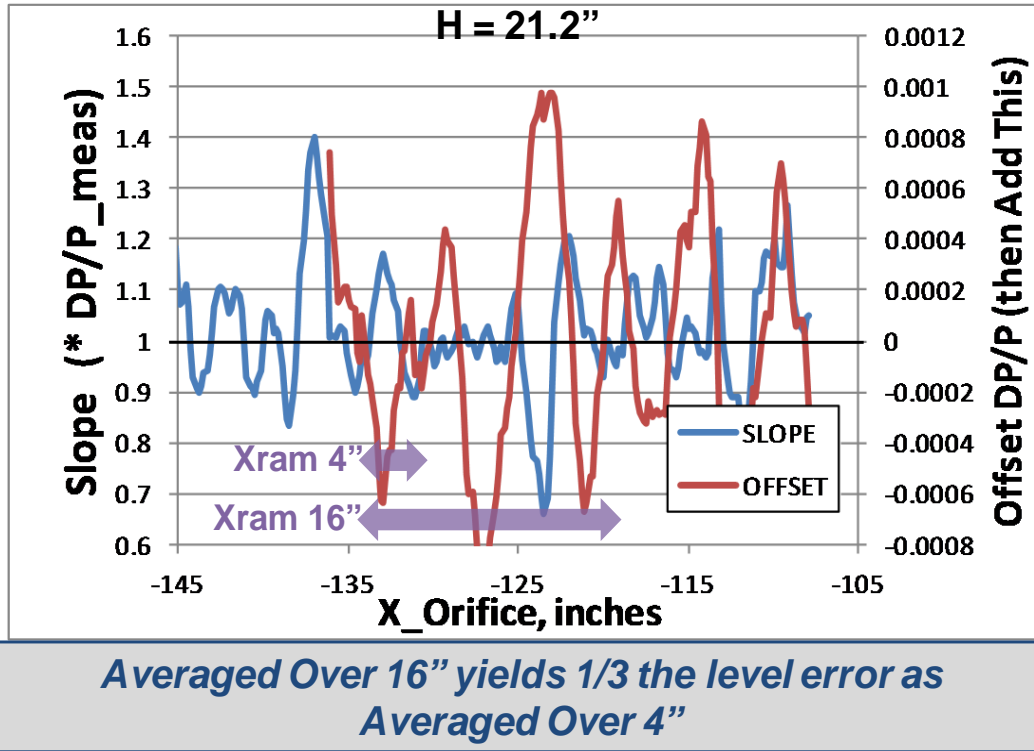
Figure 87. Slope and zero (offset) correction for each orifice based on SEEB-ALR measurements
