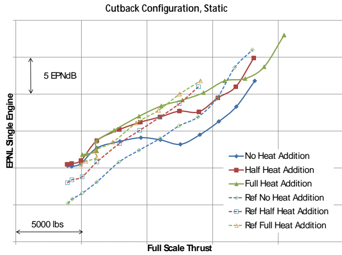
Figure 27 EPNL for Cutback Configuration, Static Conditions Processed to Flyover.
