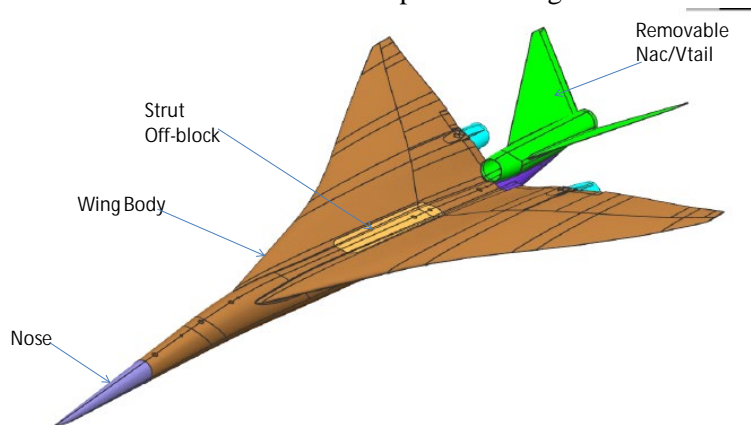
Figure 65. The 0.008 scale wind tunnel model of the QR4 configuration has removable nacelles and a two position tail to capture important sonic boom increments
