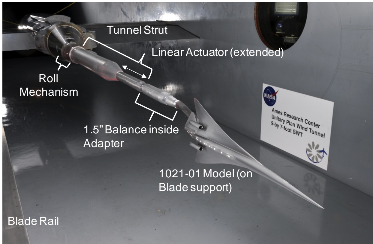
Figure 78. 1021-01 Model (on blade), balance and actuation equipment
