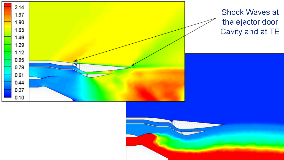
Cruise Mach and total temperature distributions, M = 1.6 , Alt = 50,000 ft
