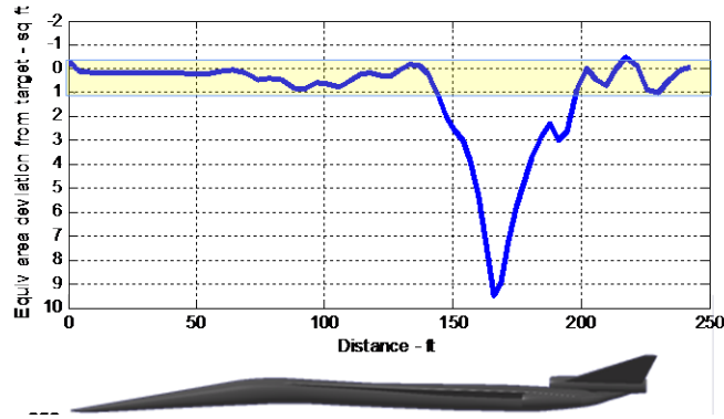
Figure 48. The response surface method was used to match the undertrack to within \pm 1 sq ft
