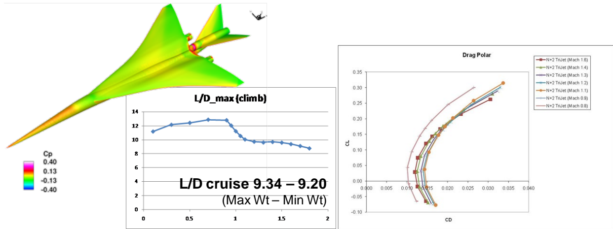
Figure 60. The QR4 1021-01 (N+2) Trijet design simultaneously achieves low sonic boom and good supersonic L/D due to careful attention to wave drag reduction during the low boom design process
