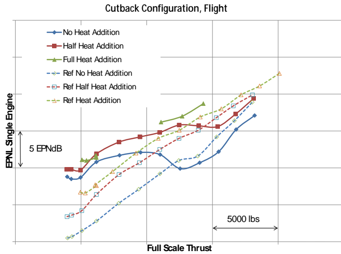
Figure 28 EPNL for Cutback Configuration, Flight Conditions Processed to Flyover.
