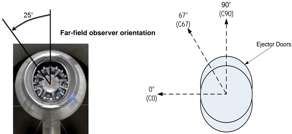
Figure 19 Far-field observer orientations: clocking positions for Ejector nozzle tests (ESCORT configuration names – C67, C90, C0).
