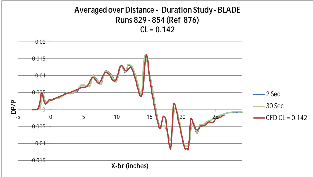
Figure 101. Insignificant variation between the 2 and 30 sec sampling when Averaging 26 Over Distance
