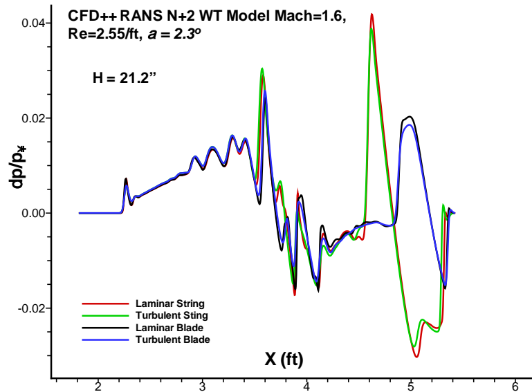
Figure 83. Signature Difference Between Laminar and Turbulent
