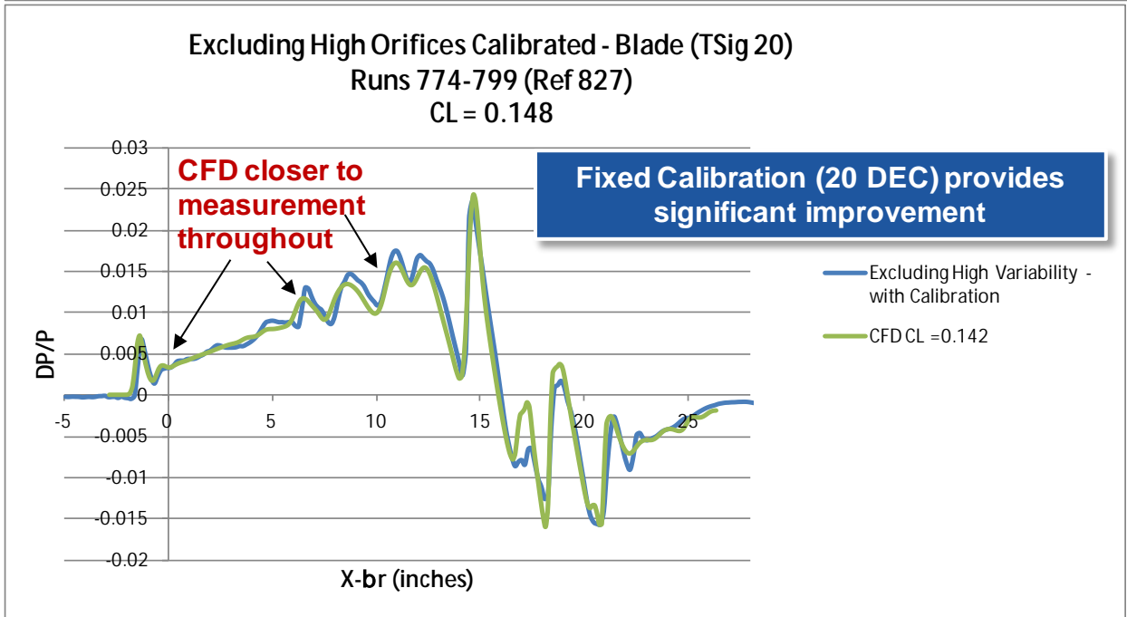
Figure 95. Calibration provides significant improvement
