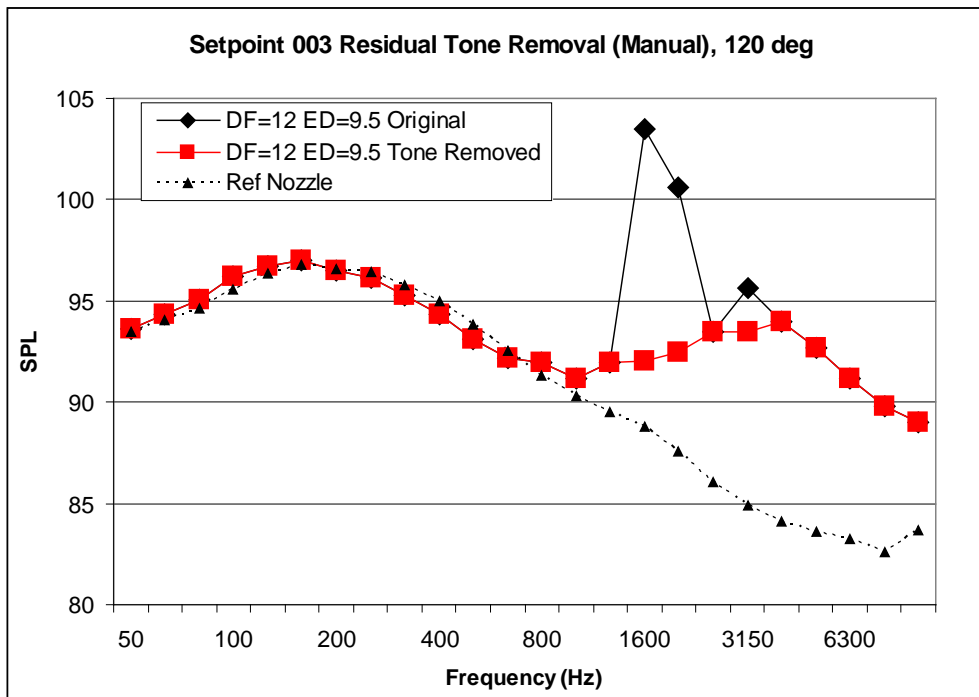
Figure 30 Source noise level comparisons with and without tonal contribution, example at 120 deg polar emission angle
