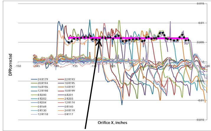
Figure 28. Variations of +/- 20% of Flat-Top Pressure Repeated at the Same Rail Position Despite Different Model Position
