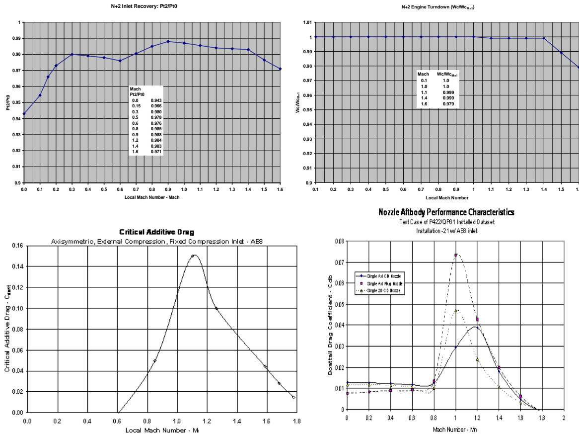
Figure 2 Inlet and Nozzle After-body Drag Characteristic Requirements
