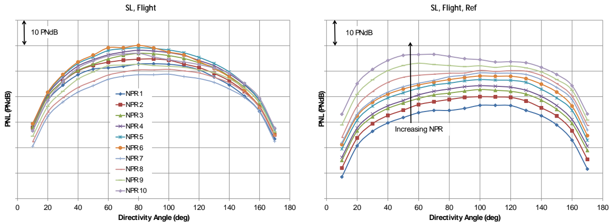
Figure 47 PNL for Sideline Configuration, Flight Conditions, Processed to Sideline, No Heat Addition Cycle Conditions, Test Nozzle on Left, and Reference Nozzle on Right.
