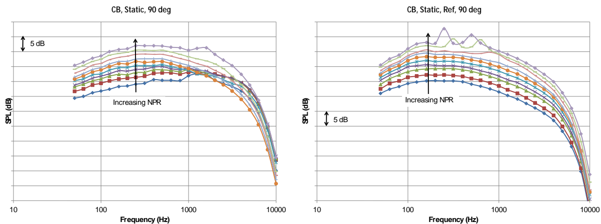
Figure 31 SPL at 90 deg for Cutback Configuration, Static Conditions, Processed to Flyover, No Heat Addition Cycle Conditions, Test Nozzle on Left, and Reference Nozzle on Right.
