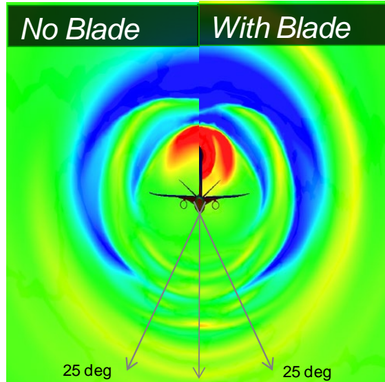
Figure 70. The highly swept blade support has a minimal impact on the measured pressure signature from directly undertrack to approximately 25 degrees off-track
