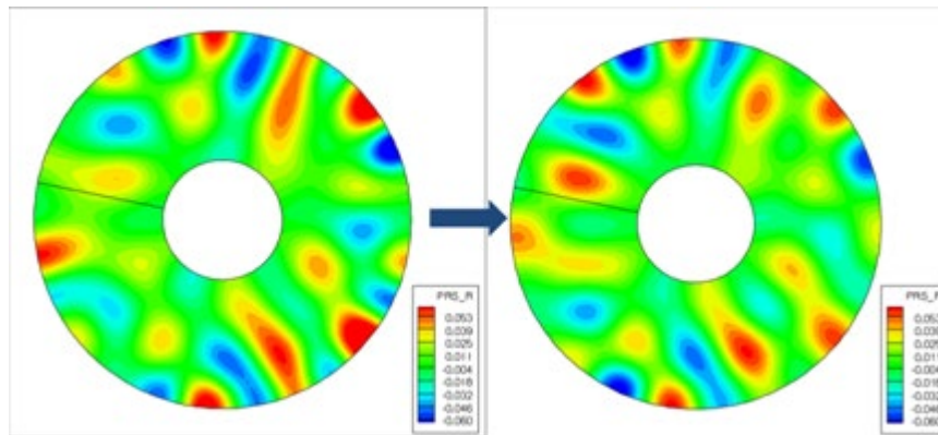
Figure 64 Schematic showing a harmonic perturbation field (full field on left) and radiating part only on right.
