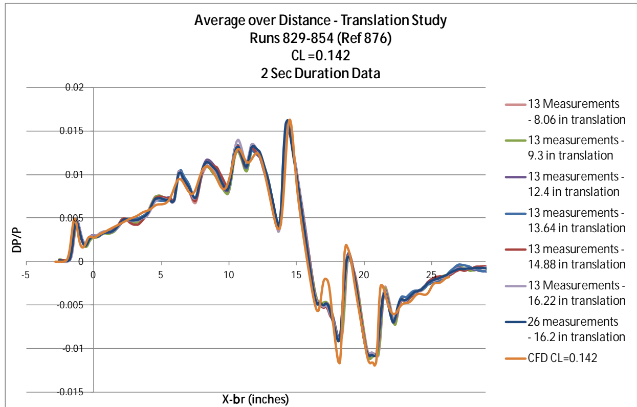
Figure 103. It is not definitively clear the minimum length of translation required to achieve sufficient accuracy
