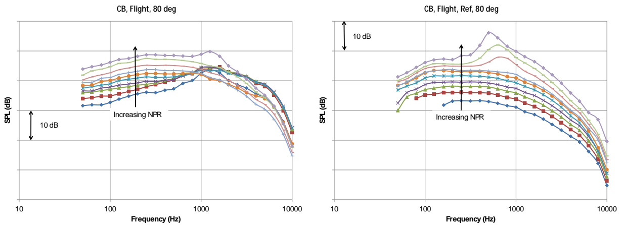
Figure 36 SPL at 80 deg for Cutback Configuration, Flight Conditions, Processed to Flyover, No Heat Addition Cycle Conditions, Test Nozzle on Left, and Reference Nozzle on Right.
