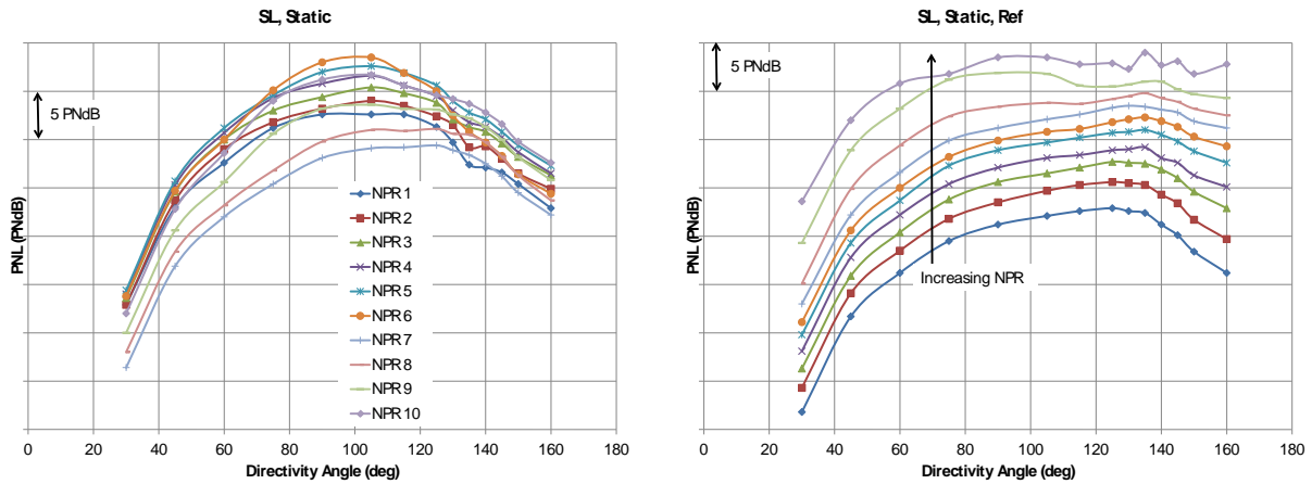
Figure 42 PNL for Sideline Configuration, Static Conditions, Processed to Sideline, No heat addition Cycle Conditions, Test Nozzle on Left, and Reference Nozzle on Right.
