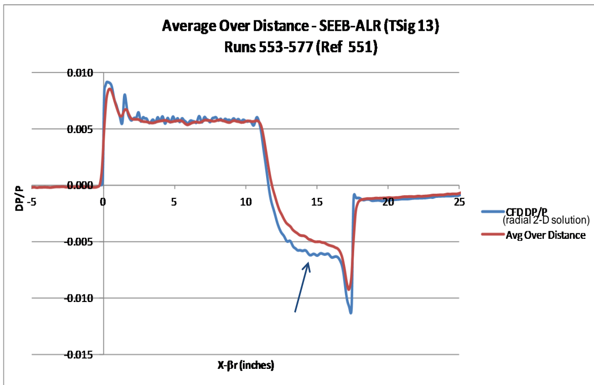
Figure 90. Great front signature match but aft level mismatch with CFD was unexpected
