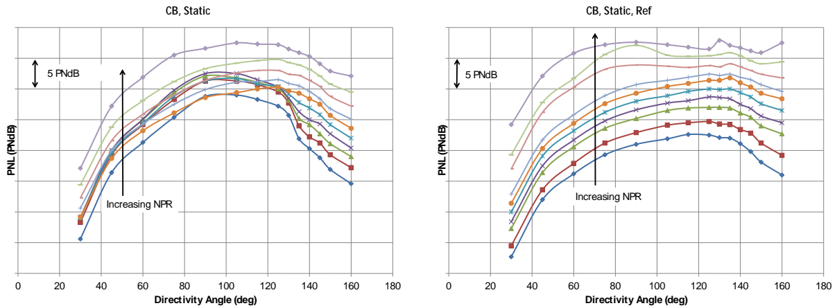
Figure 29 PNL for Cutback Configuration, Static Conditions, Processed to Flyover, No Heat Addition Cycle Conditions, Test Nozzle on Left, and Reference Nozzle on Right.
