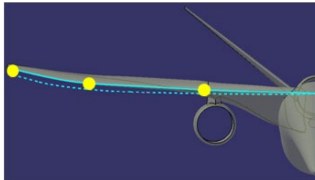
Figure 104. MDAO Wing Twist Design Variables
