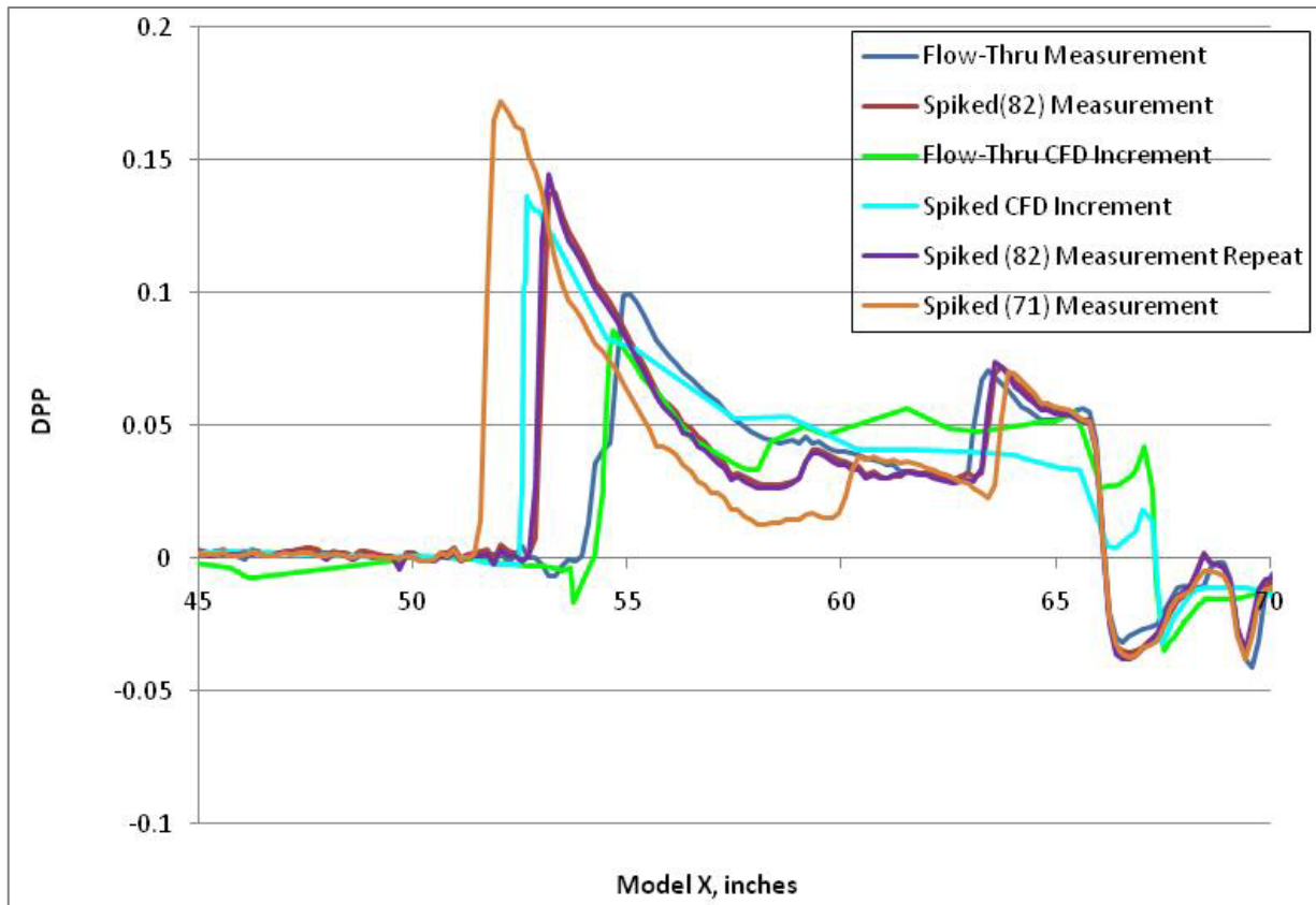
Figure 39. CFD and Test increments
