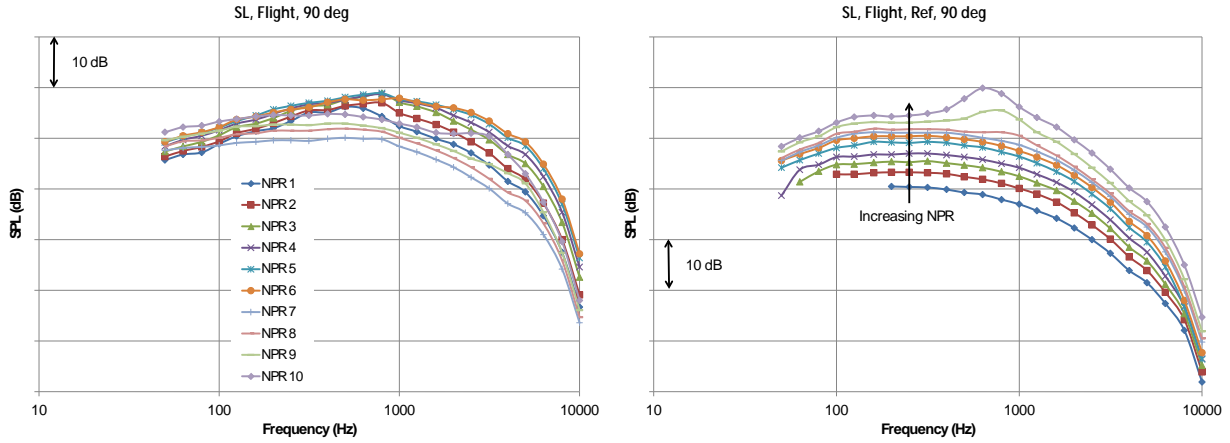
Figure 50 SPL at 90 deg for Sideline Configuration, Flight Conditions, Processed to Sideline, No Heat Addition Cycle Conditions, Test Nozzle on Left, and Reference Nozzle on Right.
