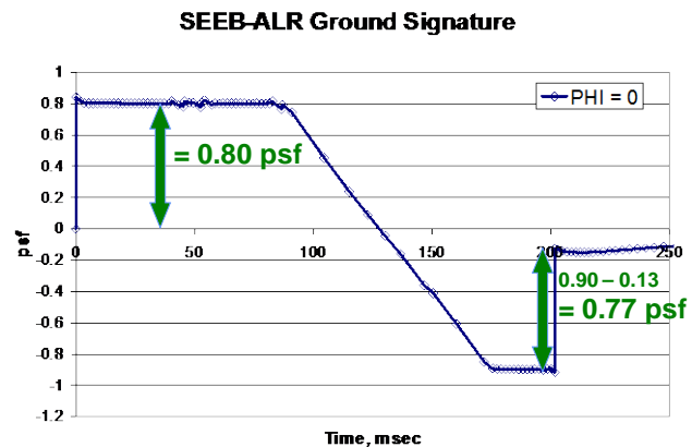
Figure 17. SEEB-ALR Design also Provides Flat-Top Pressure Validation
