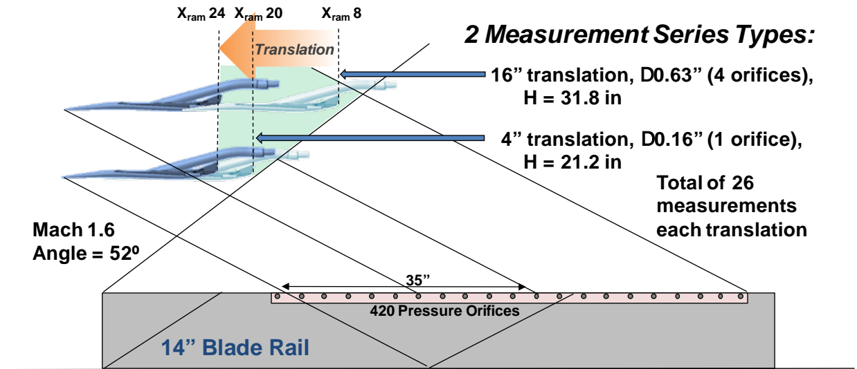
Figure 77. New procedures for 2 types of sonic boom measurement
