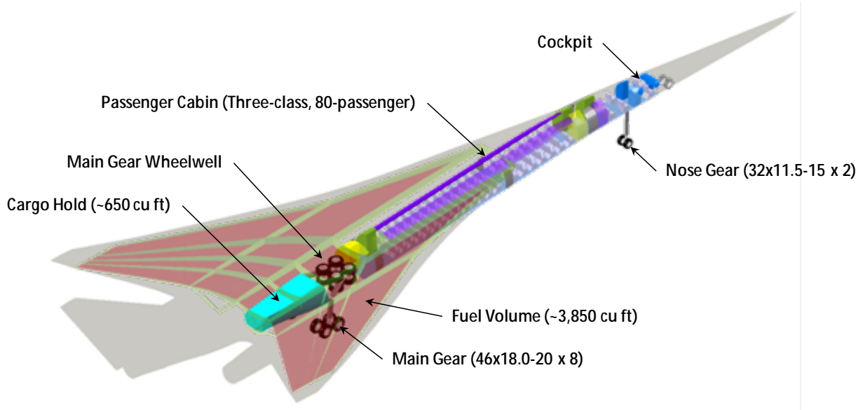
Figure 61. LM N+Notional vehicle layout
