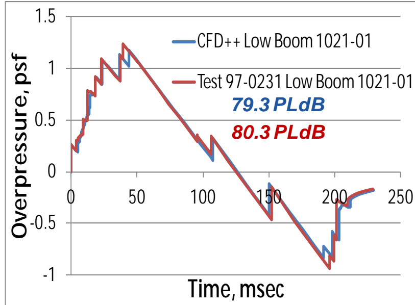
Figure 100. Matching measurement produces matching ground propagation within 1 PLdB of prediction
