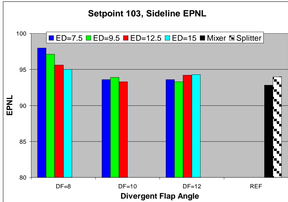
Figure 27 Effect of mixer-ejector configuration on EPNL and comparisons to reference nozzle
