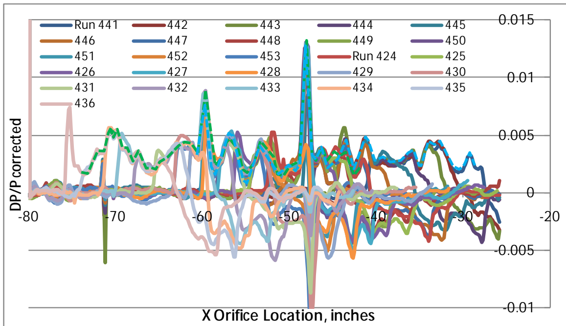
Figure 29. Distortion Pattern Overlays from Different Measurement Distances
