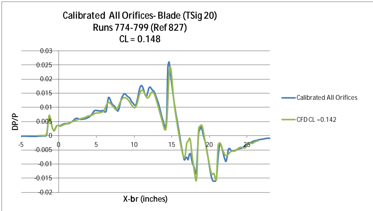
Figure 98. Calibrated (if available) All Orifices best process for signatures
