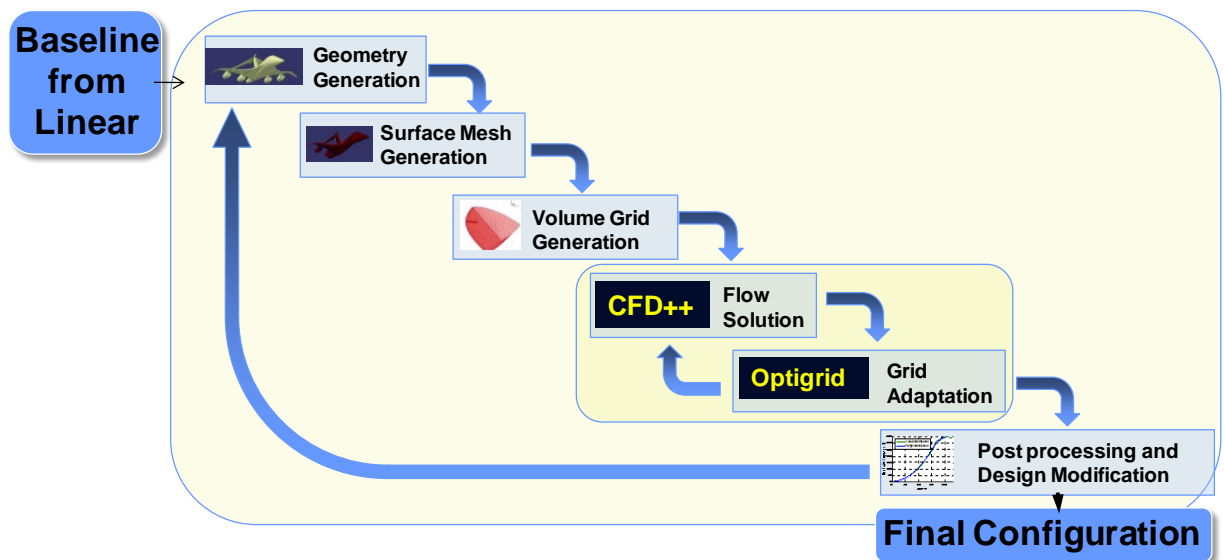
Figure 40. N+2 design tools enabled rapid iteration of low boom concepts
