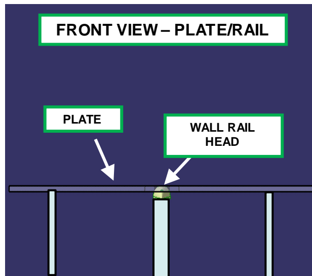
Figure 14. Plate Measurement Off-Set from Wall Concept
