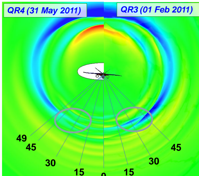
Figure 55. Design refinements between QR3 and QR4 significantly reduced the magnitude of the expansion spike and resulted in a shaped signature to almost 40 degrees off-track
