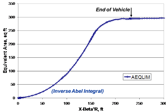
Figure 21. (3) Integrate Target Equivalent Area
