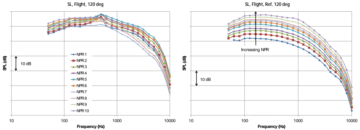
Figure 51 SPL at 120 deg for Sideline Configuration, Flight Conditions, Processed to Sideline, No Heat Addition Cycle Conditions, Test Nozzle on Left, and Reference Nozzle on Right.
