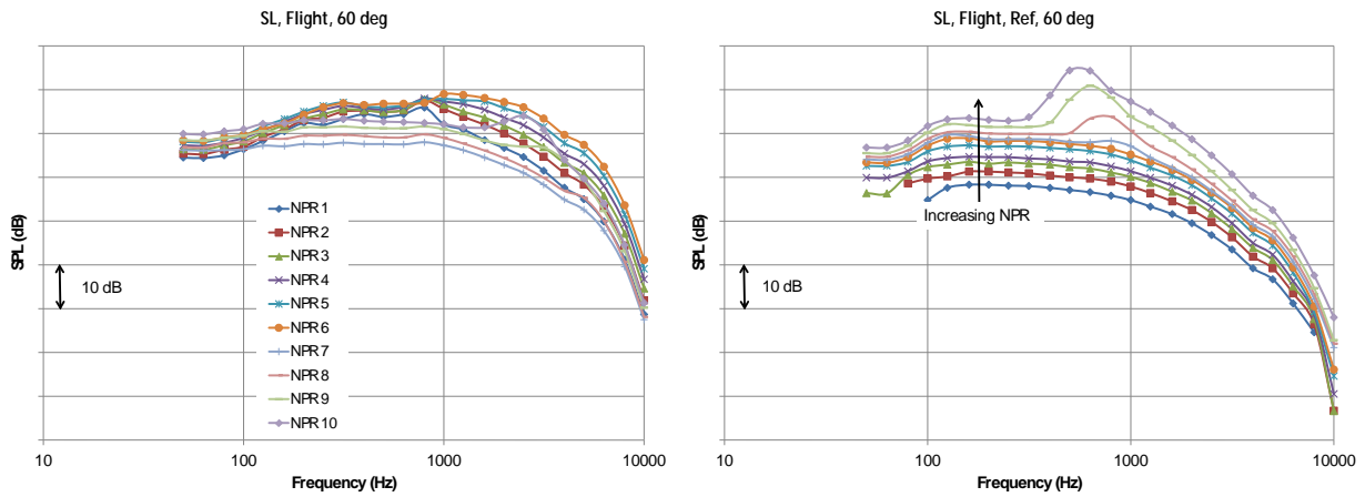
Figure 48 SPL at 60 deg for Sideline Configuration, Flight Conditions, Processed to Sideline, No Heat Addition Cycle Conditions, Test Nozzle on Left, and Reference Nozzle on Right.
