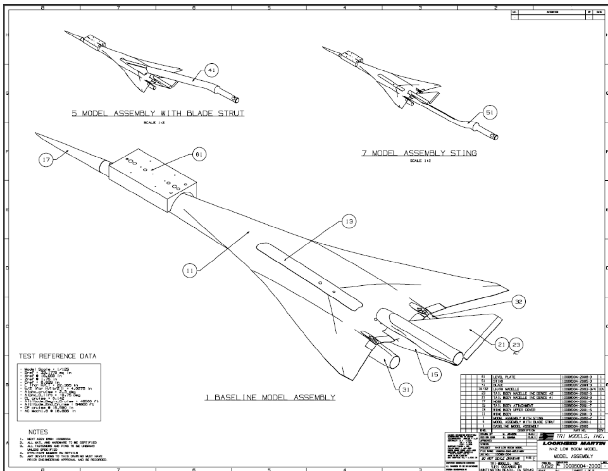
Figure 73. Assembly drawings of the LM N+2 Low Boom Model and support hardware
