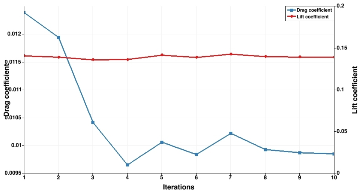
Figure 18. Detail of the shape design optimization (min Cd, Cl=0.14), and evolution of the optimization (right)
