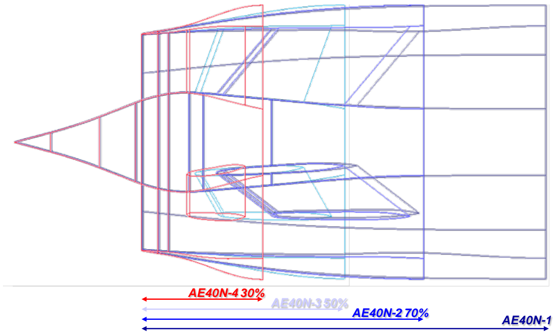
Figure 115. Side View of Inlets Used in Diffuser Length Study
