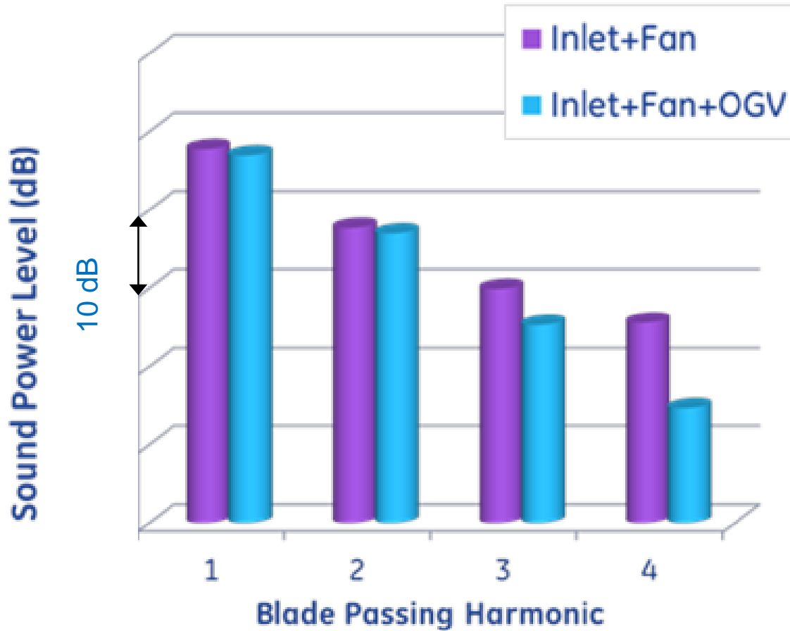
Figure 65 Sound power level at an axial plane just in front of the fan due to the inlet distortion-fan interaction and the combined inlet distortion-fan-OGV interaction.
