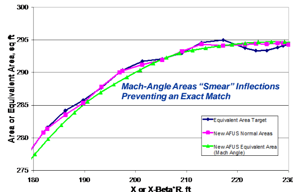
Figure 22. (4) Match Mach-Angle Area with Normal Area Distribution
