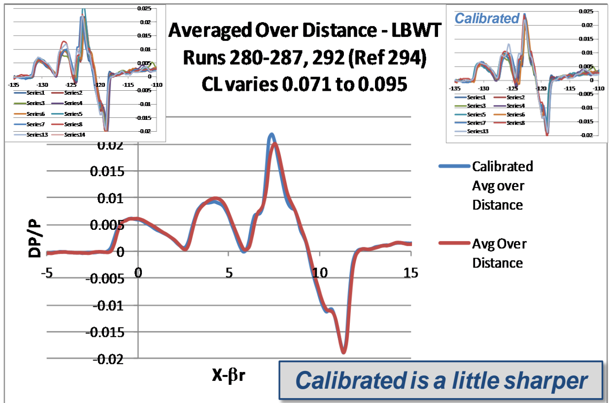
Figure 92. Technique applied to LM1 with only 9 measurements and large CL variation
