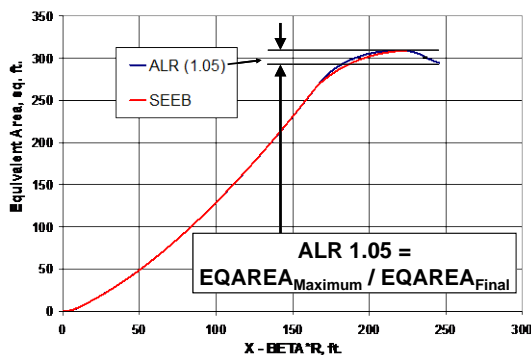
Figure 16. More Practical SEEB-ALR Target with 5% Area Drop at Aft End
