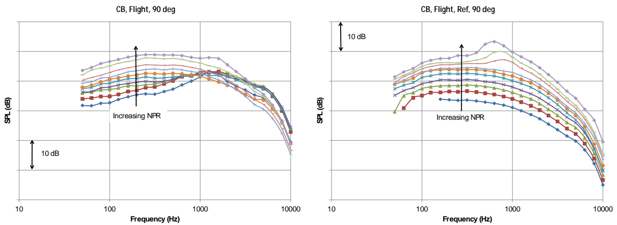
Figure 37 SPL at 90 deg for Cutback Configuration, Flight Conditions, Processed to Flyover, No Heat Addition Cycle Conditions, Test Nozzle on Left, and Reference Nozzle on Right.
