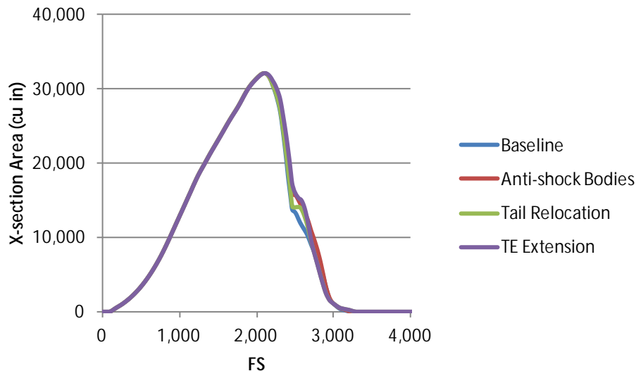
Figure 54. Area distribution comparison
