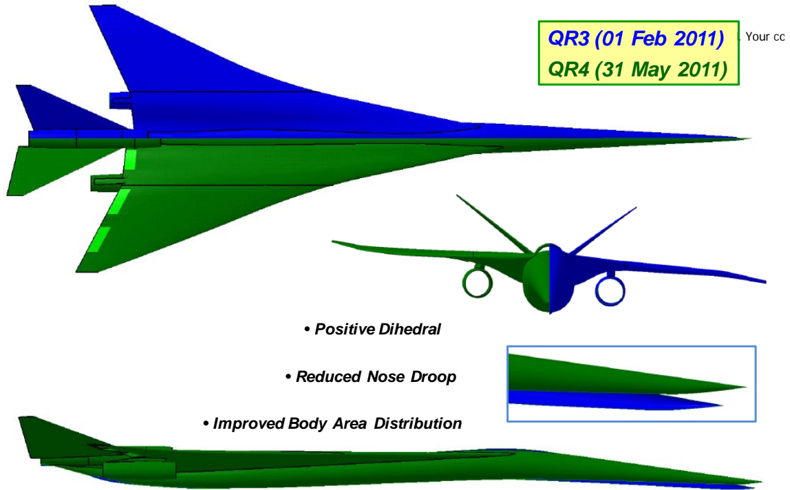
Figure 51. The design of the trijet N+2 configuration was significantly modified between QR3 and QR4 to improve off track loudness while retaining good under-track performance
