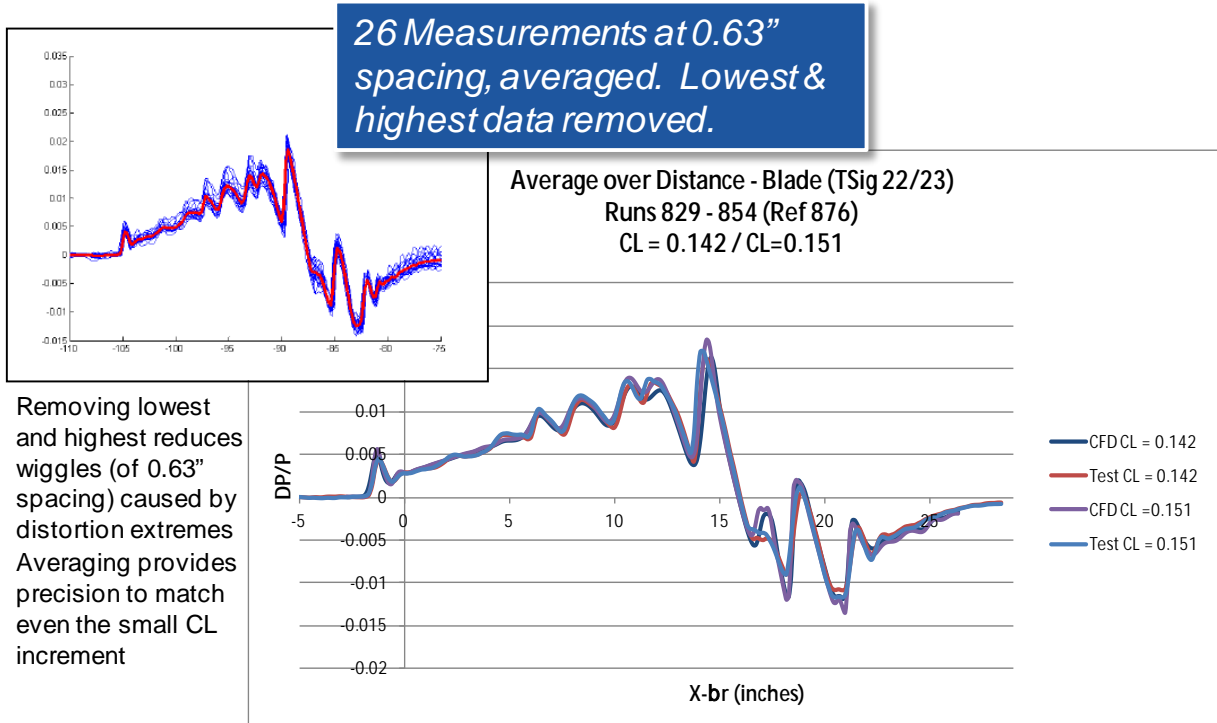
Figure 88. Pre-Test CFD Matches Measurement with Remarkable Precision
