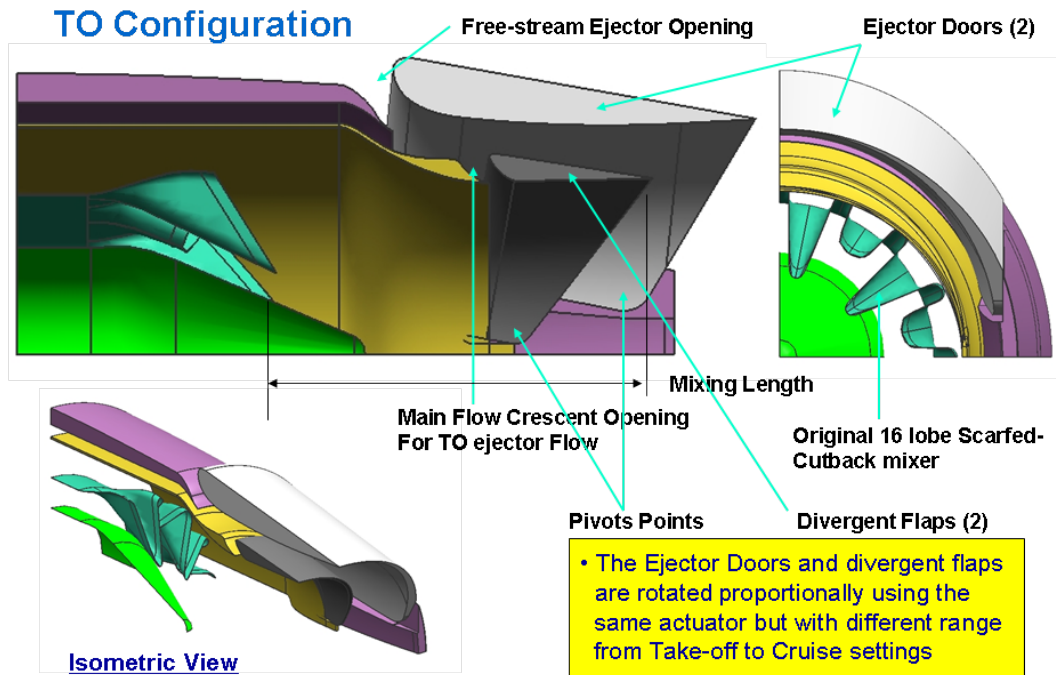
Mixer-ejector nozzle concept (patent pending)
