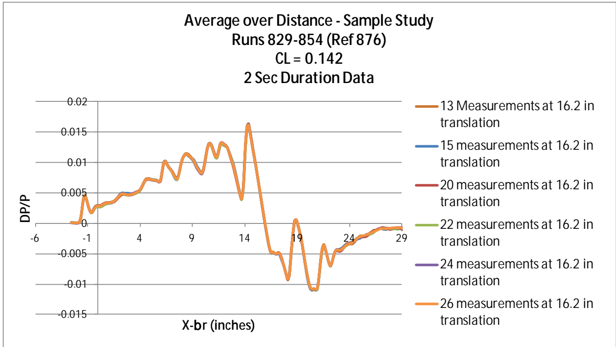
Figure 102. Initial approximation: reduce testing to 2 sec samples and 18 measurements
