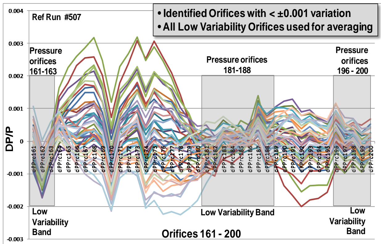
Figure 93. Excluded High Variability Orifices Averaged Technique
