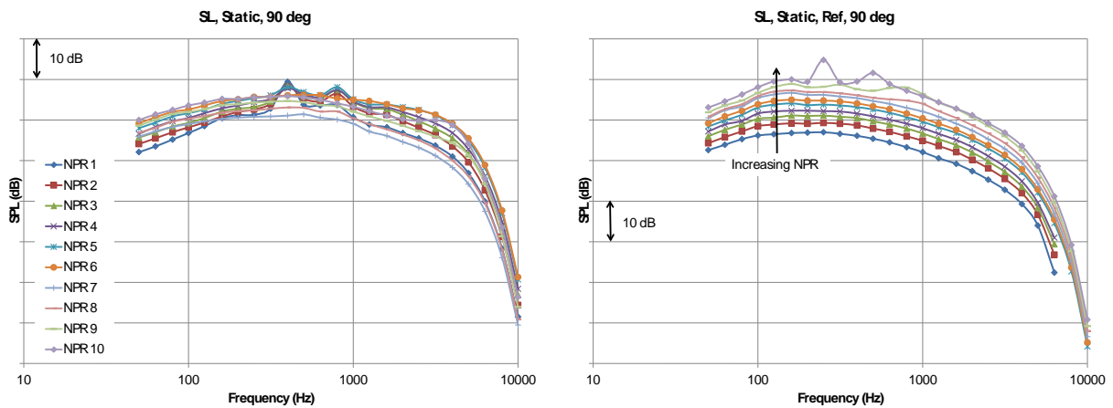
Figure 44 SPL at 90 deg for Sideline Configuration, Static Conditions, Processed to Sideline, No Heat Addition Cycle Conditions, Test Nozzle on Left, and Reference Nozzle on Right.
