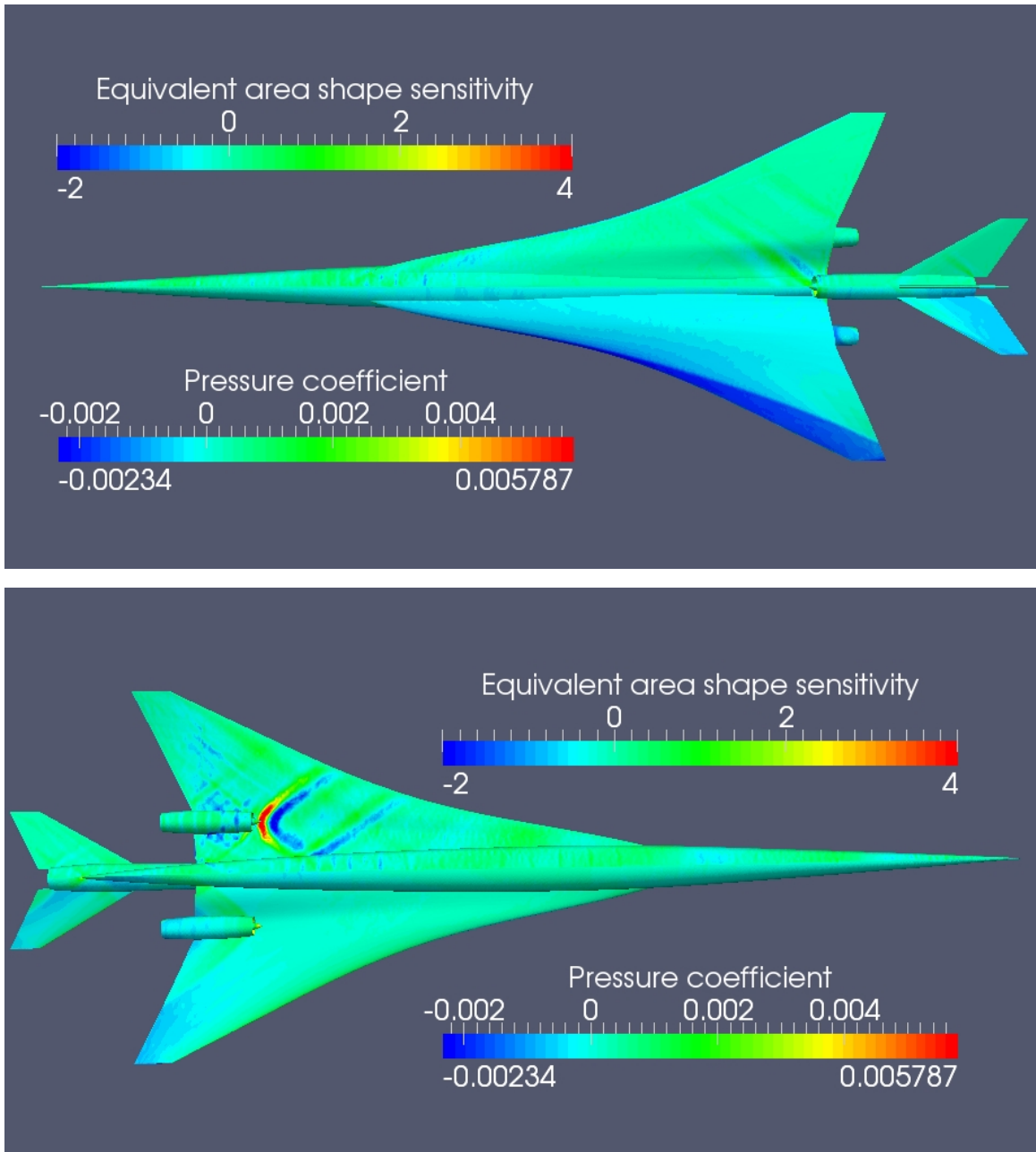
Figure 11. Upper and lower surface C_p and shape sensitivity distributions
