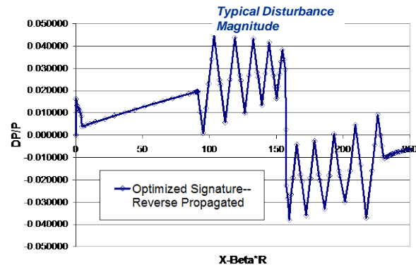
Figure 20. (2) Reverse Propagation
