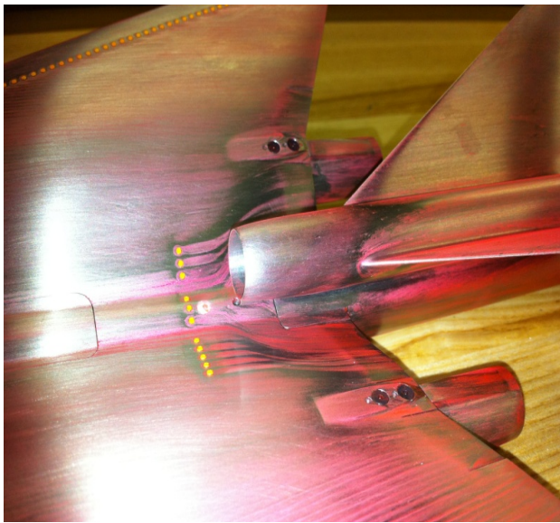
Figure 81. Flow around Center Nacelle Nicely Attached
