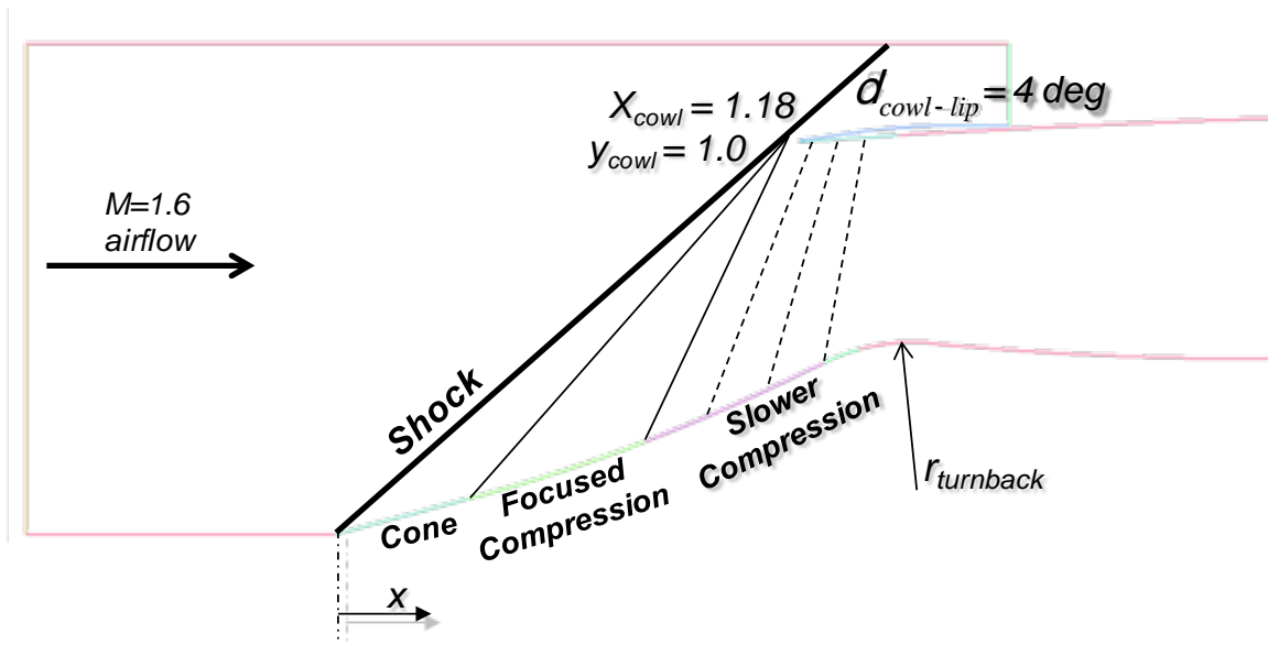
Figure 113. Sample 2-D CFD Domain and Geometry Features of the Inlet
