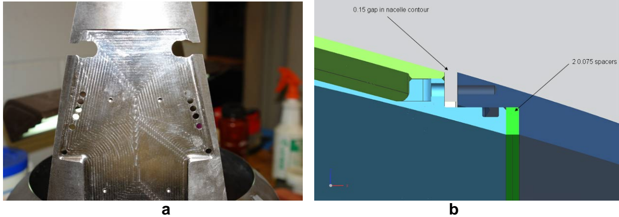
Figure 20 Model details: side wall (a) -undercover plate with Pin holes to set ejector doors; Secondary nozzle split joint (b) - 2-third stream Spacers used to vary throat area
