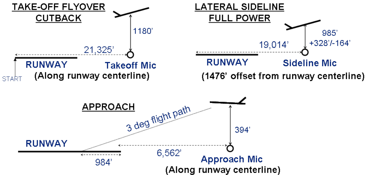
Figure 5 N+2 Trajectory Operating Conditions for Noise Predictions
