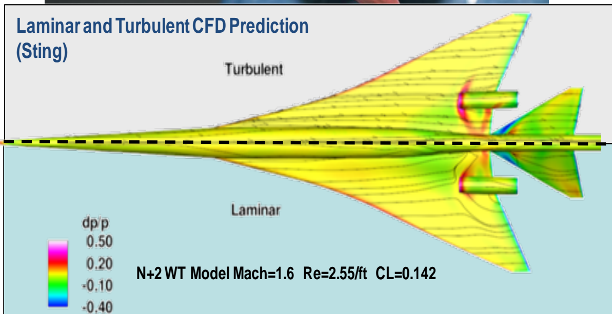
Figure 85. Oil flow showing fully attached like turbulent on lower surface
