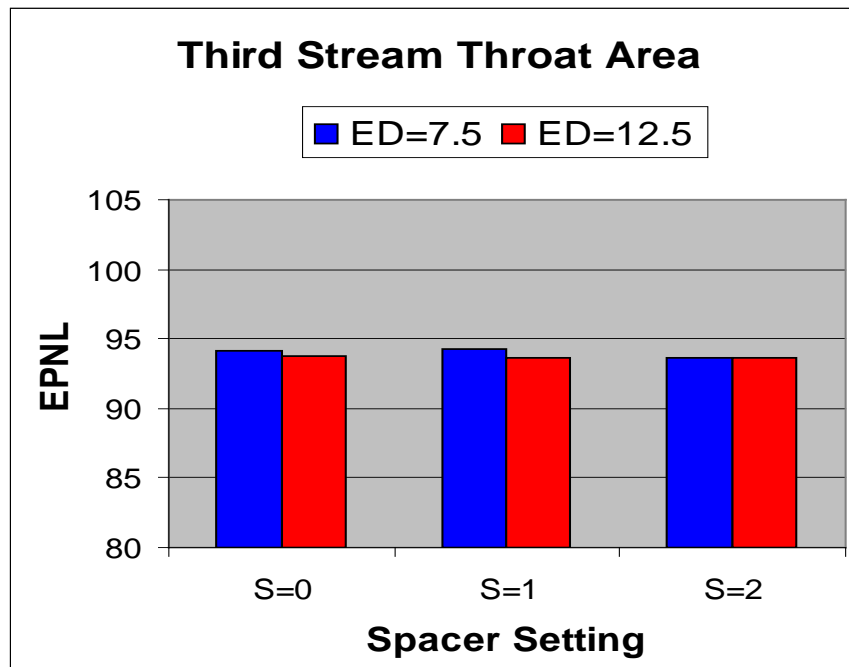
Figure 29 Effect of throat area change (spacers) on EPNL (set point 103), all results at DF=10
