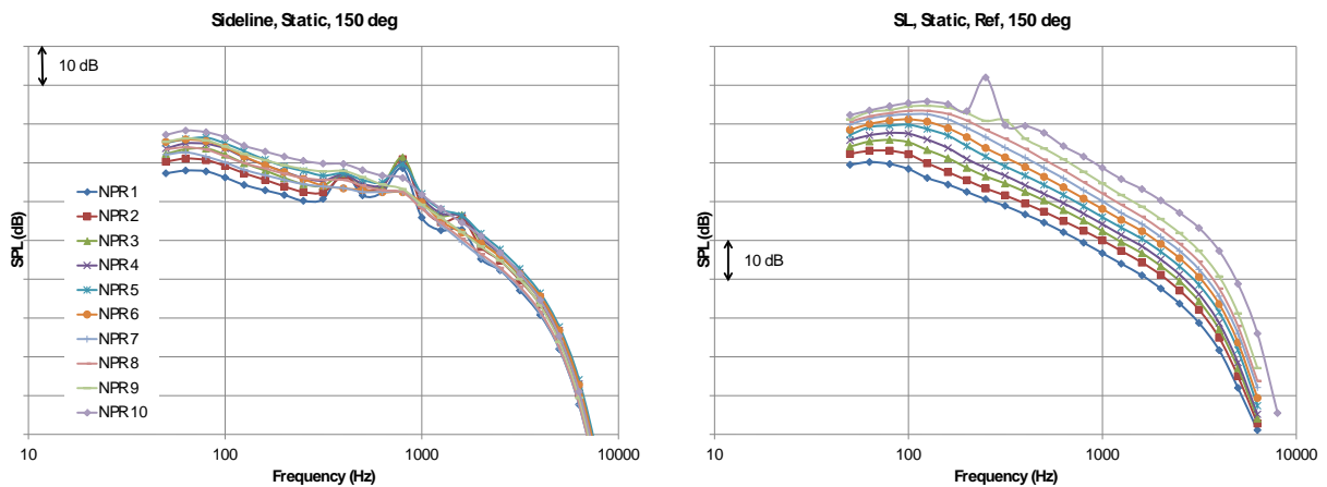
Figure 46 SPL at 150 deg for Sideline Configuration, Static Conditions, Processed to Sideline, No Heat Addition Cycle Conditions, Test Nozzle on Left, and Reference Nozzle on Right.
