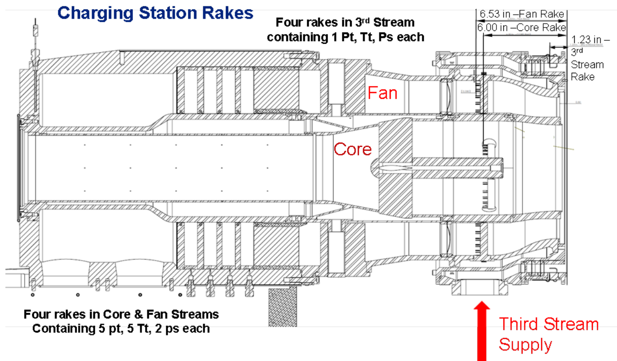
Figure 17 Modified HFJER Test Rig
