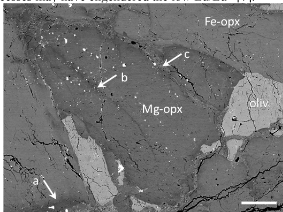
Figure 2. BSE images of magnesian veins the orthopyroxenite (a) and harzburgite (b) lithologies, and a possible melt vein (c). Scale bar is 0.1 mm.
