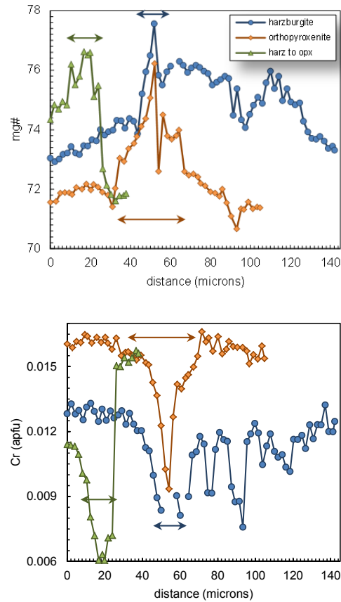
Figure 3. Traverses across Mg-veins in the orthopyroxenitic and harzburgitic lithologies, and across the contact between clasts of the two. Arrows indicate approximate locations of the veins in the traverses.
