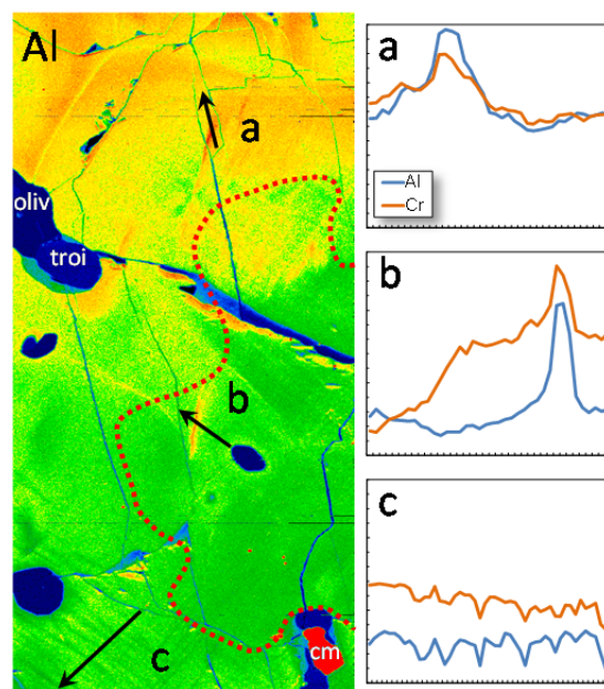
Fig. 1. Al x-ray map (blue-low; red-high), and Al and Cr traverses for MIL 07001,55. Green to brown – orthopyroxene; red - chromite (cm); blue - olivine (oliv) and troilite (troi). Red dotted line encloses core of lowest Ca pyroxene. Image is 1.0 × 0.5 mm. Vertical scales on all plots are the same.
