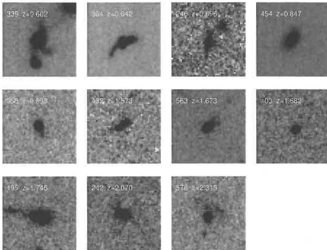
Fig. 3.— The GOODS-S i -band postage stamps of the 11 ERS galaxies in our sample. The irregular morphologies, interacting companions, and tidal features demonstrate ongoing star-formation of these galaxies.
