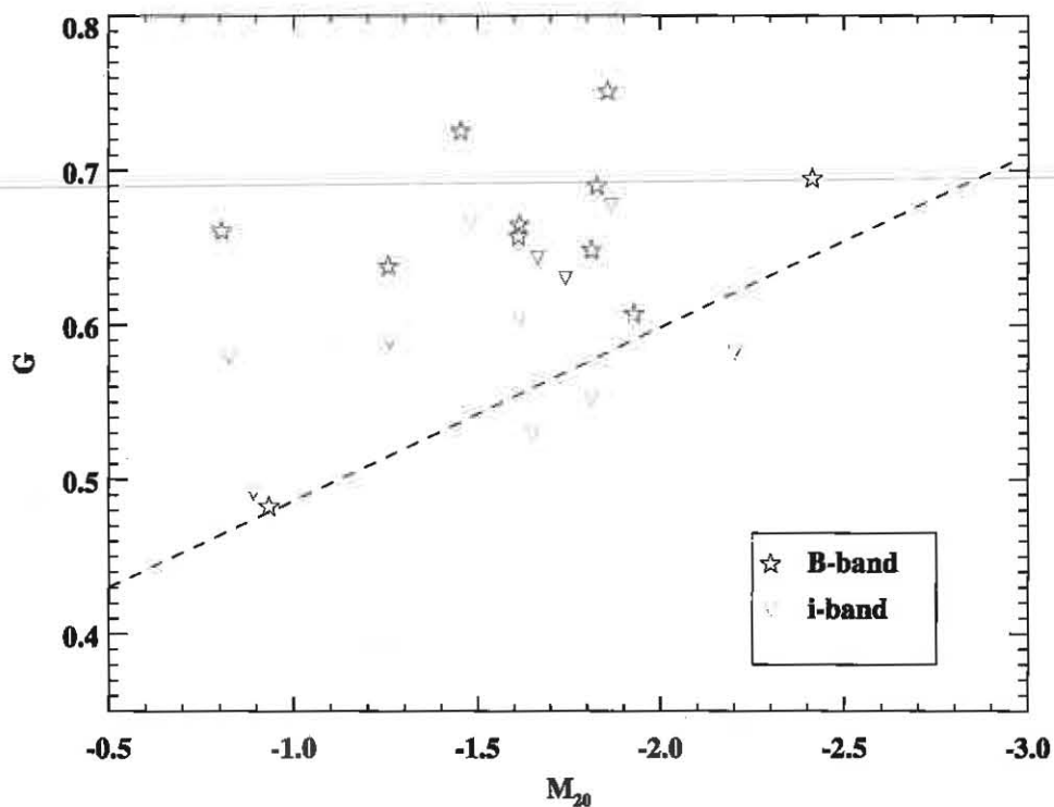
Fig. 4.— Gini coefficient G vs. M_{20} to demonstrate the morphology analysis of the 11 galaxies in our sample. The dashed line is the empirical line dividing interacting galaxies (upper region) with normal galaxies (lower region) from Lotz et al. (2004). The blue stars represent galaxies based on B -band image analysis. The red triangles are that based on i -band image analysis. Most galaxies lie above the line demonstrating disturbed morphologies.
