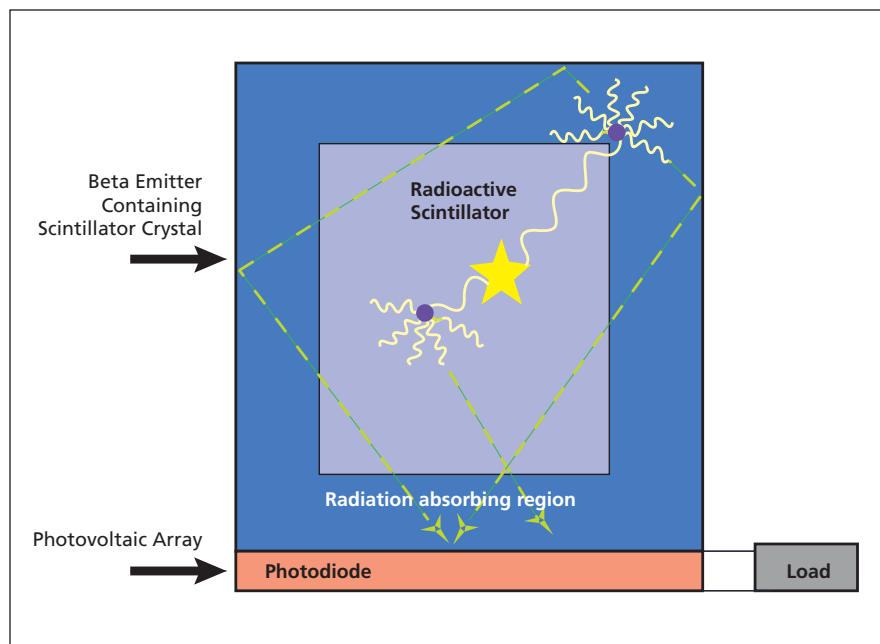
The Scintillator-Based Beta Battery : Isotope containing scintillator and surrounding scintillator captures virtually all of the energy emitted by the beta emitter.
