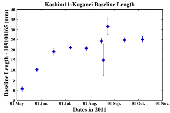
Figure 2. Post-seismic baseline length changes of Kashima11 – Koganei11 from sessions that were correlated at NICT and are listed in Table 2, as well as APSG29 and T2077 (which were correlated at GSI/Tsukuba and are omitted from Table 2). The APSG29 and T2077 points have the largest error bars.
