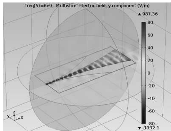
Ey field on the element at 6 GHz \epsilon_r = 10
