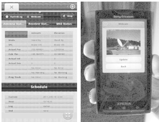
Figure 4. (left) A screen shot of the smartphone software with Antenna Control Unit and the current schedule. (right) Webcam of the radio telescope in the interface of the smartphone software for VLBI experiments.
