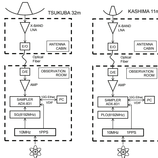
Figure 1. A system block diagram. RF direct sampling was operated at Kashima 11-m and Tsukuba 32-m.
