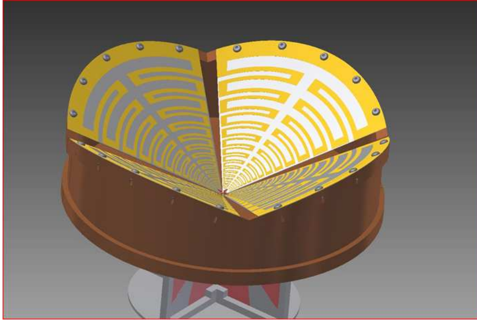
Figure 3. Drawing of the new circular Eleven feed.
