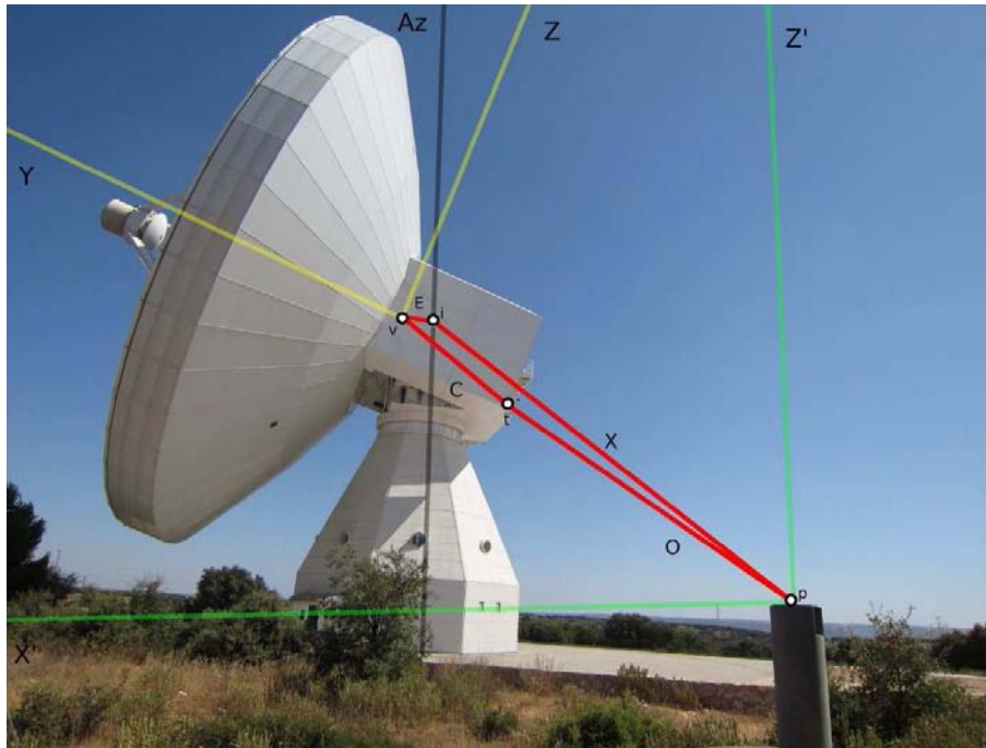
Figure 1. Geometric approach to determine the location of the Invariant Reference Point of the 40-m radio telescope at Yebes observatory.
