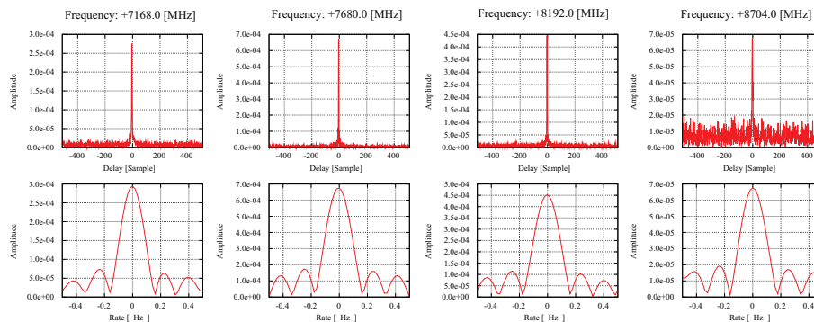
Figure 2. First fringes for DSAMS (Direct Sampling Applied for Mixed Signals) applied for X-band VLBI. The sampling mode of ADX-831 is 2bit-1024Msps. All four X-band fringes were simultaneously obtained with just one sampler.
