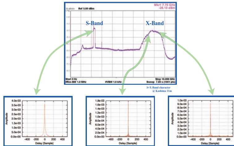
Figure 3. First fringe of DSAMS (Direct sampling applied for mixed signals) applied for geodetic VLBI. The sampling mode of ADX-831 is 2bit-1024Mps. Fringes of S-band and X-band were simultaneously obtained with only one sampler.
