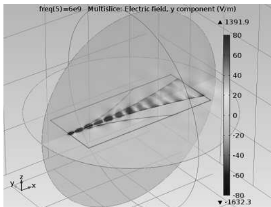
Ey field on the element at 6 GHz \epsilon_r = 2.2
