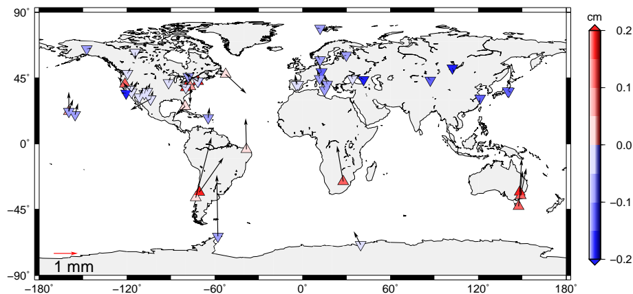
Figure 2. Influence of a priori gradients on station coordinates at epoch 2000.0. In both cases, tropospheric gradients were estimated as piecewise linear offsets every six hours with 1 mm absolute and 0.5 mm relative constraints. We show the differences in the sense DAO a priori gradients minus zero a priori gradients . Horizontal position changes are shown as arrows, vertical changes by color-coded triangles pointing in the direction of change (from Spicakova et al. (2012, [4])).
