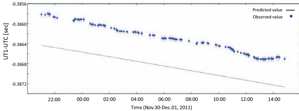
Figure 2. dUT1 values estimated from the “UREO01” session.
