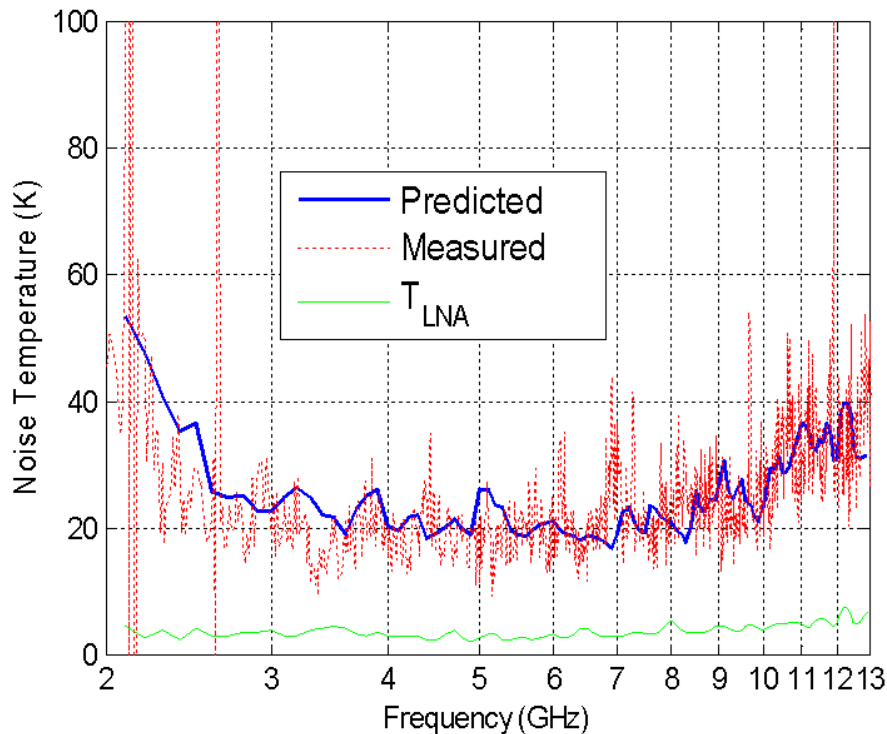
Figure 4. Measured (dashed line, red) and predicted system noise temperature (solid line, blue). The noise temperature of the LNAs is shown as thin solid line in green.
