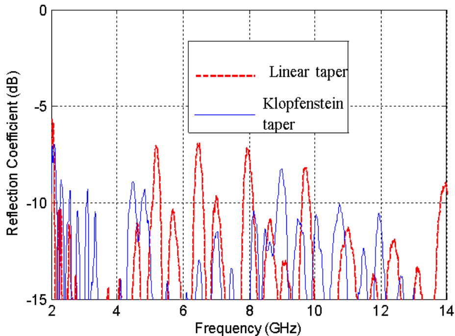
Figure 2. Measured reflection coefficient for the two balun-fed Eleven feed prototypes: linear taper (dashed line, red) and Klopfenstein taper (solid line, blue).
