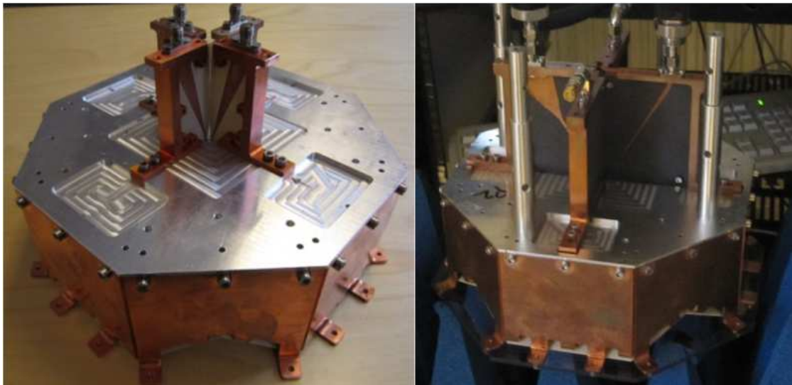
Figure 1. Balun-fed Eleven feeds with linear taper (left) and with Klopfenstein taper (right).
