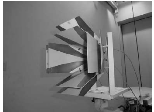
Figure 4. Experimental elements for wideband feeds.
