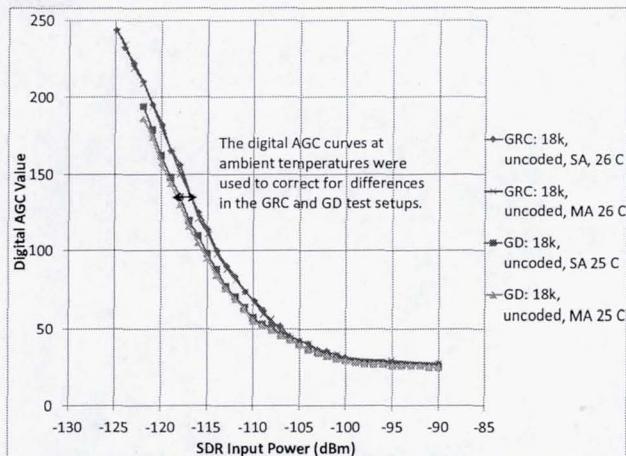
Figure 2: This graph illustrates the GD and GRC test setup alignment process. The GD data was -1.5 dB offset from the GRC data.
