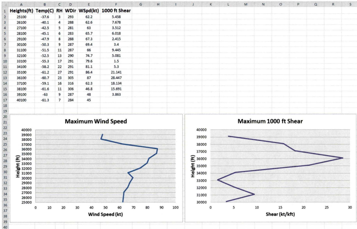
Figure 5. Example screen capture of the X100 worksheet tab in GUI.
