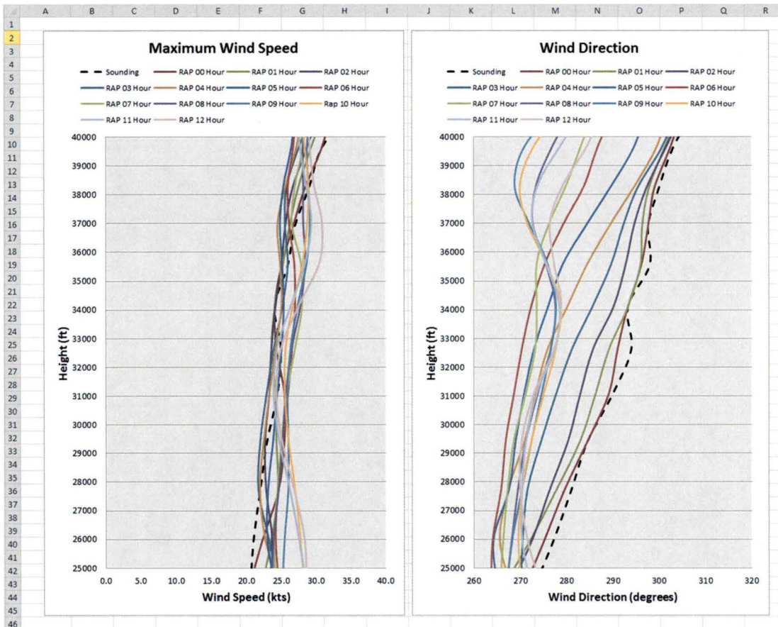
Figure 6. Screen capture of the RAP tab in GUI.
