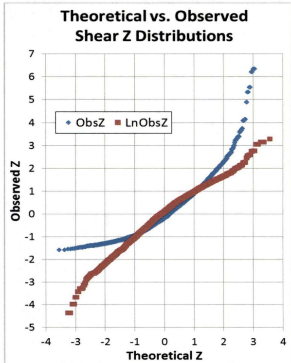
Figure 3. Same as Figure 2 but for wind shear.
