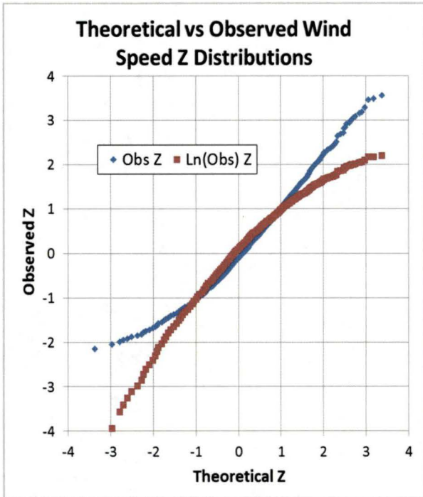
Figure 2. Curves showing the relationship of the z values for the observations (blue) and the ln of the observations (red) to the theoretical Gaussian z values.
