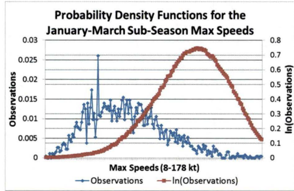
Figure 1. The PDFs of the maximum speed observations (blue, left axis and solid grid lines) and ln of the observations (red, right axis and dotted grid lines).
