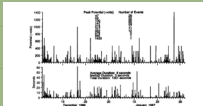
(a) DMSP Charging Frequency December 1986 – January 1987
