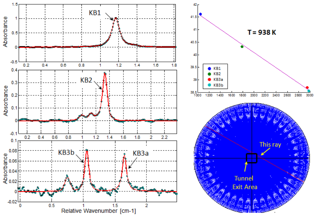
Figure 13. Fitted spectra, calculated temperature, and location of a cold ray.
