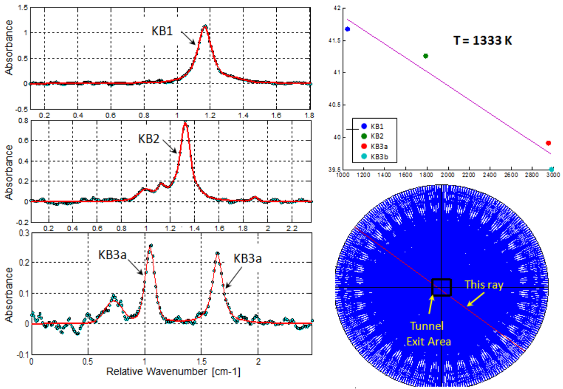
Figure 14. Fitted spectra, calculated temperature, and location of a hot ray.
