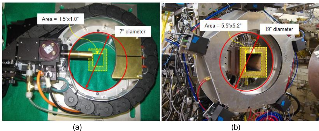
Figure 6. (a) TDLAT system used for measurements on UVaSCF and (b) TDLAT system for measurements on DCSCF.
