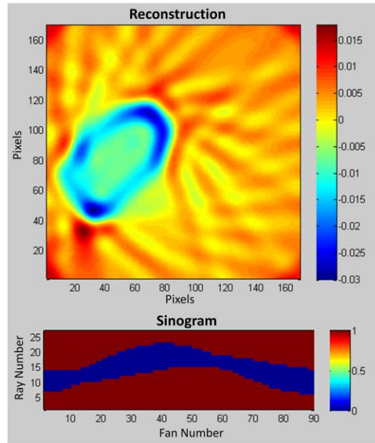
Figure 11. Sinogram and Tomographic Reconstruction of opaque object.
