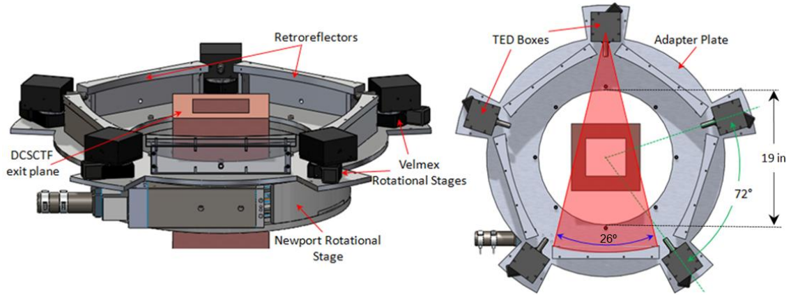
Figure 7. SolidWorks model of the TDLAT system.
