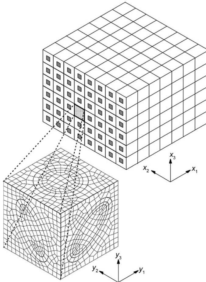
Figure 1.—Schematic illustration of a triply periodic array in the global ( x_1, x_2, x_3 ) space of multiphase composite media with its repeating unit-cell (RUC) having hexahedral subcells, defined with respect to its ( y_1, y_2, y_3 ) local coordinate system.
