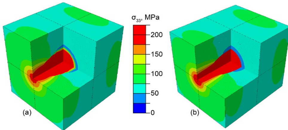
Figure 8.—Stress distributions in the RUC with a spheroidal inclusion. (a) HFGMC results, (b) FE results.
