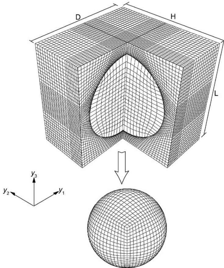
Figure 5.—Parametric HFGMC 3-D meshes for an RUC with spherical inclusion using hexahedral subcells.
