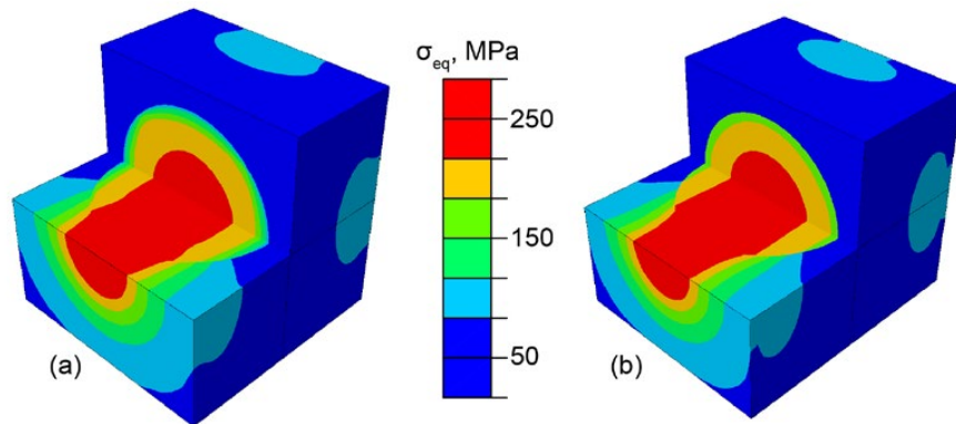
Figure 6.—Stress distributions in the RUC with a spherical inclusion. (a) HFGMC results, (b) FE results.
