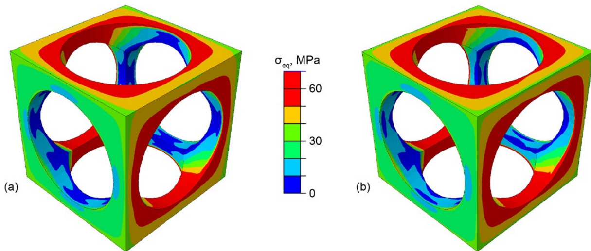
Figure 12.—Stress distributions in the RUC of the foam material. (a) HFGMC results (periodic displacements), (b) FE results (periodic displacements).
