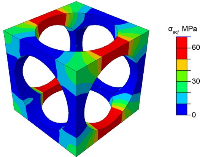
Figure 13.—Stress distributions in the RUC of the foam material showing HFGMC results with full periodic conditions (displacements and tractions).
