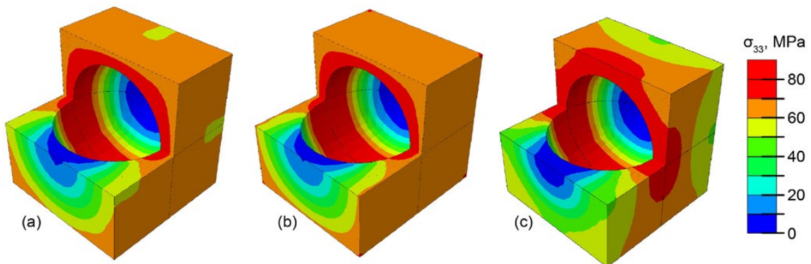
Figure 4.—Stress distributions in the RUC with a spherical cavity. (a) HFGMC results (periodic displacements), (b) FE results (periodic displacements), and (c) HFGMC results (periodic displacements and tractions).
