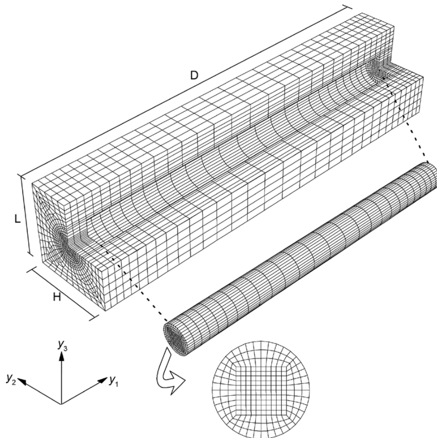
Figure 9.—Parametric HFGMC 3-D meshes for an RUC, with discontinuous aligned fiber having a circular cross-section, using hexahedral subcells.
