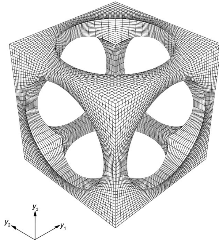
Figure 11.—Parametric HFGMC mesh for an RUC of a foam material.
