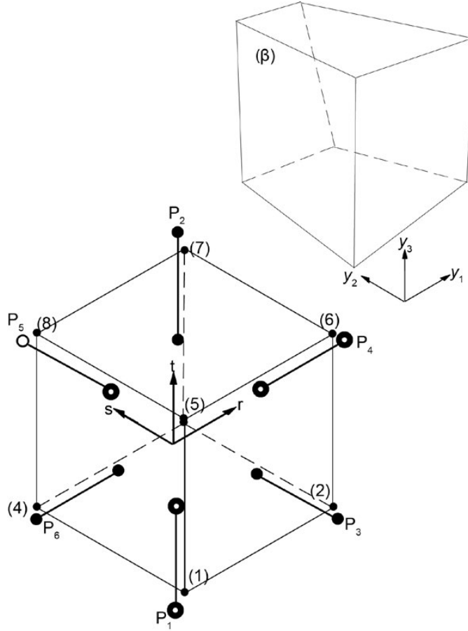
Figure 2.—A hexahedral shaped subcell in its physical and natural coordinates. Numbering for the faces and corners are shown.
