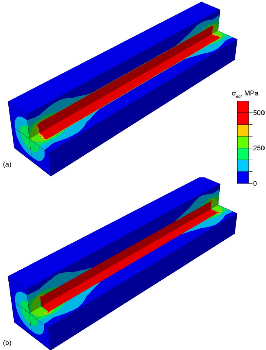
Figure 10.—Stress distributions in the RUC with the discontinuous fiber. (a) HFGMC results, (b) FE results.
