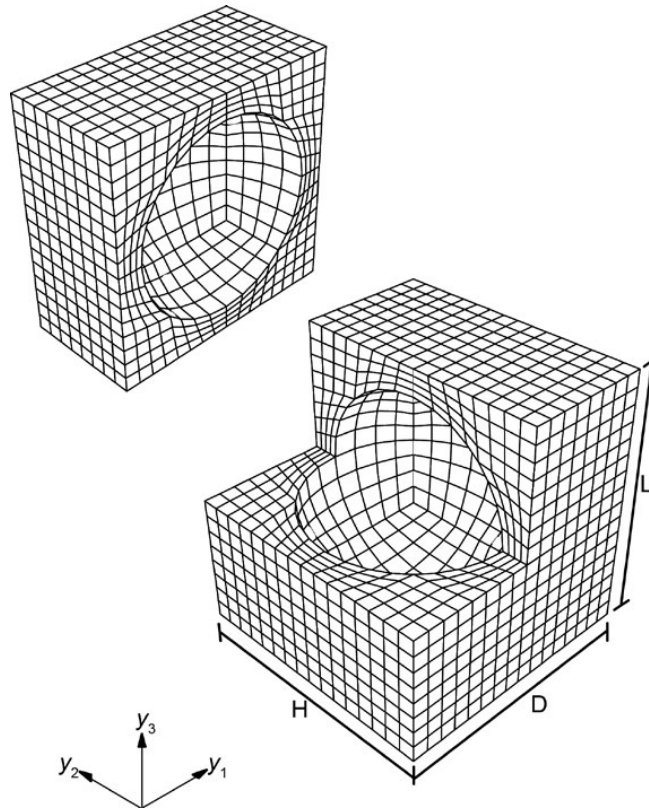
Figure 3.—Parametric HFGMC meshes for an RUC with spherical cavity.
