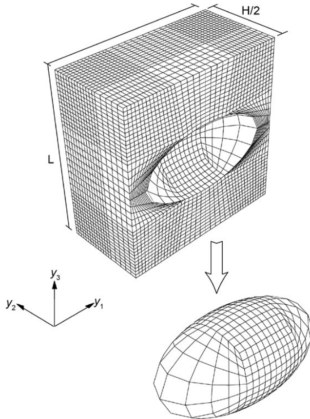
Figure 7.—Parametric HFGMC 3-D meshes for an RUC with spheroidal inclusion using hexahedral subcells.
