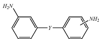
2-RING DIAMINE
