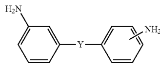
2-RING DIAMINE
