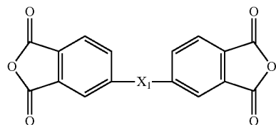
SYMMETRIC DIANHYDRIDE
