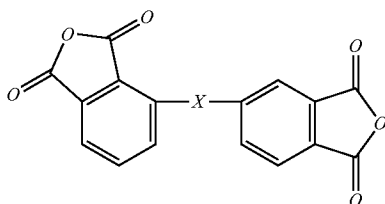
ASYMMETRIC DIANHYDRIDE
