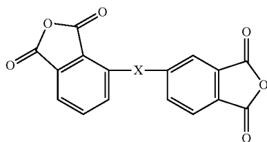
ASYMMETRIC DIANHYDRIDE
