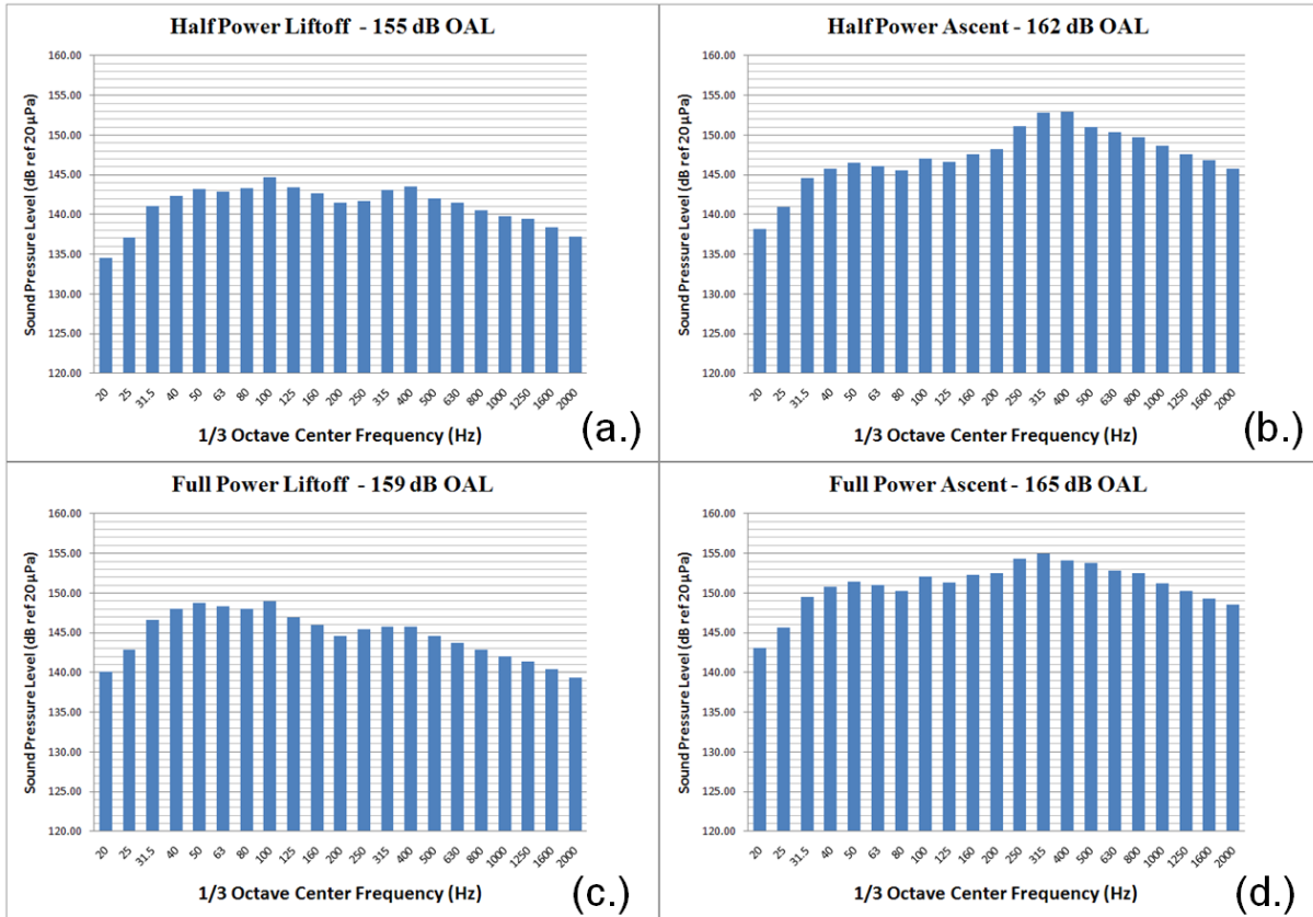
Figure 5. Average Measured Sound Pressure Level. (a.) Half Power Lutoff. (b.) Half Power Ascent (c.) Full Power Lutoff. (d.) Full Power Ascent .
