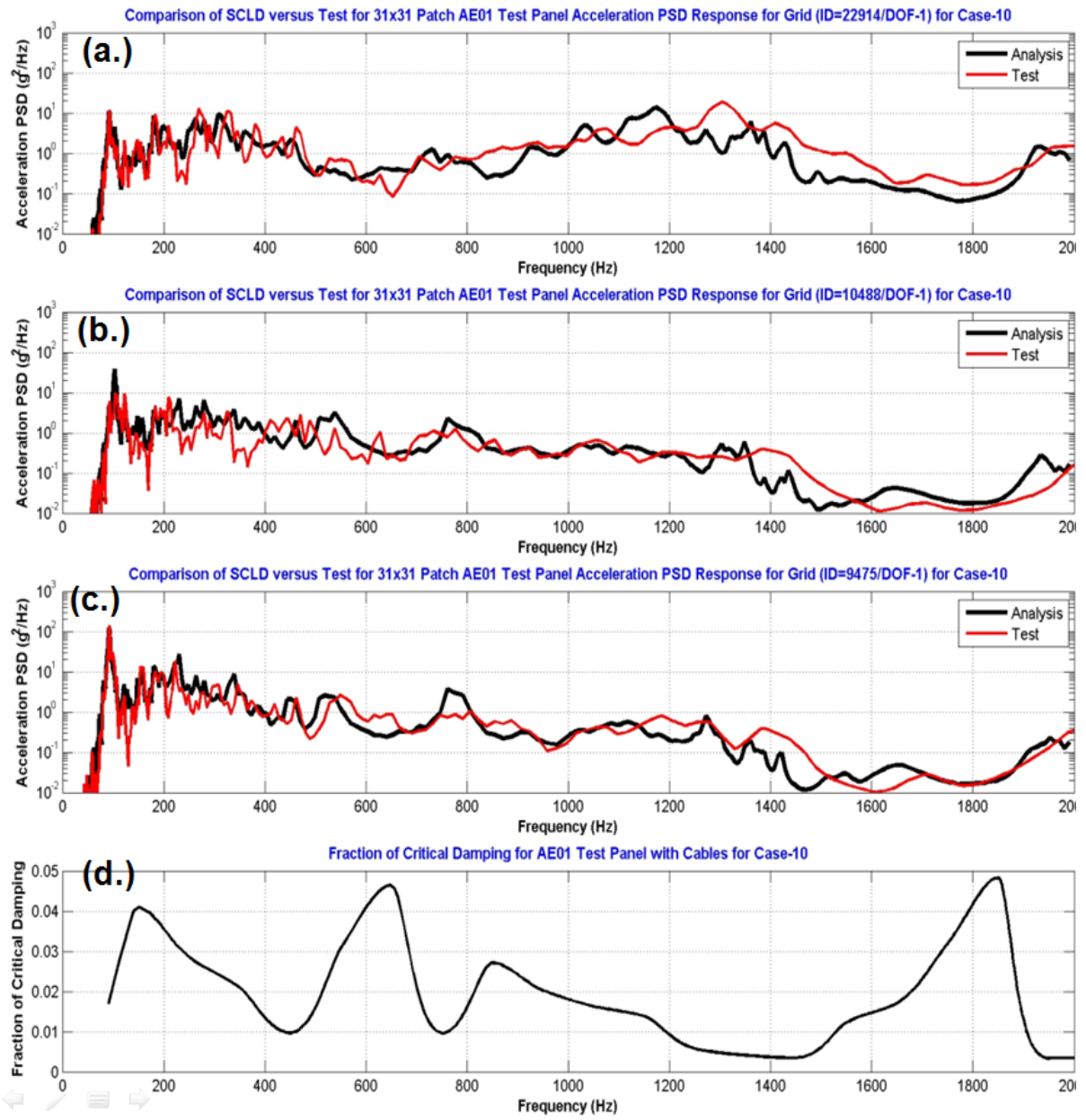
Figure 14. Example Comparison Response at Locations not used in the Optimization Set vs. Measured Response for Light Cable Set (Case 10) Full Power Liftoff. (a.) Accelerometer 2z - 22914. (b.) Accelerometer 16z - 10488. (c.) Accelerometer 30z - 9475. (d.) System Damping Estimate.
