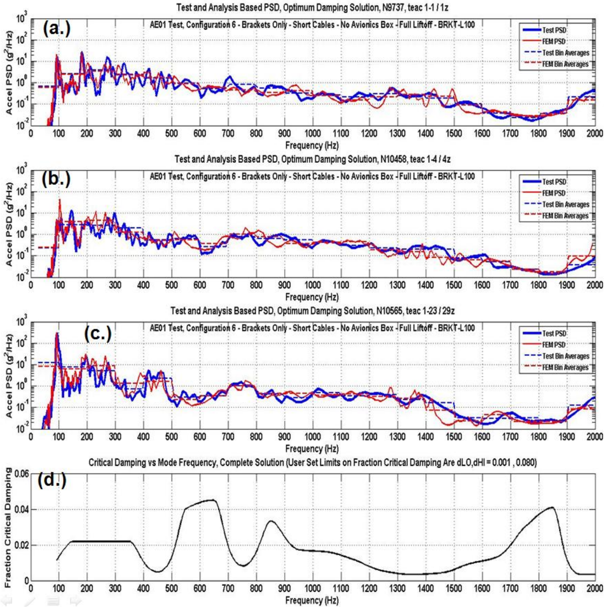
Figure 17. Response at Locations in the Optimization Set vs. Measured Response for “Brackets Only” (Case 6) Full Power Liftoff. (a.) Accelerometer 1z - 9737. (b.) Accelerometer 4z - 10458. (c.) Accelerometer 29z - 10565. (d.) System Damping Estimate.
