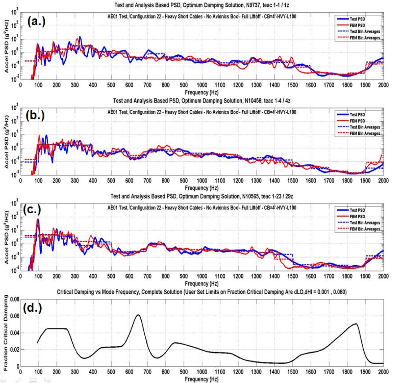
Figure 20. Response at Locations in the Optimization Set vs. Measured Response for Heavy Cable Set (Case 22) Full Power Liftoff. (a.) Accelerometer 1z - 9737. (b.) Accelerometer 4z - 10458. (c.) Accelerometer 29z - 10565. (d.) System Damping Estimate.
