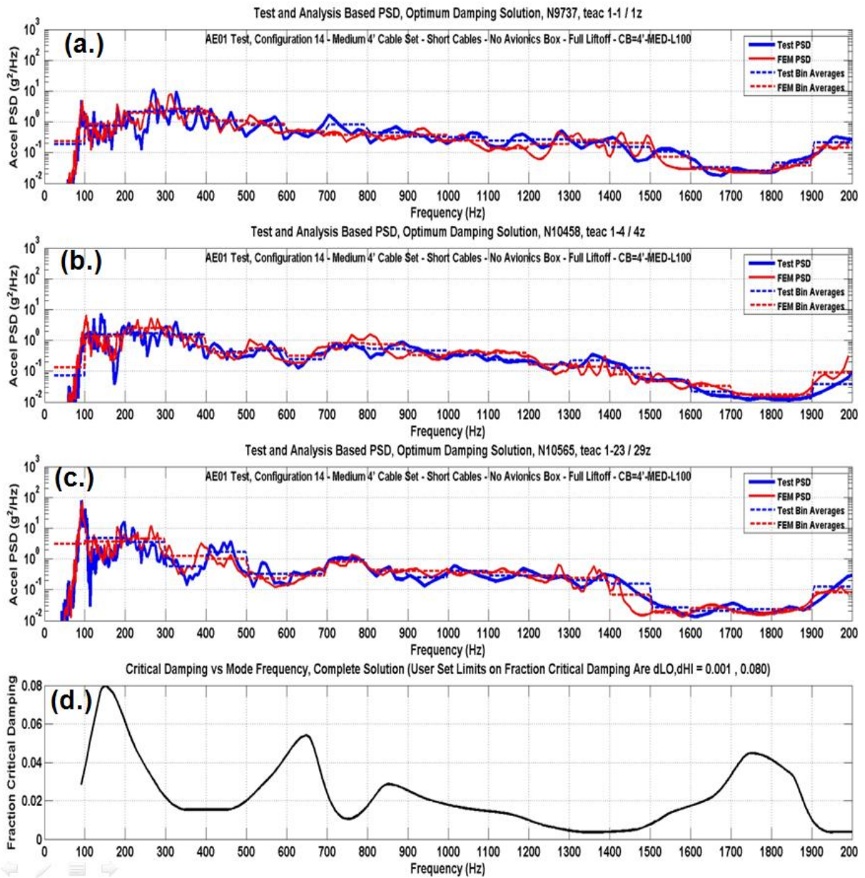
Figure 19. Response at Locations in the Optimization Set vs. Measured Response for Medium Cable Set (Case 14) Full Power Liftoff. (a.) Accelerometer 1z - 9737. (b.) Accelerometer 4z - 10458. (c.) Accelerometer 29z - 10565. (d.) System Damping Estimate.
