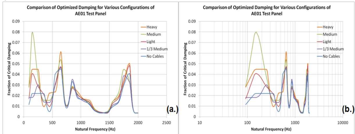
Figure 15. Estimated System Damping Schedule for Various Cable Set Configurations. (a.) Linear Frequency Scale Liftoff. (b.) Logarithmic Frequency Scale Liftoff.
