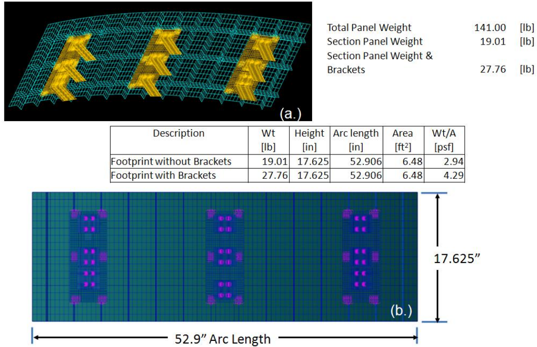
Figure 3. Foot print of local panel structure. (a.) FEM view of rib stiffened panel with adapter/brackets configured to support cables. (b.) FEM VIEW OF RIB stiffened panel with dimensions. The weight and weight per unit area are also summarized in the figure.
