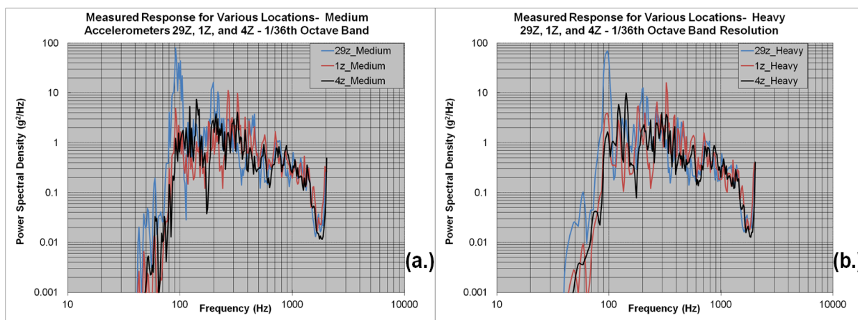
Figure 9. Measured Response at Various Measurement Locations from Consistent Cable Set Configurations. (a.) Medium Liftoff. (b.) Heavy Liftoff.
