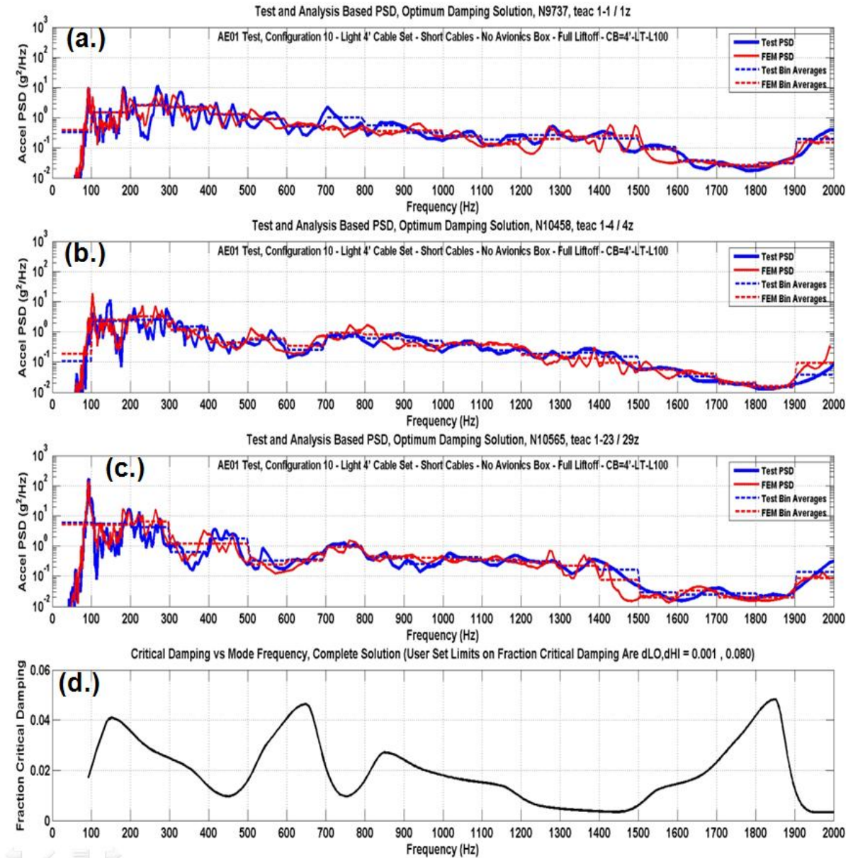
Figure 13. Example Comparison Response at Locations in the Optimization Set vs. Measured Response for Light Cable Set (Case10) Full Power Liftoff. (a.) Accelerometer 1z - 9737. (b.) Accelerometer 4z - 10458. (c.) Accelerometer 29z - 10565. (d.) System Damping Estimate.
