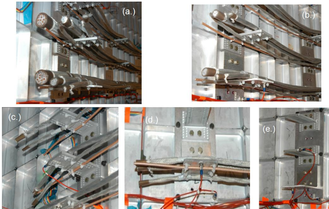
Figure 4. Photo depiction of each configuration (a) Heavy (b) Medium (c.) Light (d) 1/3 of Medium (e.) Brackets without cables
