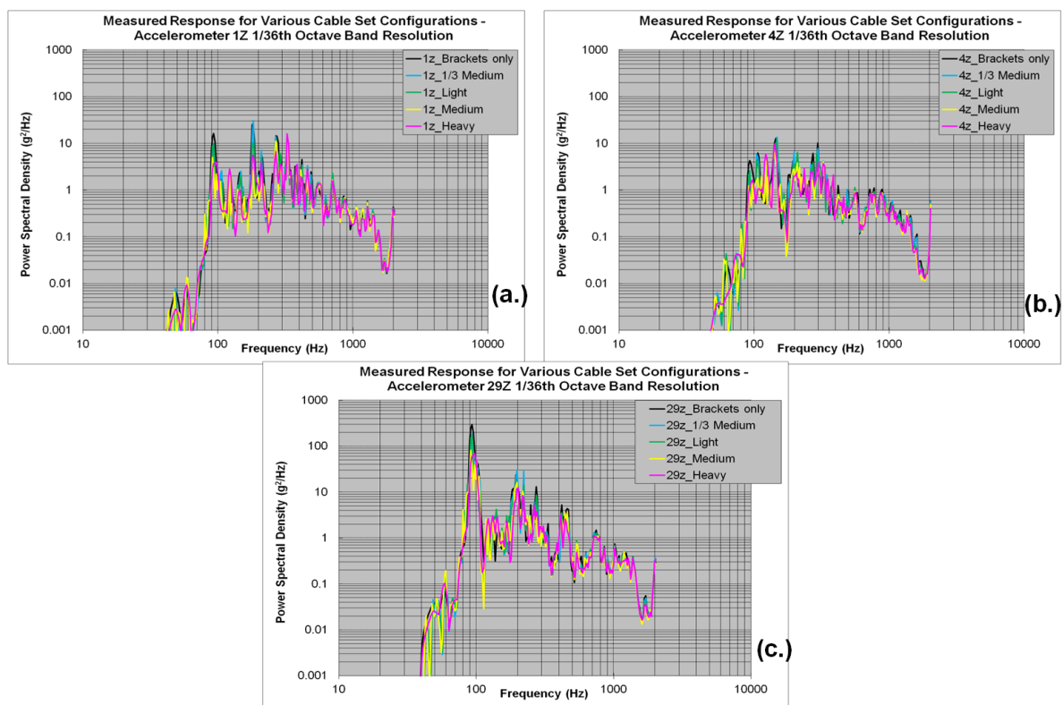
Figure 8. Measured Response for Various Cable Set Configurations - 1/36th Octave Band Full Power Liftoff. (a.) Accelerometer 1z. (b.) Accelerometer 4z. (c.) Accelerometer 29z.
