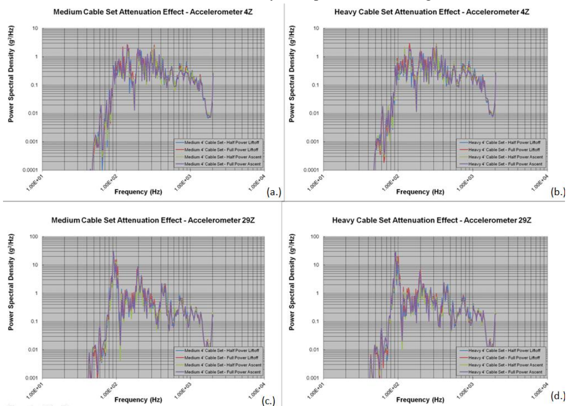
Figure 10. Overlay of Normalized Response Measurements provided as Linearity Check. Consistent Cable configurations assessed for different excitation levels.. (a.) Accelerometer 4z Medium Configuration. (b.) Accelerometer 4z Heavy Configuration. (c.) Accelerometer 29z Medium Configuration. (d.) Accelerometer 29z Heavy Configuration.
