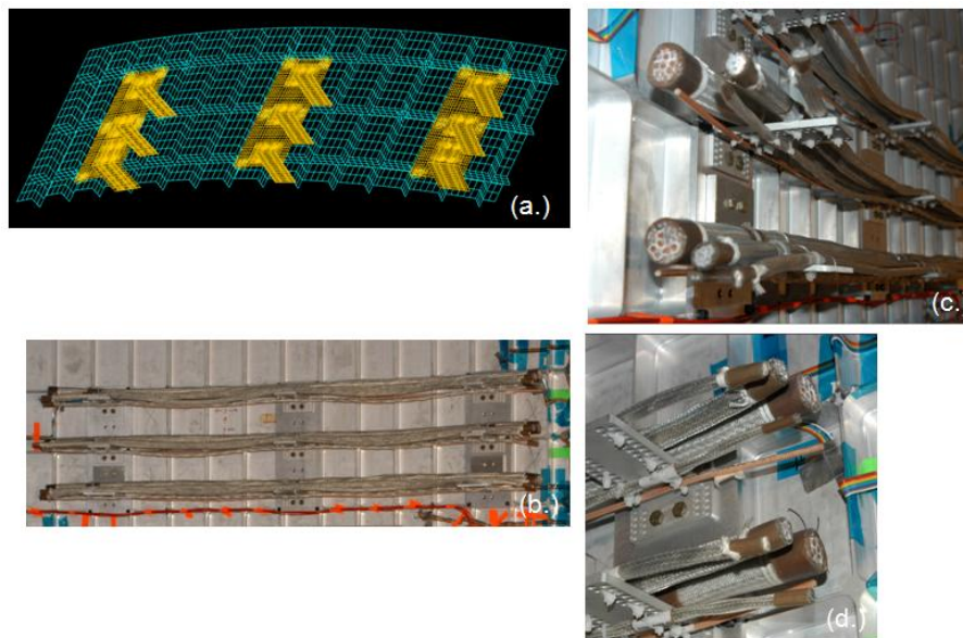
Figure 2. Local structure provided for integration of cable harnesses. (a.) FEM view of rib stiffened panel with adapter/brackets configured to support cables. (b.) Photo of same local structures configured with heavy cable set. (c.) close-up of heavy cable set from left end (d.) View of flight like test article from anechoic receiver room.
