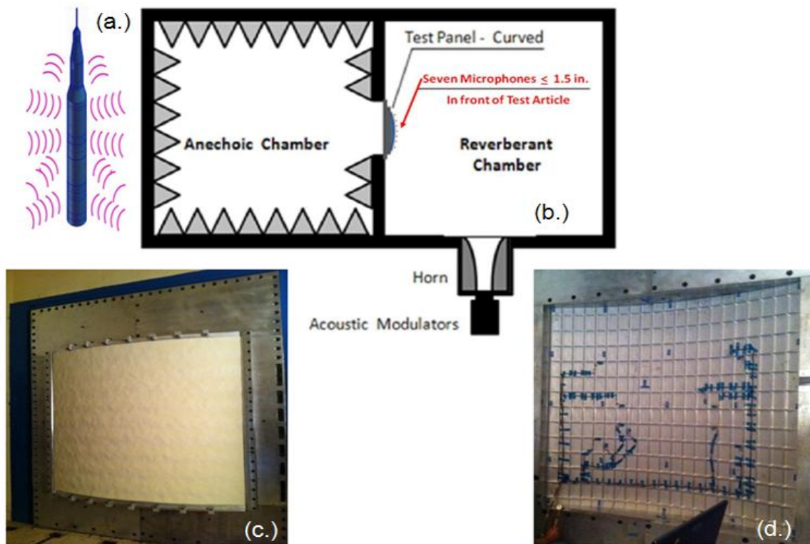
Figure 1. Relating test chamber setup and vehicle panel test article to excitation of a flight vehicle panel. (a.) Acoustic or fluctuating pressures affect the exterior surface of vehicle panels. (b.) Ground test setup. (c.) Flight like excitation of exterior surface in baffled panel test setup. (Reverberant) (d.) View of flight like test article from anechoic receiver room.
