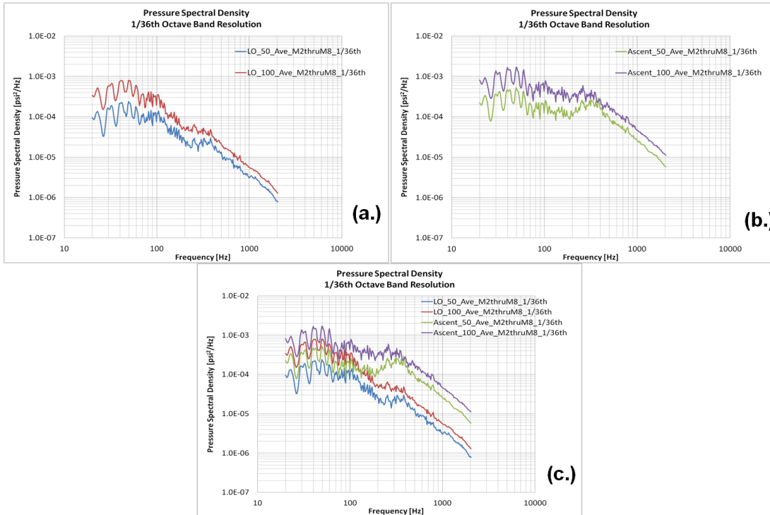
Figure 6. Average Measured Pressure Spectral Density presented as 1/36 th Octave Band Averaged Spectra. (a.) Overlay of Full Power Liftoff with Half Power Liftoff. (b.) Overlay of Full Power Ascent with Half Power Ascent. (c.) Overlay of all four Test Levels.
