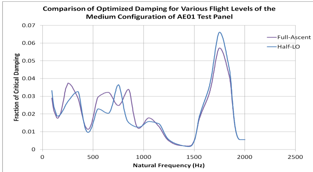
Figure 16. Range of Damping Schedule Differences produced by Exciting the same Cable Configuration at Different Levels Medium Cable Configuration
